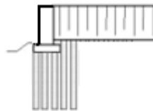
Figure 5. Illustration. Retaining wall supported on DMM without retained soil supported on DMM.
