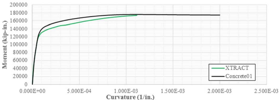
Figure 4.3 Moment-curvature results for XTRACT and OpenSees for the original conventional concrete design.
