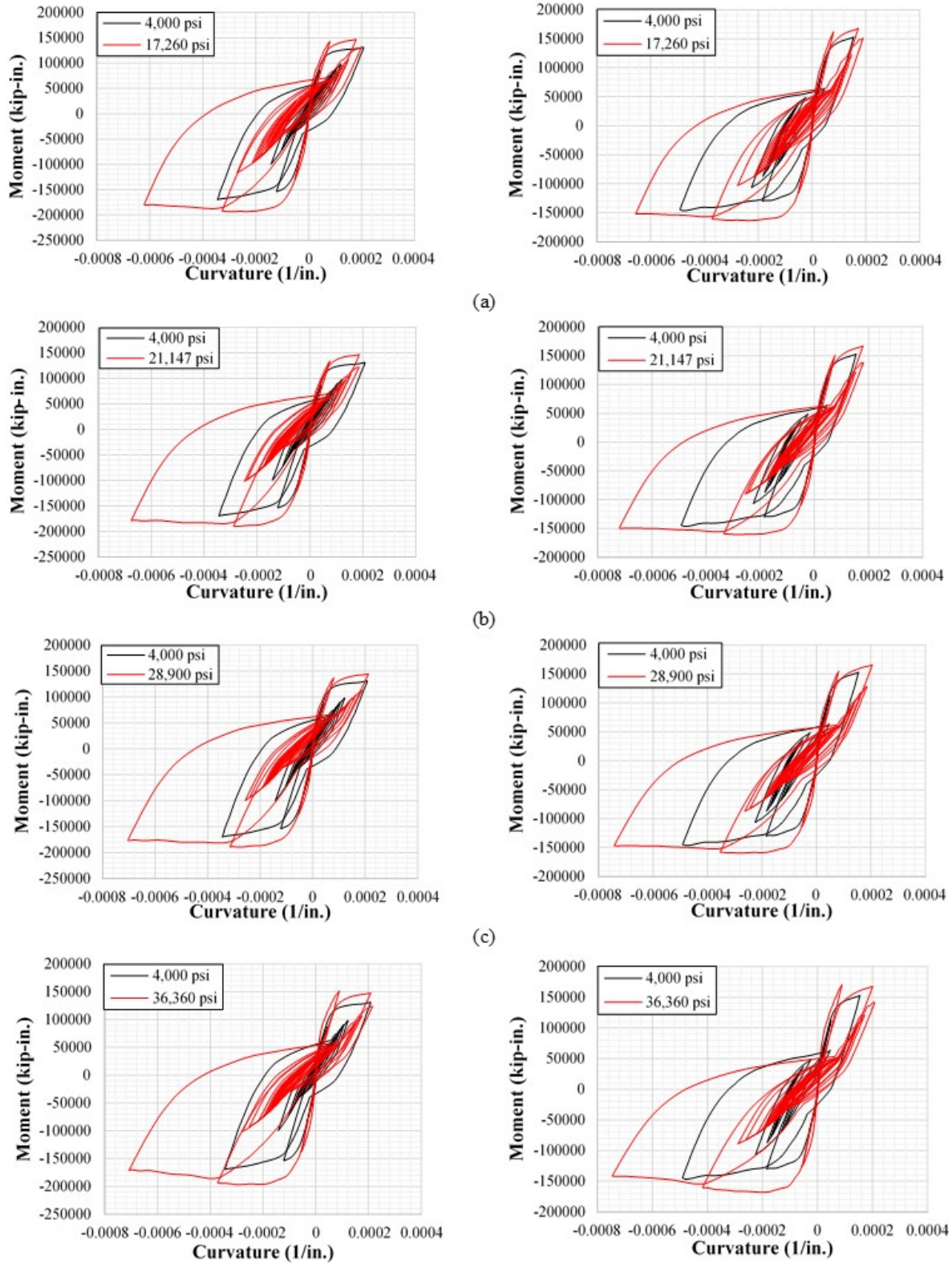
Figure 5.14 Moment-curvature response of the two pier columns for RSN 6 (Design Level) using (a) UHPC 1, (b) UHPC 2, (c) UHPC 3, and (d) UHPC 4.
