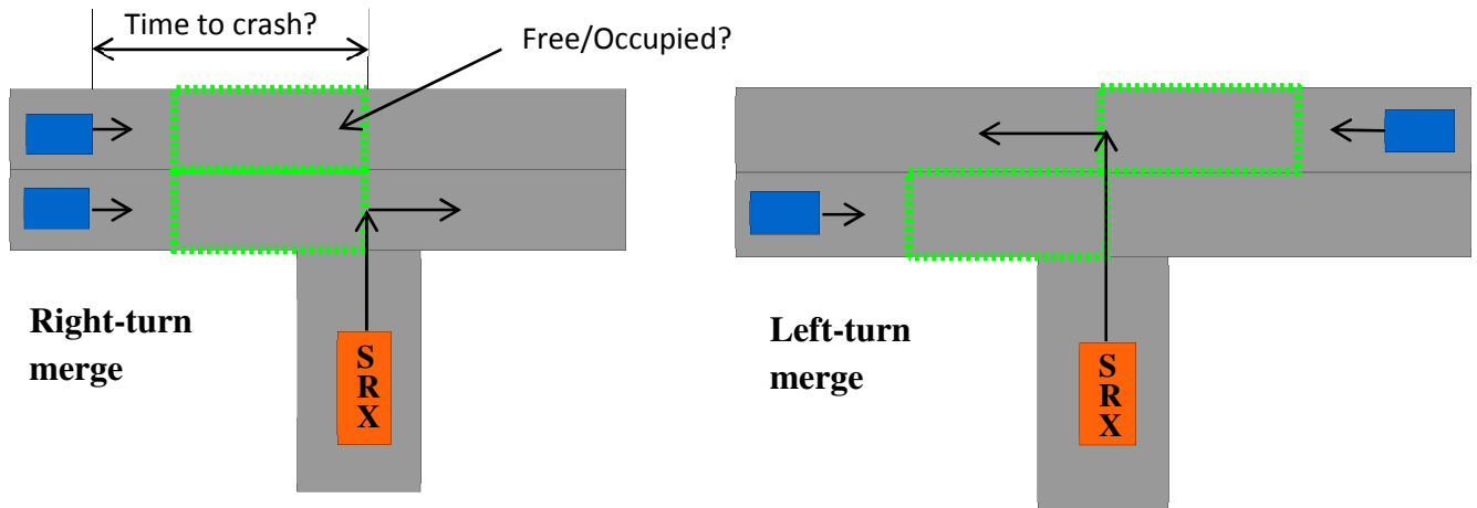
Figure 3. This figure depicts right- and left-turn merging onto a potentially high-speed road from a stop. Left: In the right-turn merge case, even though the intent is to turn into the bottom-most lane, we check both lanes in case the SRX swings out a bit into the upper lane. Right: In the left-turn merge case, we need both to clear the traffic coming from the left and enter the upper lane comfortably in front of traffic coming from the right.
