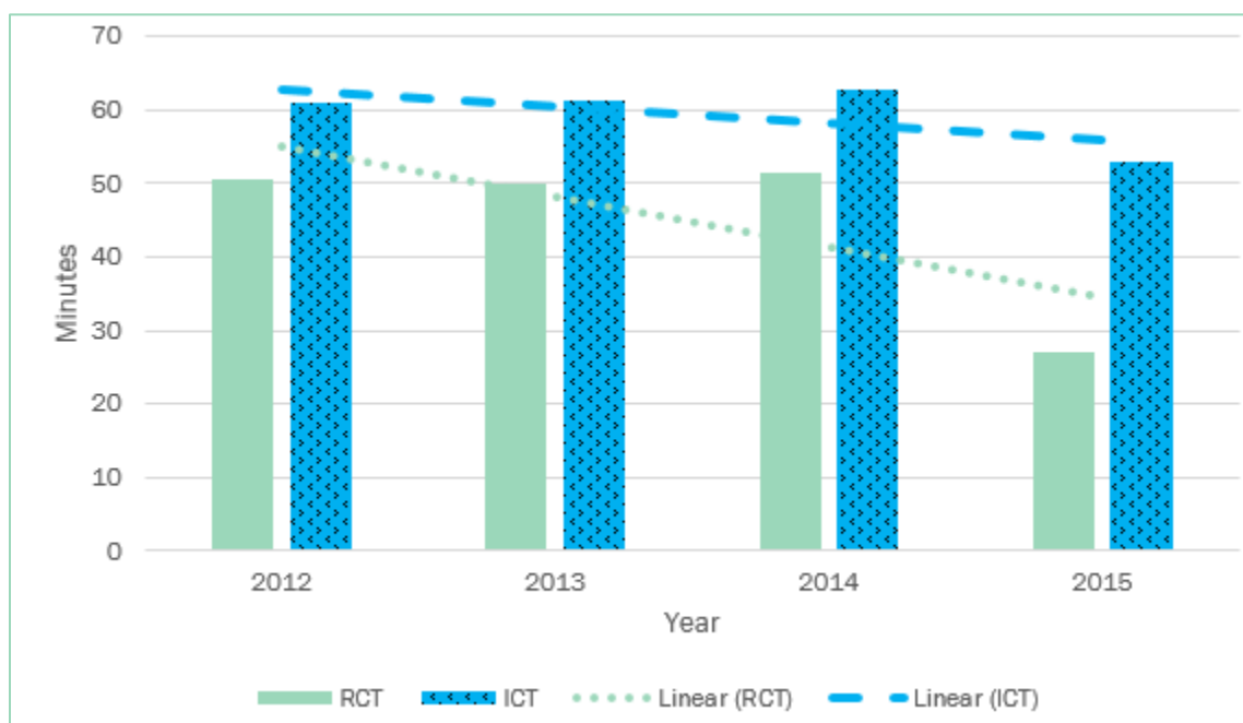
Figure 13. Bar chart. RCTs and ICTs for all crash types: Metropolitan Phoenix.
