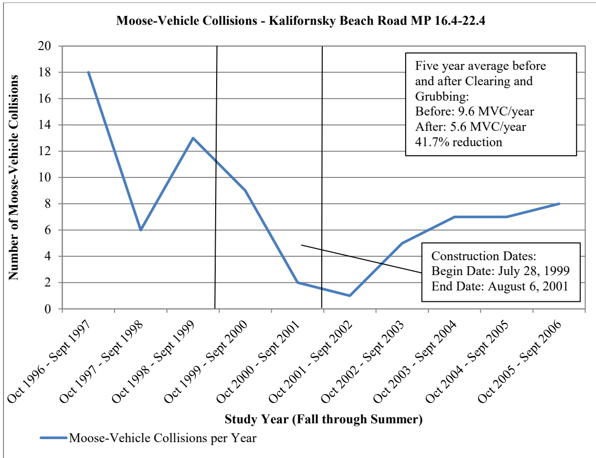
Figure C2 – Moose-Vehicle Collisions - Kalifornsky Beach Road MP 16.4-22.4
