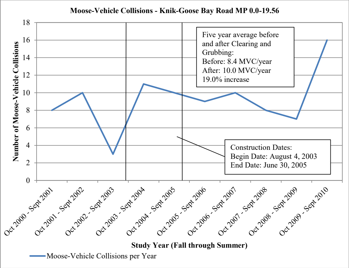
Figure C10 – Moose-Vehicle Collisions - Knik-Goose Bay Road MP 0.0-19.56
