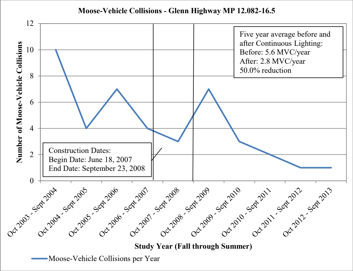
Figure C6 – Moose-Vehicle Collisions - Glenn Highway MP 12.082-16.5
