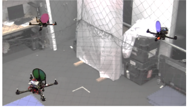
Fig. 1: A photograph of the formation of three quadrotors from our experimental setup.
