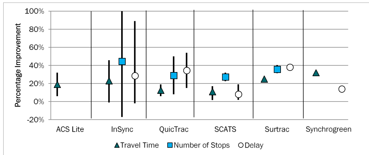
Figure 15. Graph. Effectiveness of ASCTs in phase 3.
