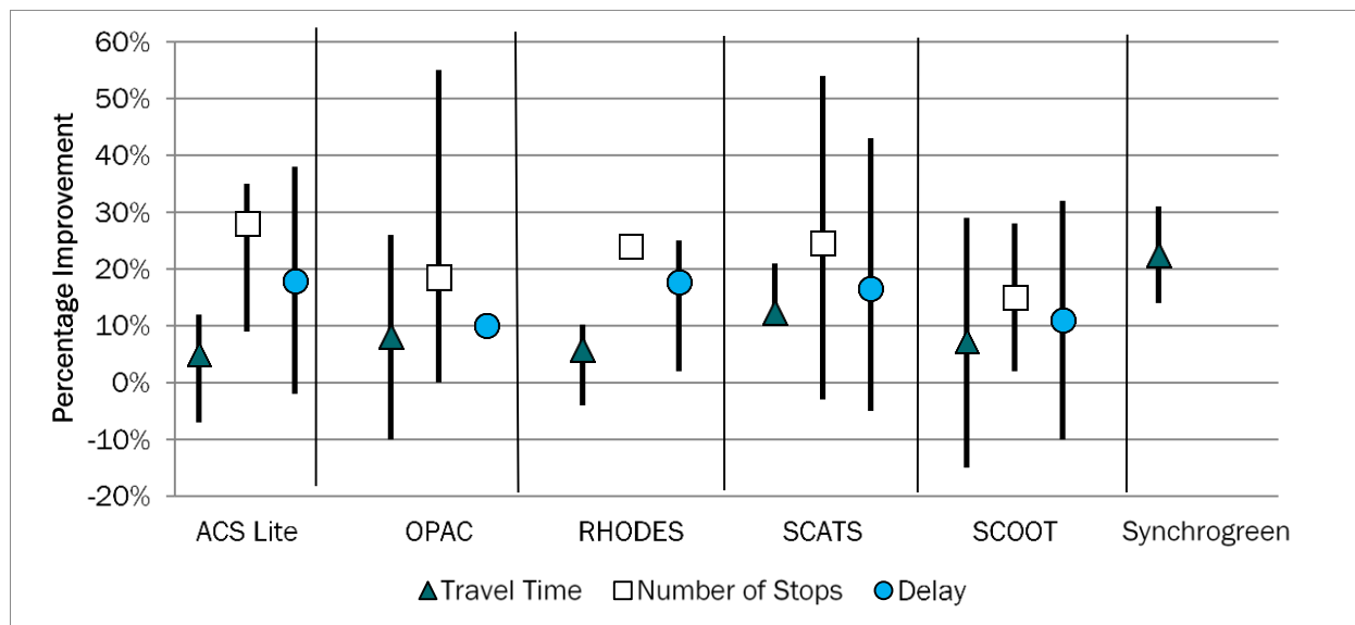
Figure 7. Graph. Effectiveness of ASCTs in phase 2.
