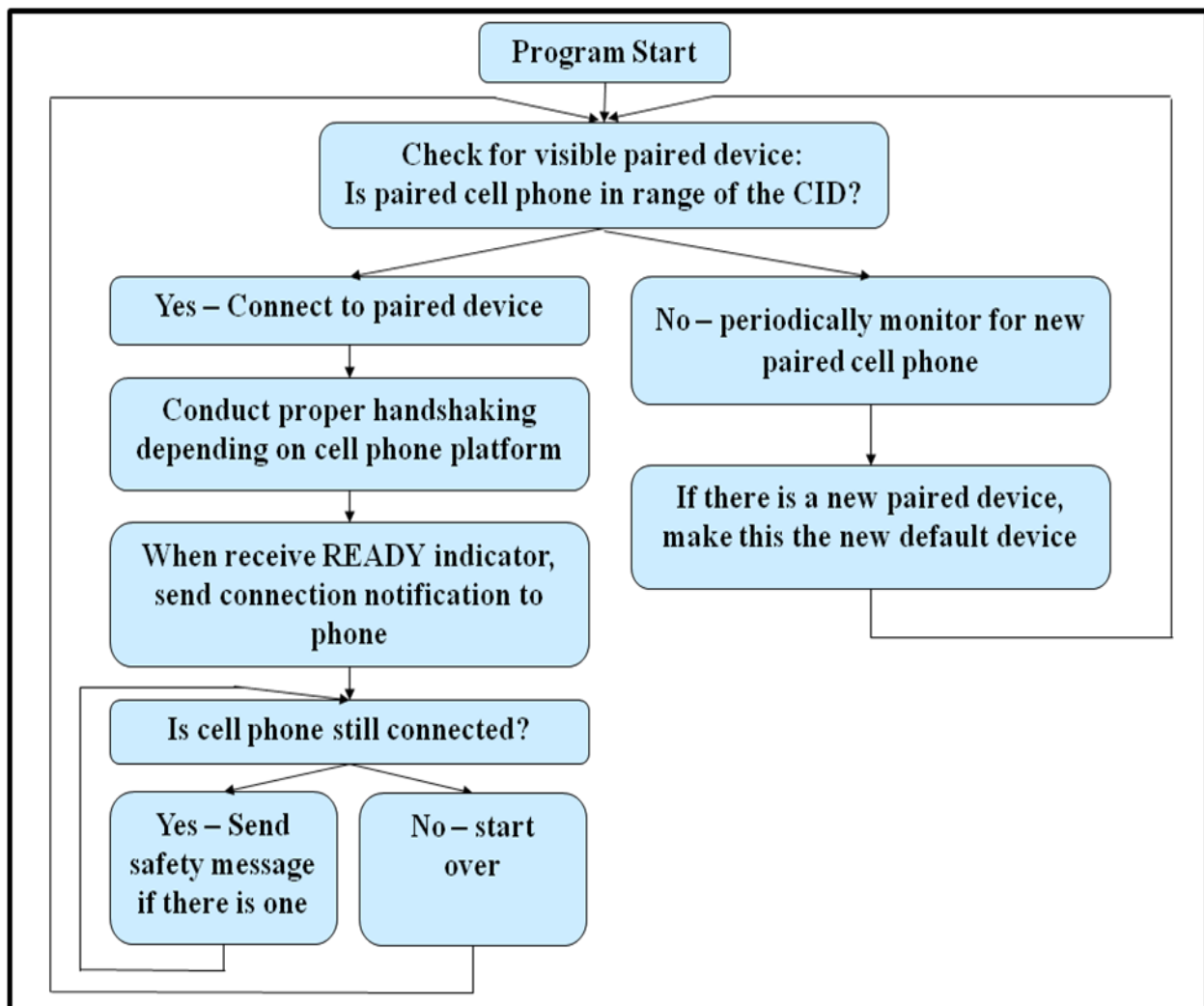
Figure 4.4. CID Application Program Flow
