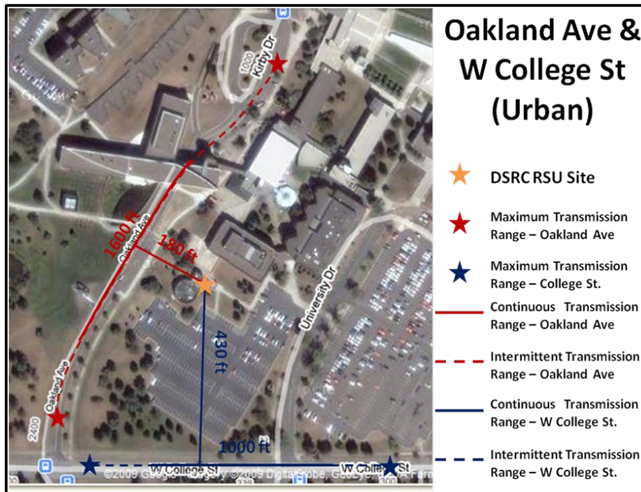
Figure 5.1. V2I Scenario 1: Elevated Fixed RSU and Mobile OBU
