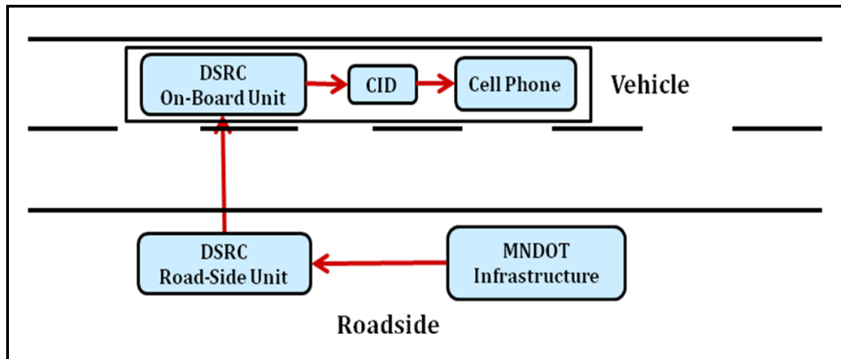
Figure 3.1. Traffic Safety Message System Architecture
