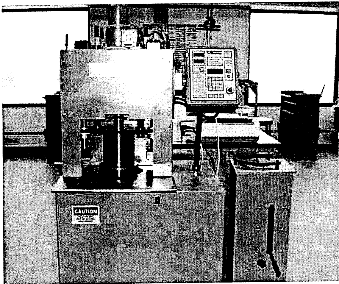
Figure 4.3 Gyratory Compactor Used at the University of Wyoming.
