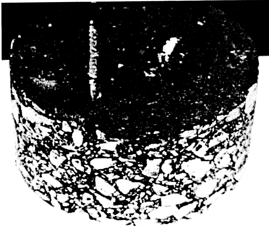
Figure 4.10 Failed GLWT Core Sample.
