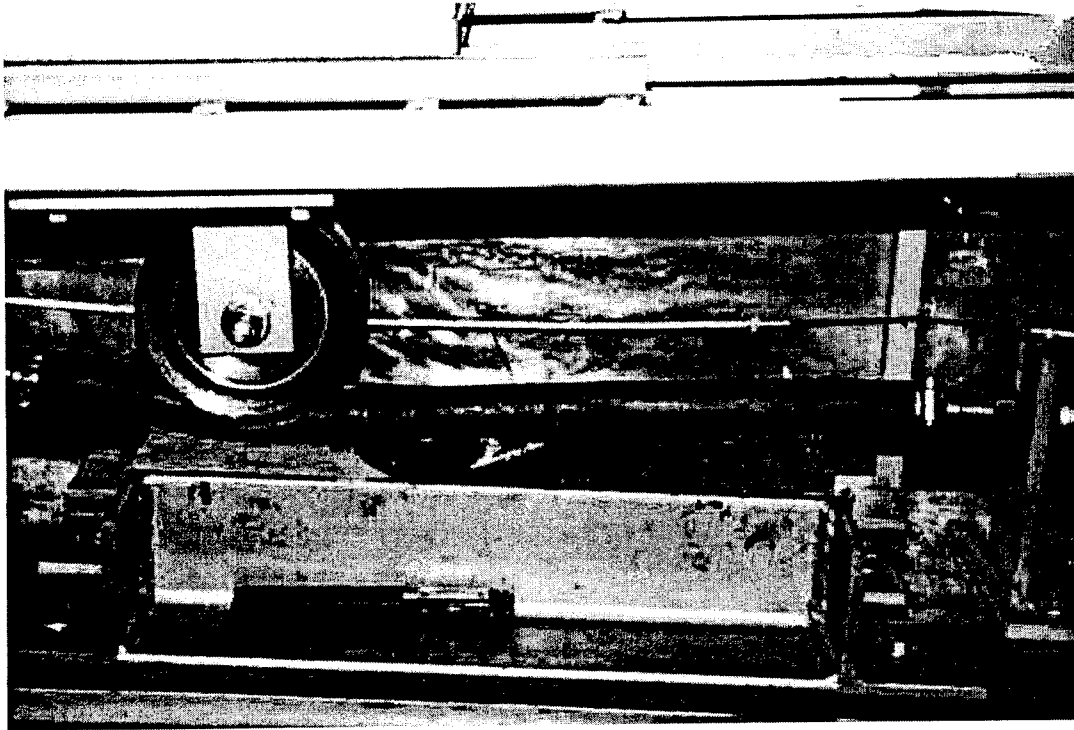
Figure 4.4 Sample Being Tested Using Georgia Loaded Wheel Tester.
