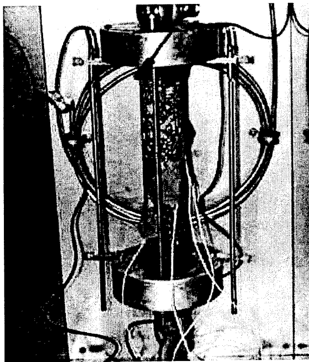
Figure 4.6 A Sample Prepared for TSRST Testing.
