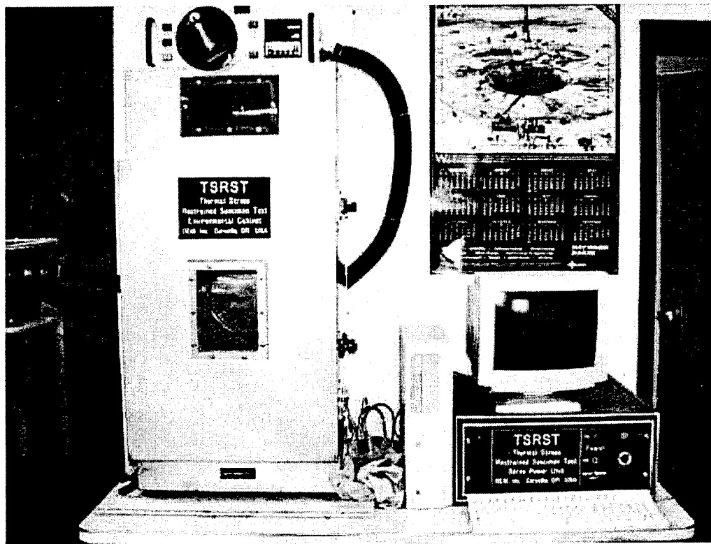
Figure 2.2 TSRST Used at the University of Wyoming.
