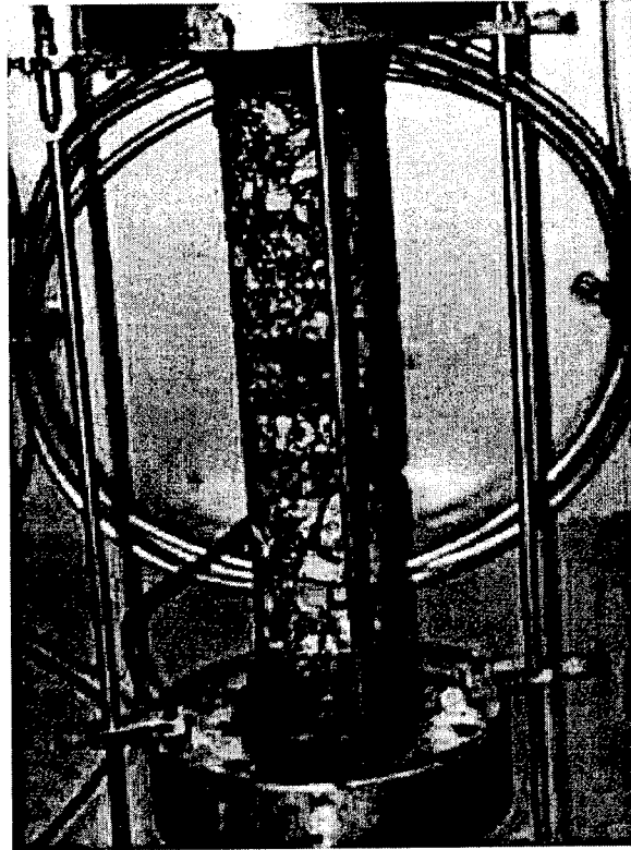
Figure 4.9 A Fractured TSRST Sample.
