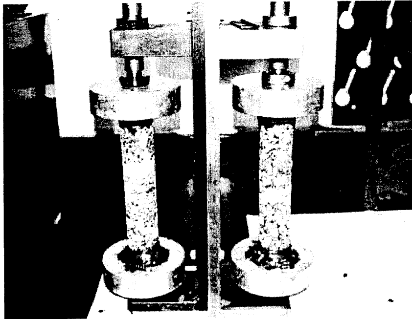
Figure 4.5 Mounting of TSRST Samples.
