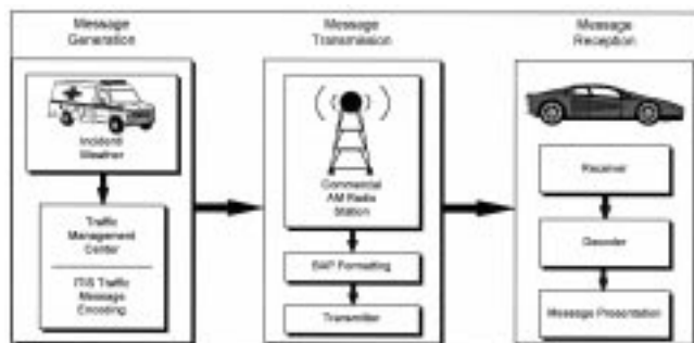
FIGURE 2 Components of Herald design concept.
