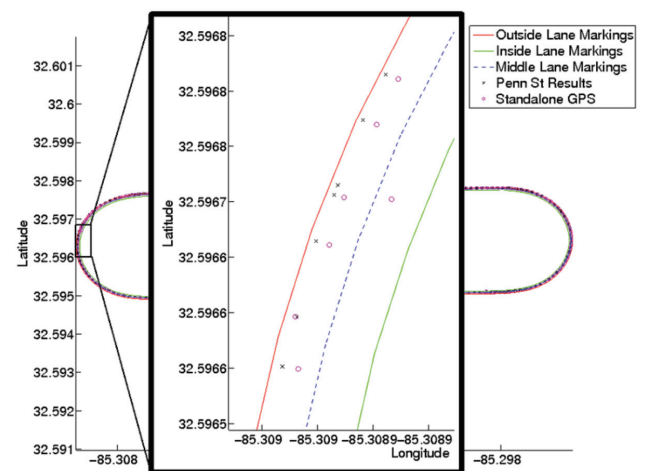
Figure 3. Chart. Penn State University's road fingerprinting concept.
