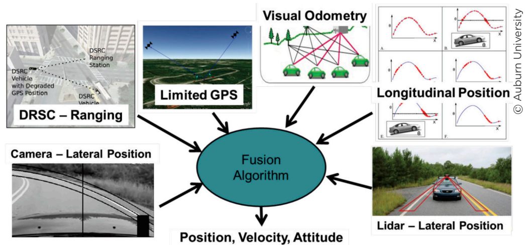
Figure 1. Diagram. The study fuses outputs from various technologies.
