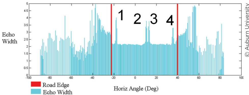
Figure 5. Chart. LIDAR Base Lane Detection.
