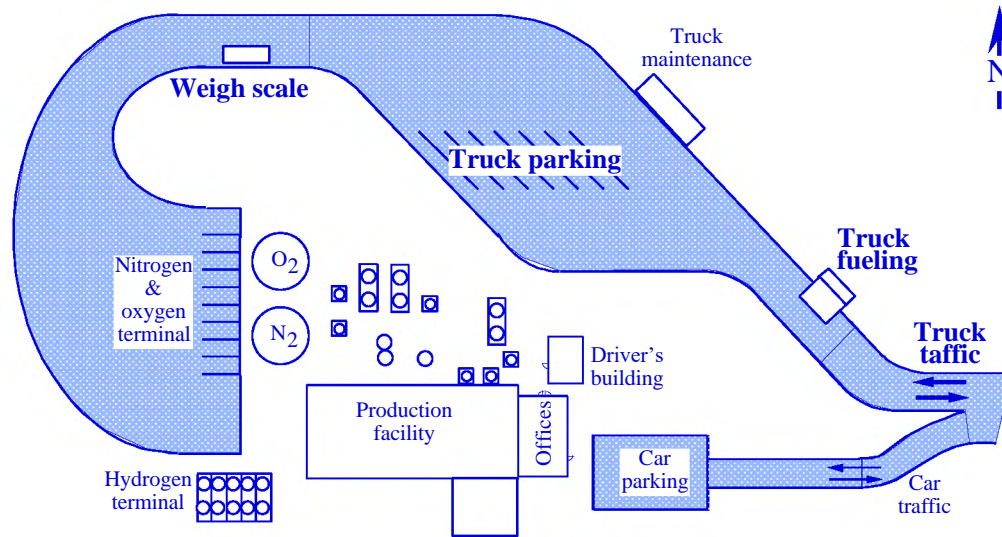
Figure 3-1. Praxair's La Porte, Indiana production and distribution facility
