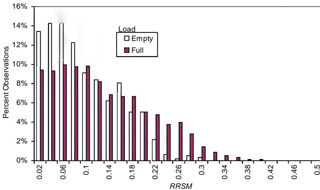
Figure 8-15. Normalized distributions of RRSM observed among non-comparable drivers on selected curves
