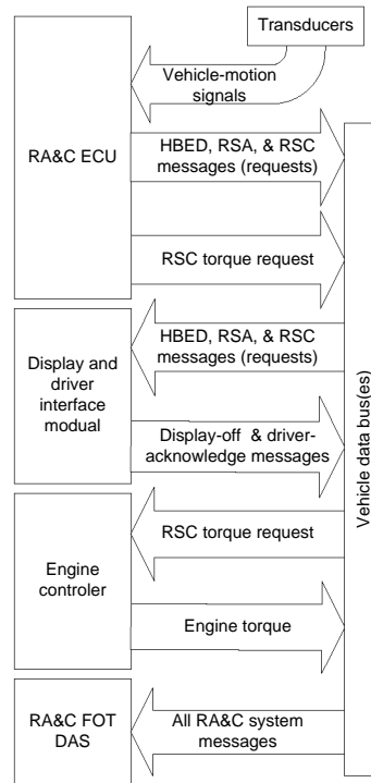
Figure 7-1. Simplified flow diagram of the messages of the RA&C system
