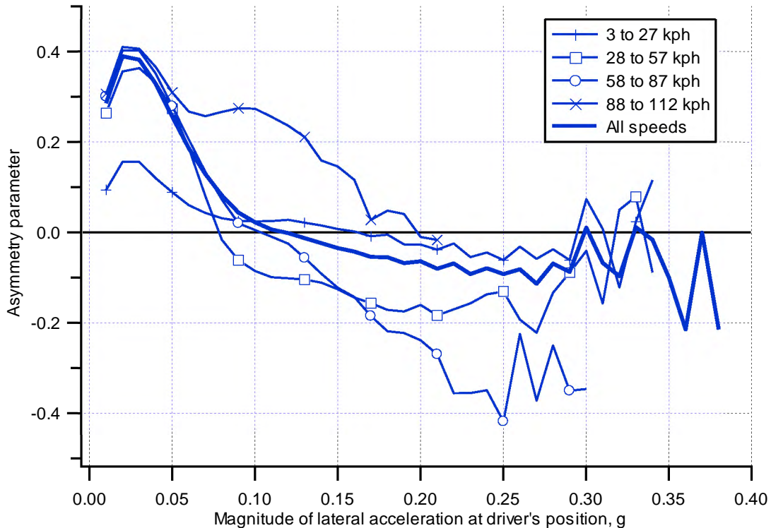
Figure 6-6. The asymmetry parameter for travel time as a function of lateral accelerations for four speed ranges and all speeds
