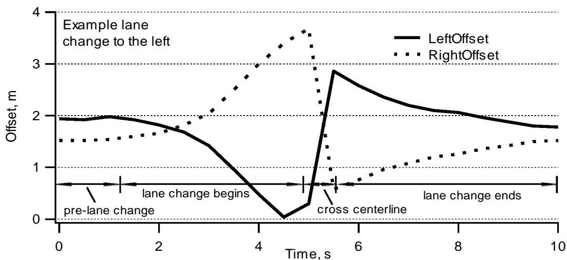
Figure A-E8. An example of the left- and right-offset values characteristic of a lane change
