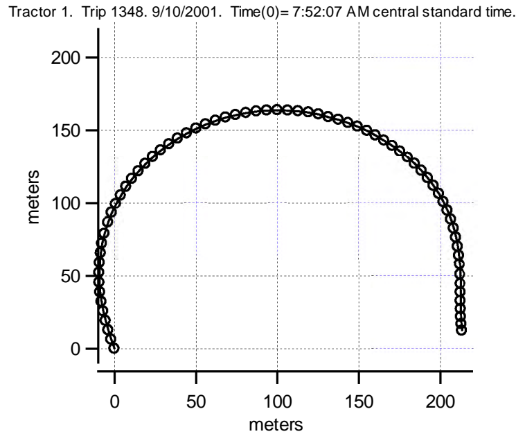
Figure 4-7. Path of the tractor in a 180 degree large-radius turn
