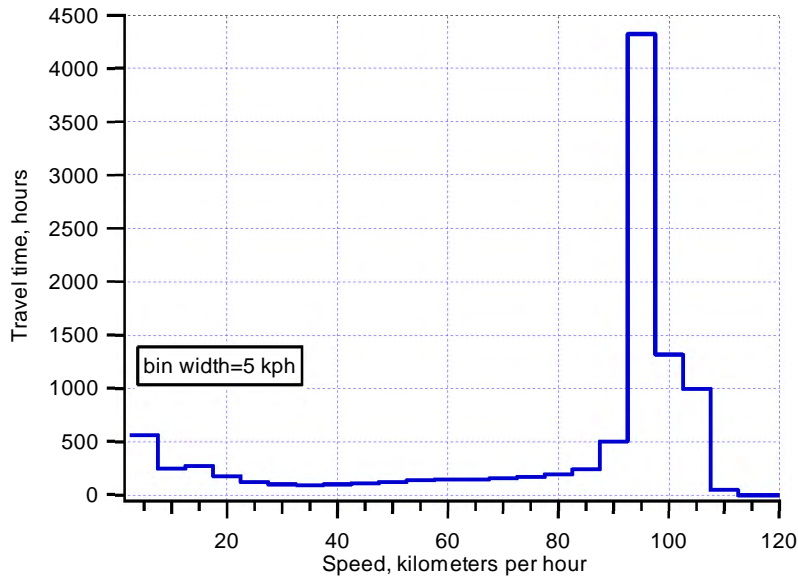
Figure 5-6. Histogram of travel time by speed
