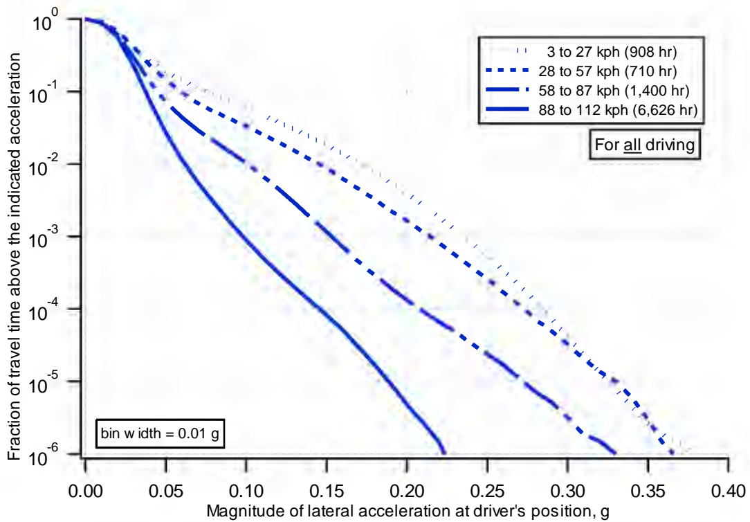
Figure 6-4. Cumulative histogram of travel time by magnitude of lateral acceleration for four speed ranges
