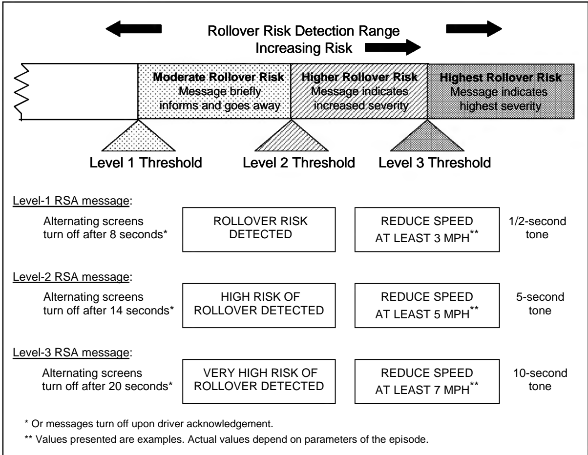
Figure 2-3. RSA concept and advisory messages.
