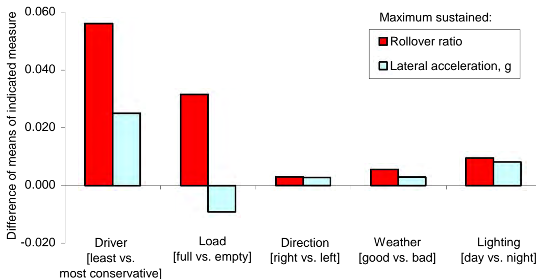
Figure 10-1. Relative strengths of different factors on turning performance 38
