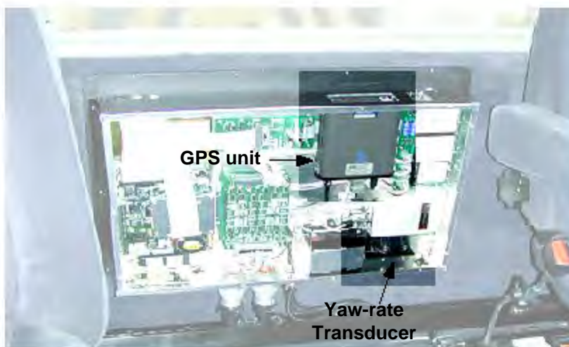
Figure 3-6. Location of GPS and yaw-rate transducer
