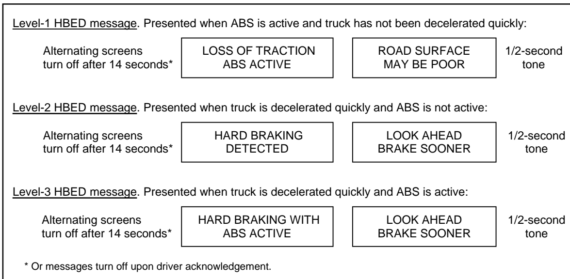
Figure 2-5. HBED advisory messages
