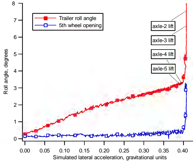
Figure A-C2. Example data from tilt-table test; 3/4 load.
