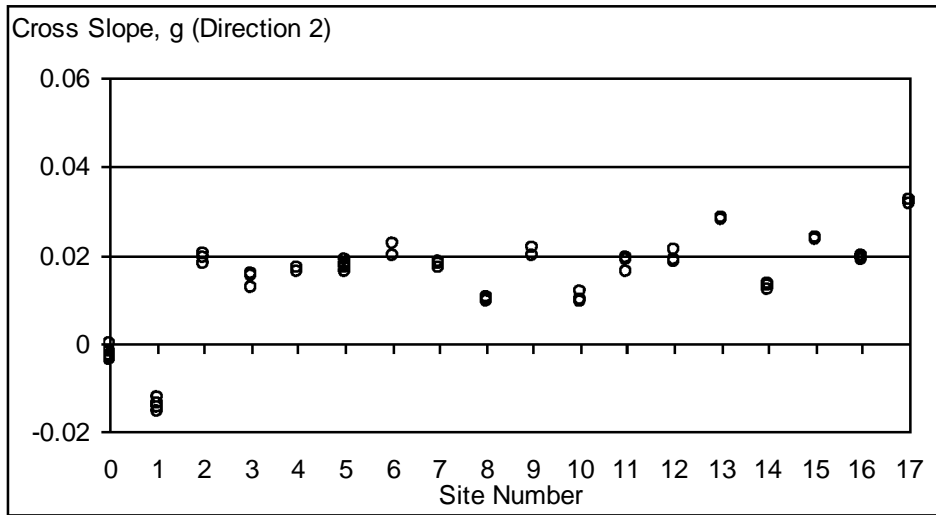
Figure A-E6. Cross slope for each site in direction 1 and 2, respectively
