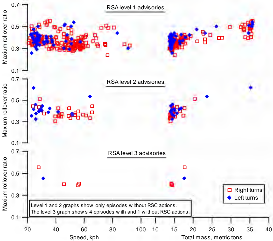
Figure 7-11. Maximum rollover ratio by speed and load for RSA episodes
