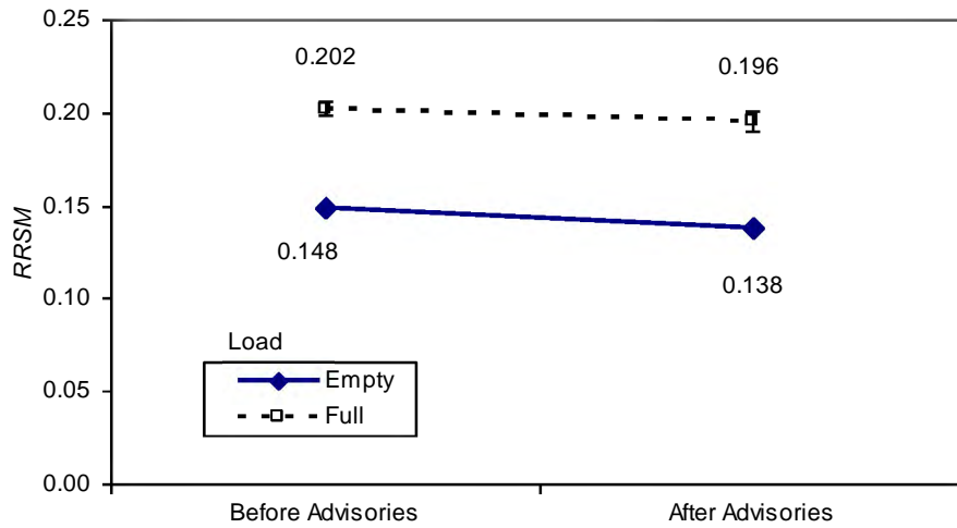
Figure 8-50. Main effects of exposure to advisory messages and load on RRSM in the interval 250 km before and after an advisory
