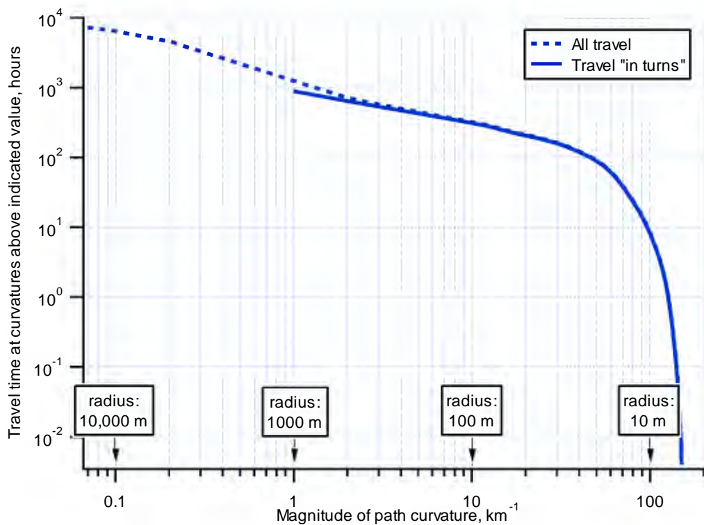
Figure 5-9. Cumulative histograms of path curvature
