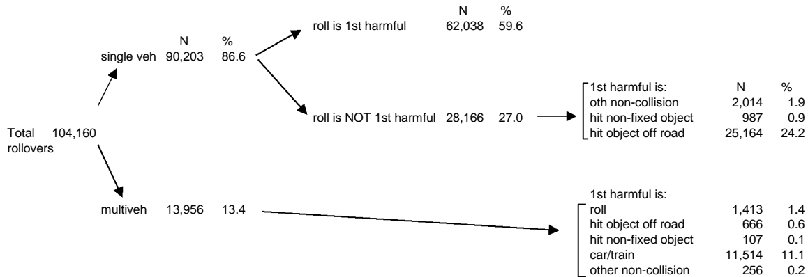
Figure A-A3—Rollover event tree, TIFA/GES 1992-1998
