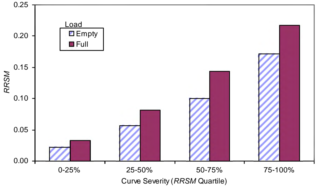
Figure 8-25. The interaction between load and curve severity
