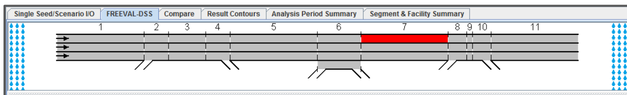
Figure 3-10. One-lane closure displayed on the facility preview graphic.
