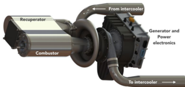
Figure 6. An 80 kW Fulcrum microturbine generator
