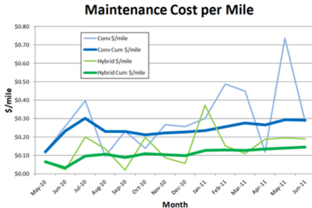
Figure 27. Hybrid vehicle maintenance cost per mile data from NREL (Reference (14))
