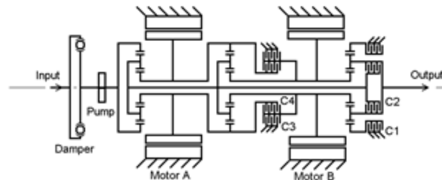
2-Mode Hybrid Configuration
