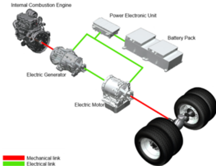
Figure 10 BAE System Series Hybriddrive
