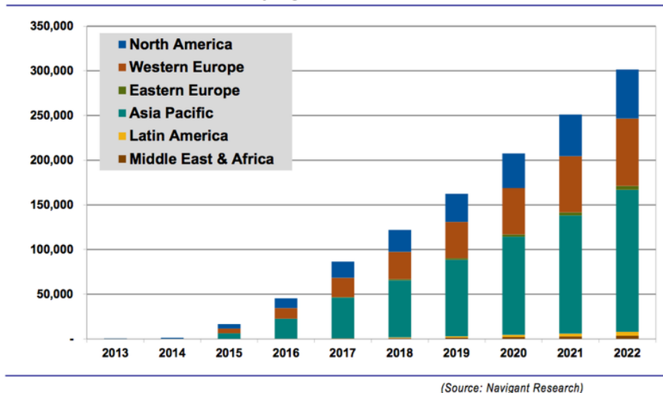
Figure 7. Wireless EV charging sales projection [Navigant Research]
