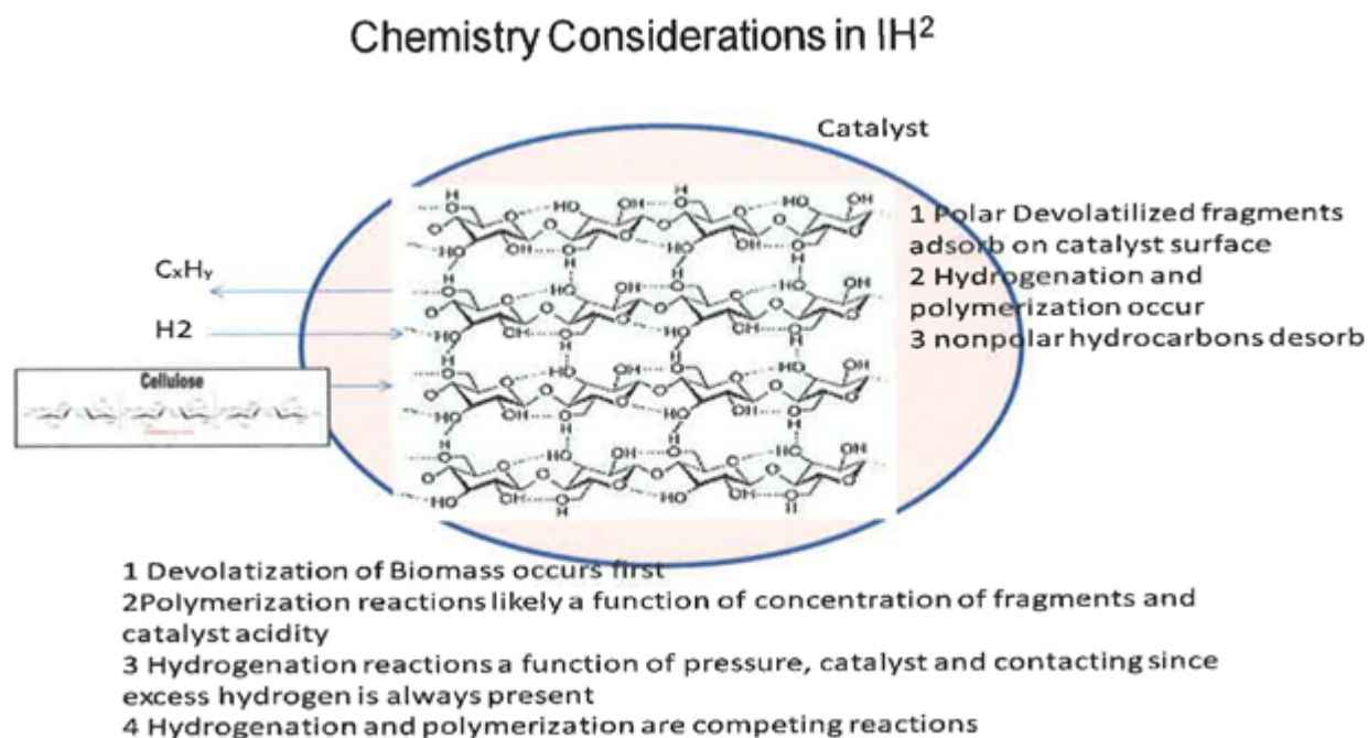
Figure 2-Chemistry of Hydropyrolysis
