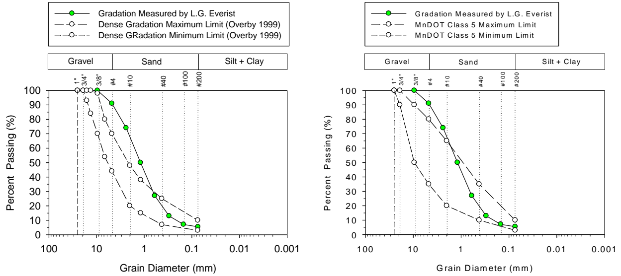
Figure 38. Gradation of Source 2 aggregate in comparison with Overby (1999) limits and MnDOT Class 5 limits
