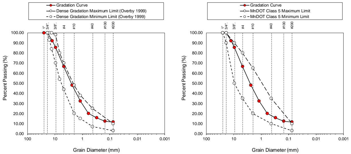
Figure 39. Gradation of Source 3 Type A aggregate in comparison with Overby (1999) limits and MnDOT Class 5 limits
