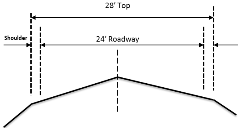
Figure 83. Roadway cross-section used in the analysis
