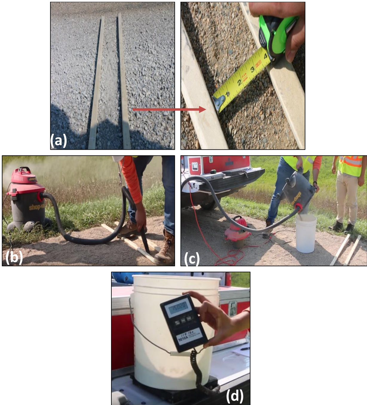
Figure 59. Equipment and steps of loose materials test: (a) making a single lane (148 in. × 4 in.), (b) collecting excessive aggregate between the surface of two wooden sticks, (c) placing collected aggregate, and (d) measuring the weight of collected aggregate
