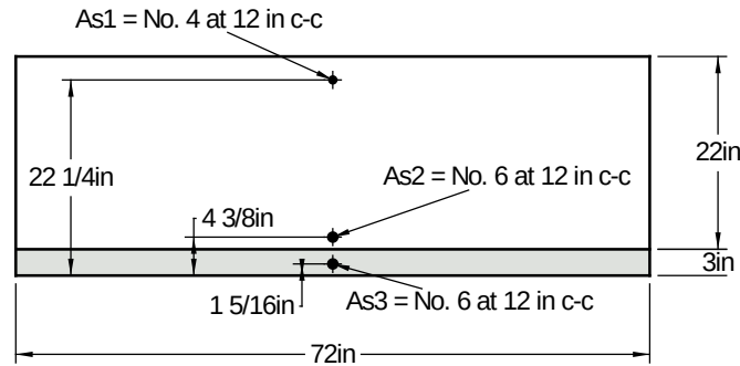
Section 3 - Longitudinal Section through Precast Flange
