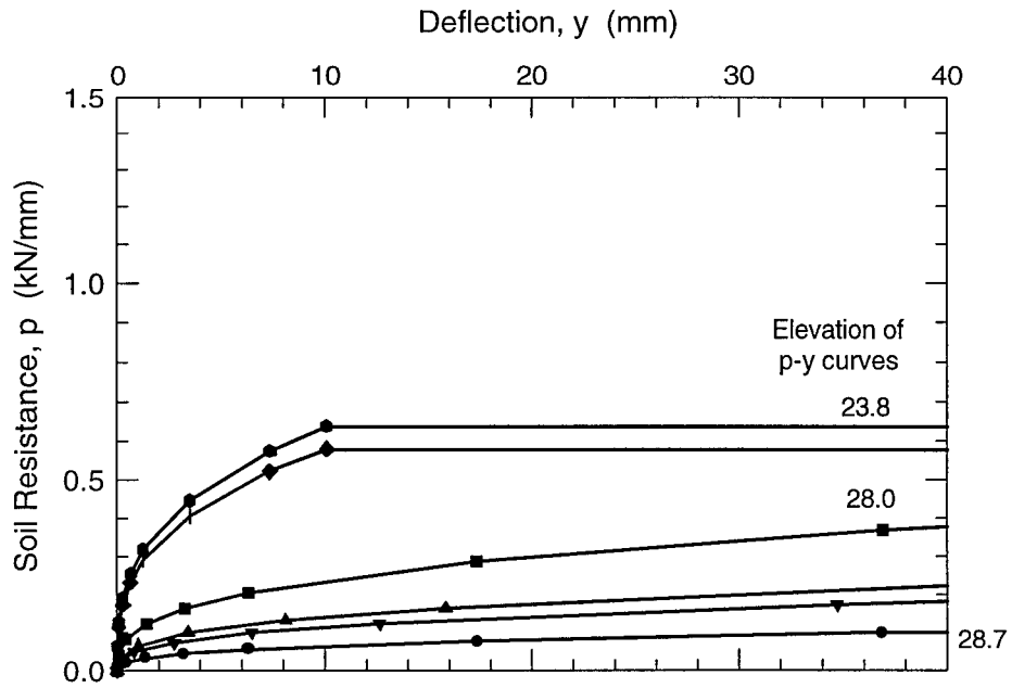
(a) Single pile p-y curves.
