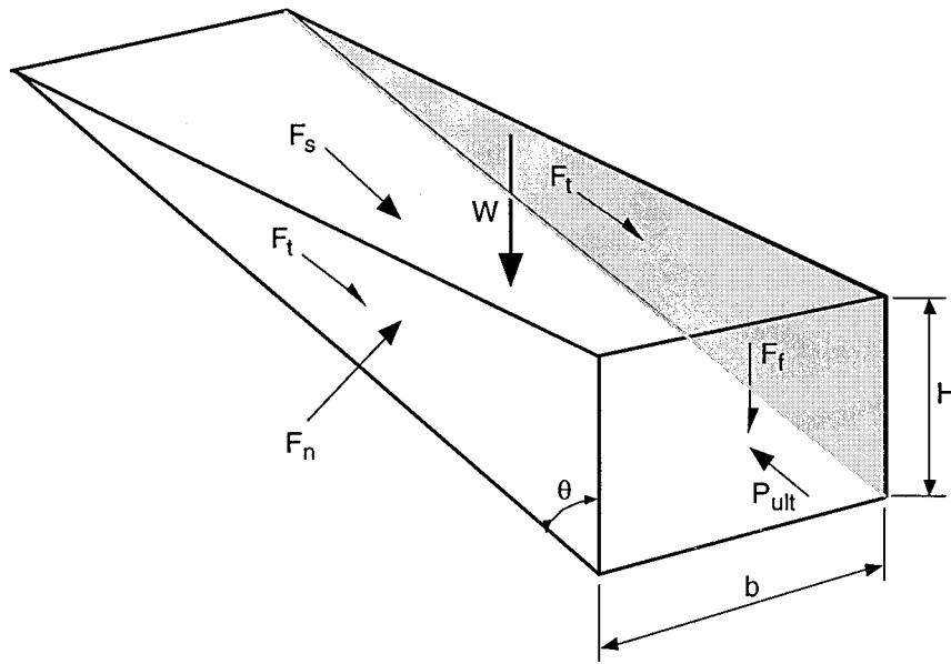
Orthogonal view of failure wedge
