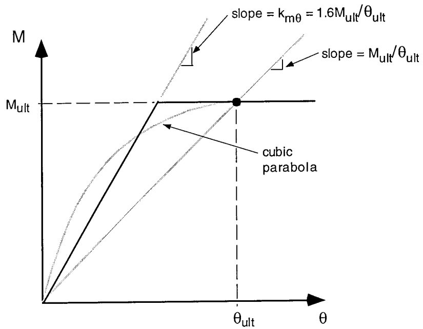
(a) Graphical illustration of k_{m\theta} approximation.
