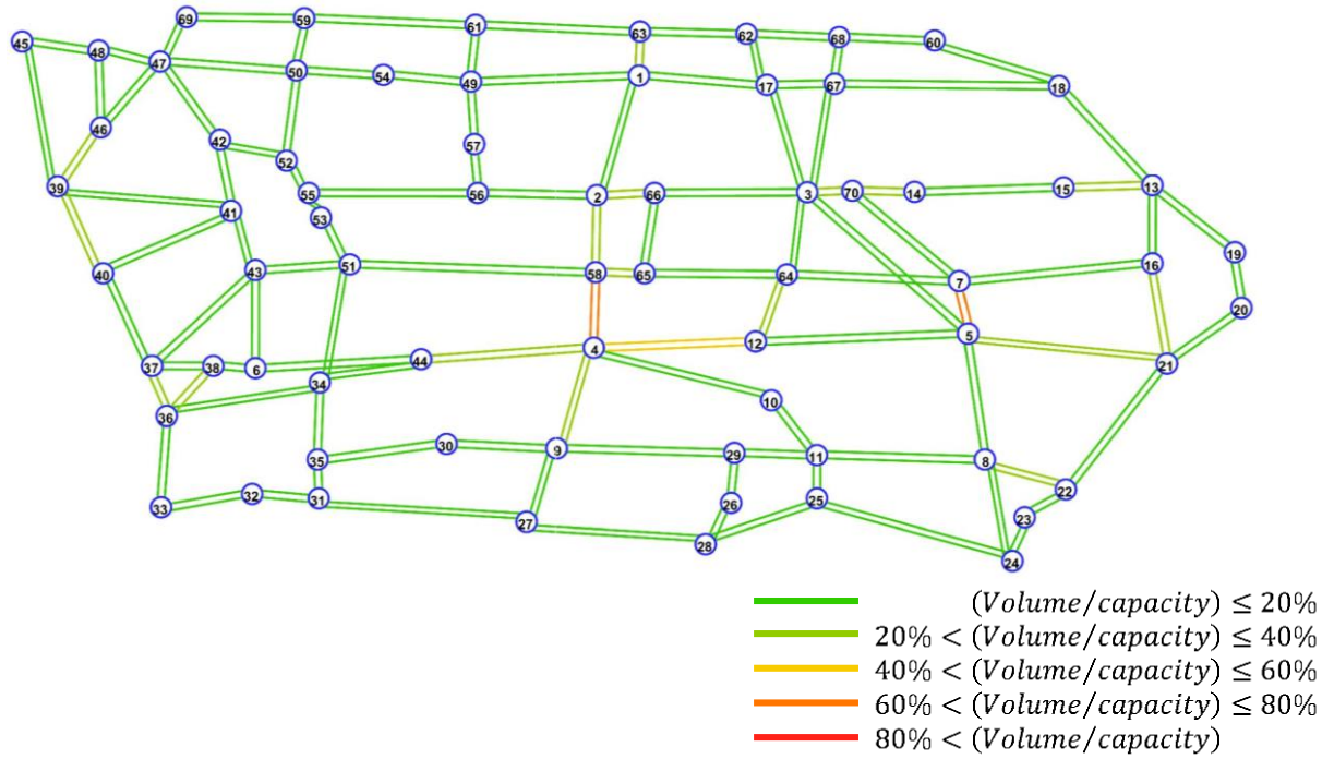
Figure 4. Iowa transportation network without expansion and without disruption
