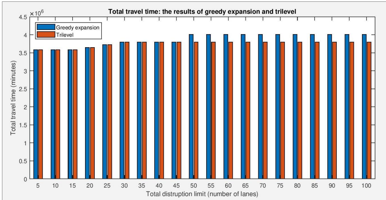
Figure 9. The comparison of total travel times between greedy expansion and the trilevel optimization model for different values of disruption limit from 5 to 100 lanes
