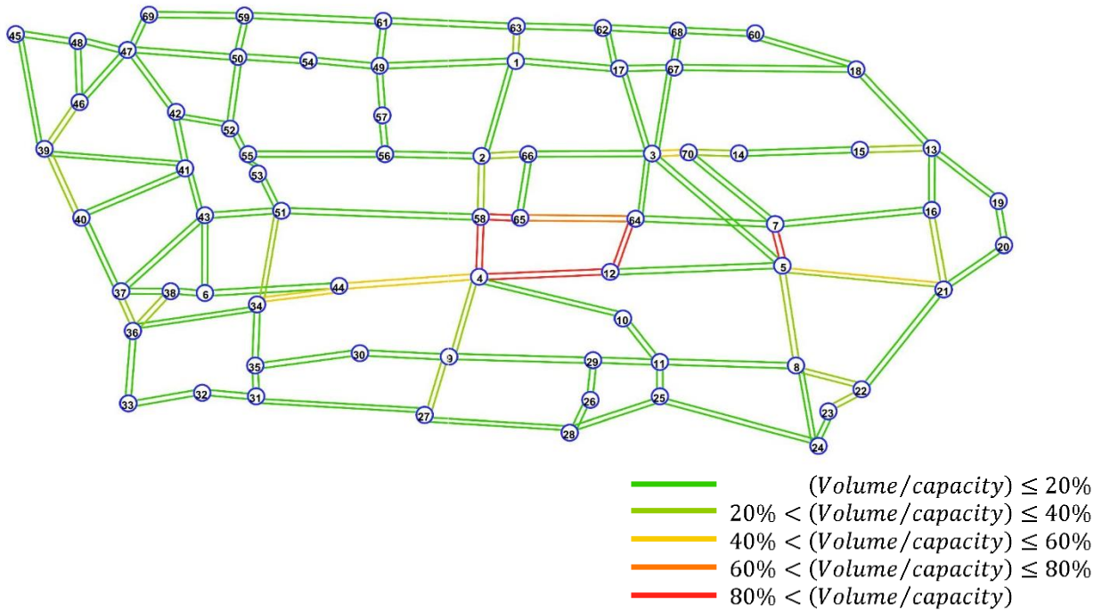
Figure 6. Iowa transportation network when the total disruption is 5 lanes
