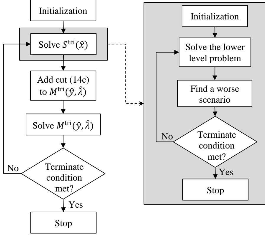
Figure 1. The algorithm flowchart
