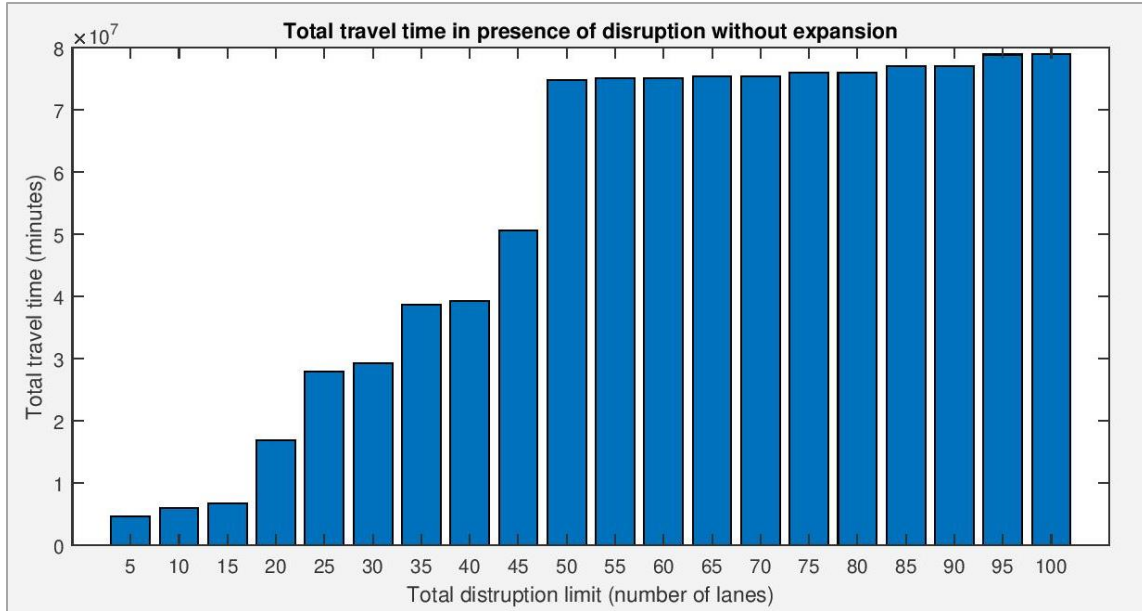
Figure 5. Total travel time in presence of disruption without expansion for different values of disruption limit from 5 to 100 lanes
