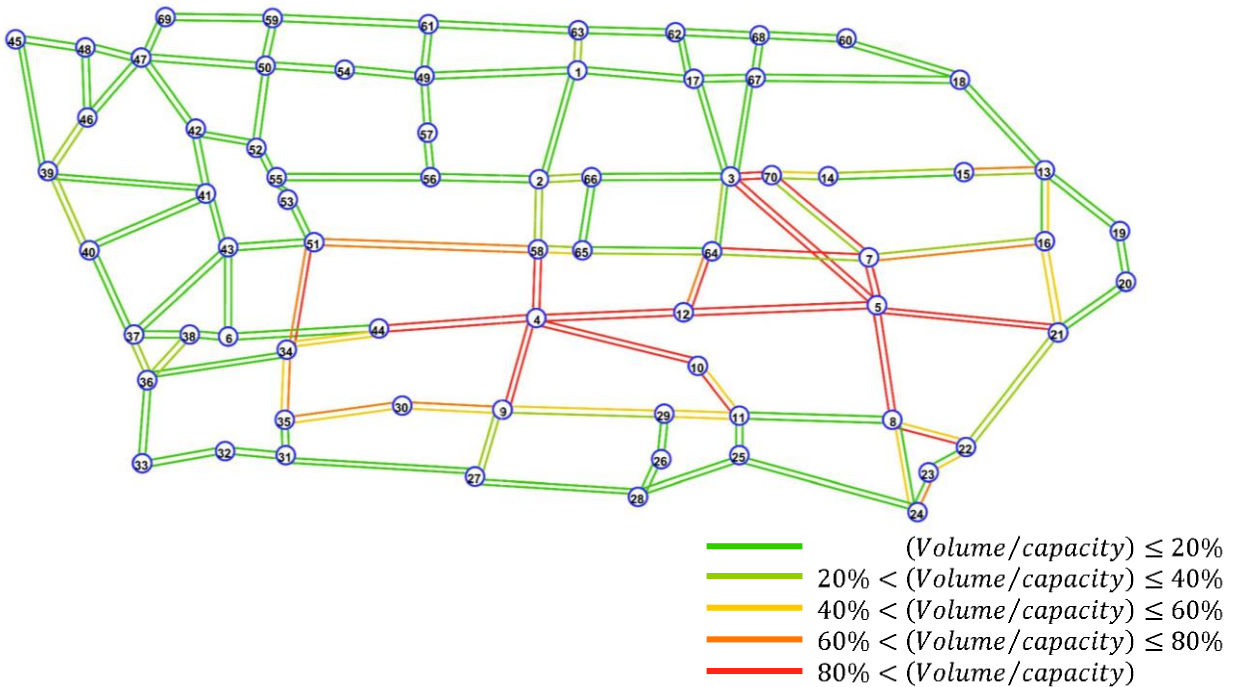
Figure 7. Iowa transportation network when the total disruption is 50 lanes
