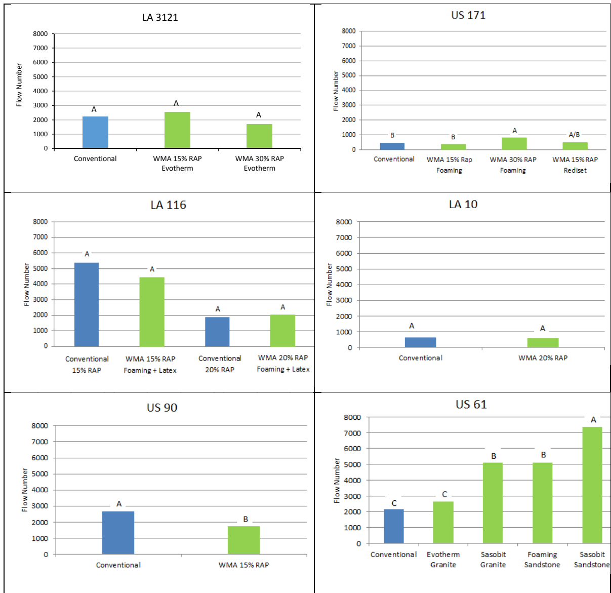
Figure 93 Statistical analysis of flow number results
