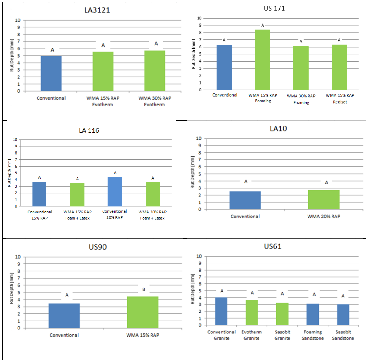
Figure 97 Statistical analysis of LWT results
