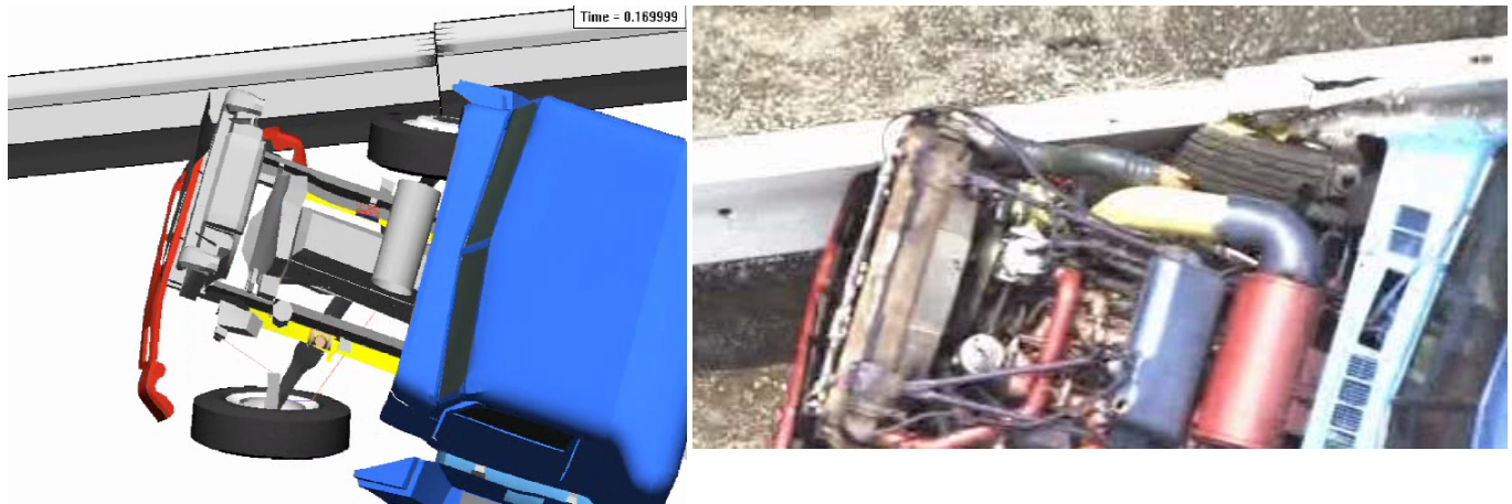
Figure 122. Illustration / Photo. Initial tire impact interaction with barrier
