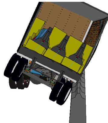
Figure 44. [CONTINUED] Photograph / Illustration. Sequential views of MwRSF Test TL5CMB-2 and FE Model simulation from an upstream viewpoint
