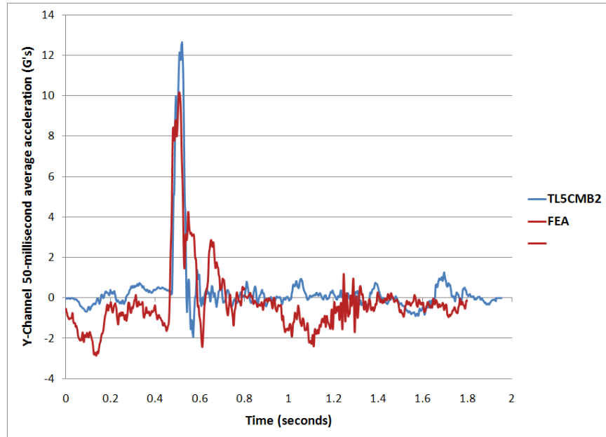
Figure 56. Chart. 50-millisecond moving average of the lateral acceleration-time history plot at rear of trailer comparing FE results to Test TL5CMB2
