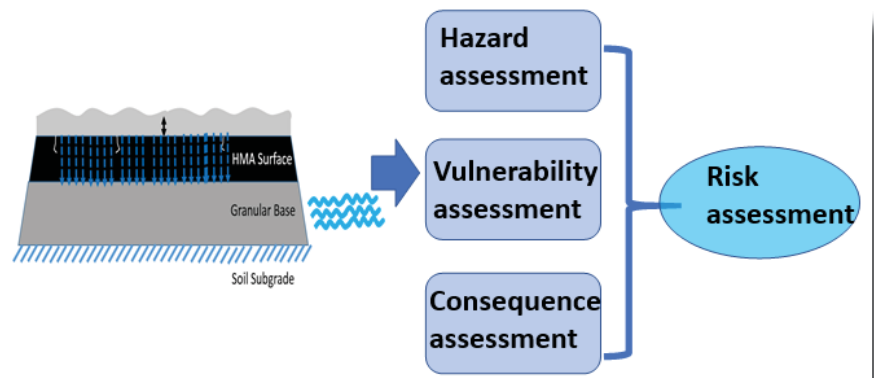
Figure 1 Schematics of a hierarchical evaluation protocol of flood-induced damage to pavement
