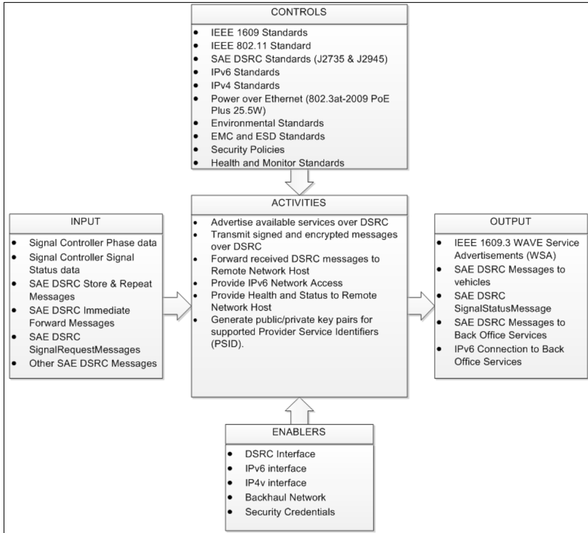
Figure 2-6. Diagram. Context Diagram for a Roadside Unit.
