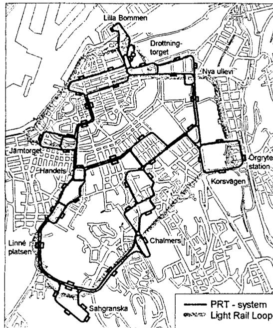
Figure 7.4. PRT network for central Göteborg
