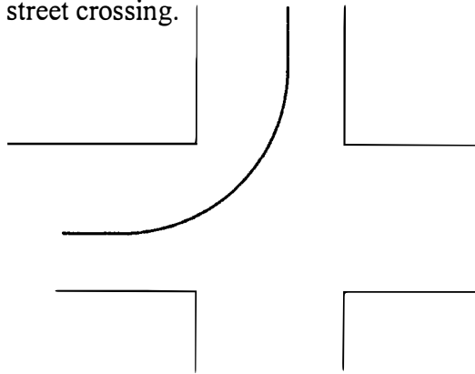
Figure 2.11. Guide-way curve with a 20-meter radius in a street crossing with 18 meters facade distance.
