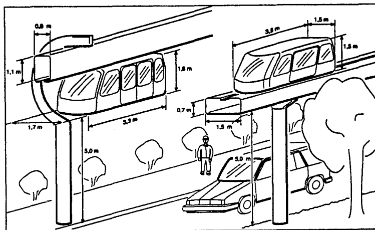
Figure 2.10. Perspective of suspended and supported systems (Stockholm Regional Planning Office)
