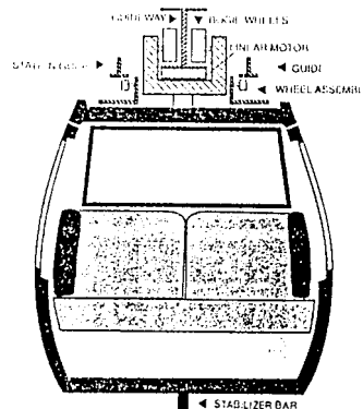
Figure 2.8. Ultra-Wave PRT (USA)
