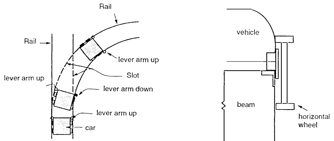
Figure 5.4. Switching with lever arm
