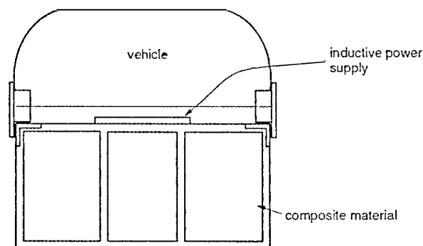
Figure 5.1. Cross-section of beam and vehicle
