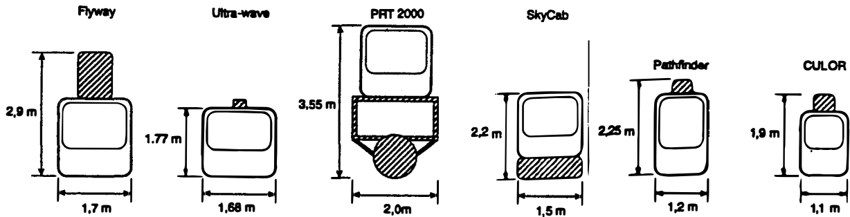
Figure 2.9. Comparative dimensions of guide-ways and vehicles (Stockholm Regional Planning Office)
