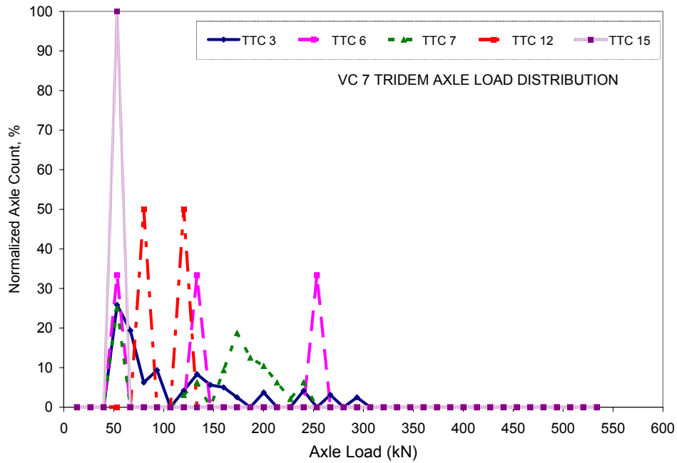
Figure 3.49 VC 7 Tridem Axle Load Distribution
