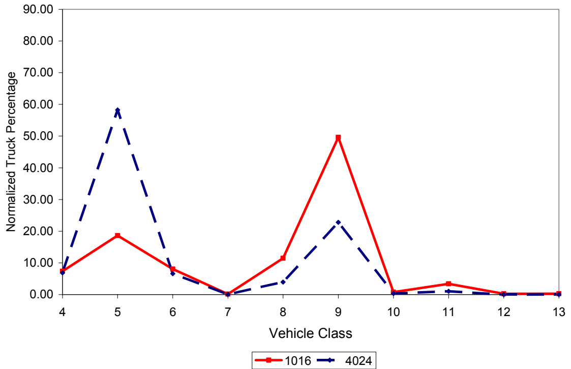
Figure 3.26 Vehicle Class Distribution for Functional Class 14
