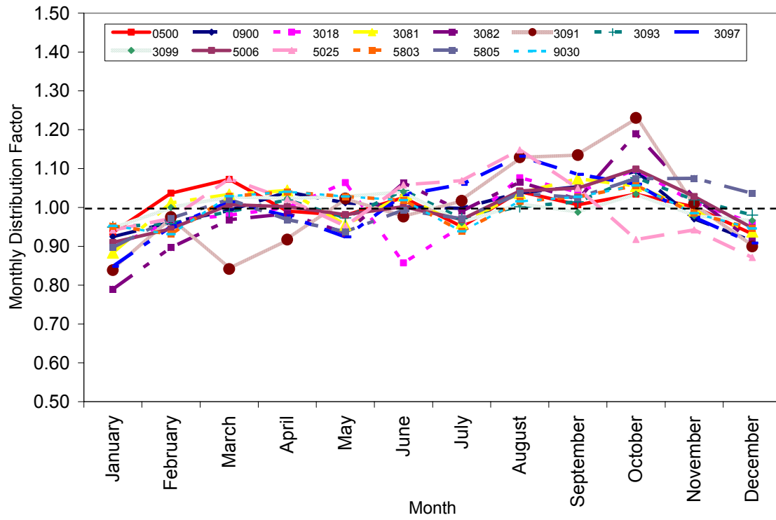
Figure 3.34 Monthly Distribution Factors for TTC 3
