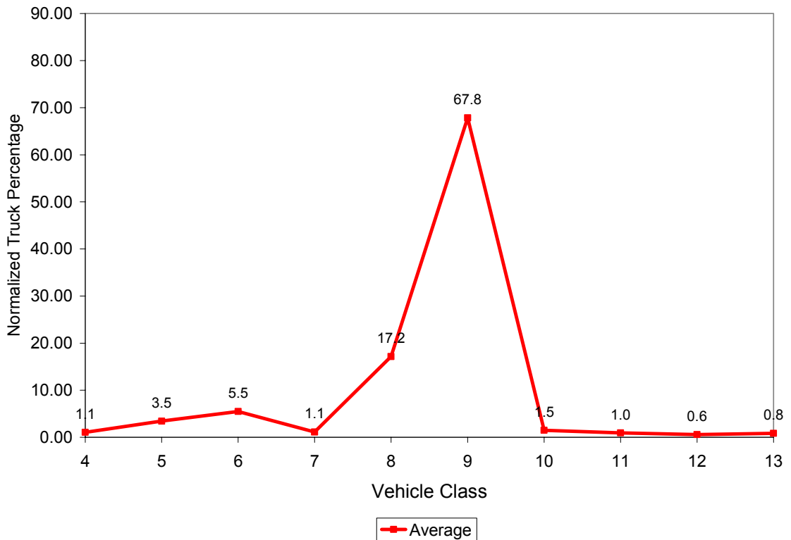
Figure 3.14 Vehicle Class Distribution for 3091
