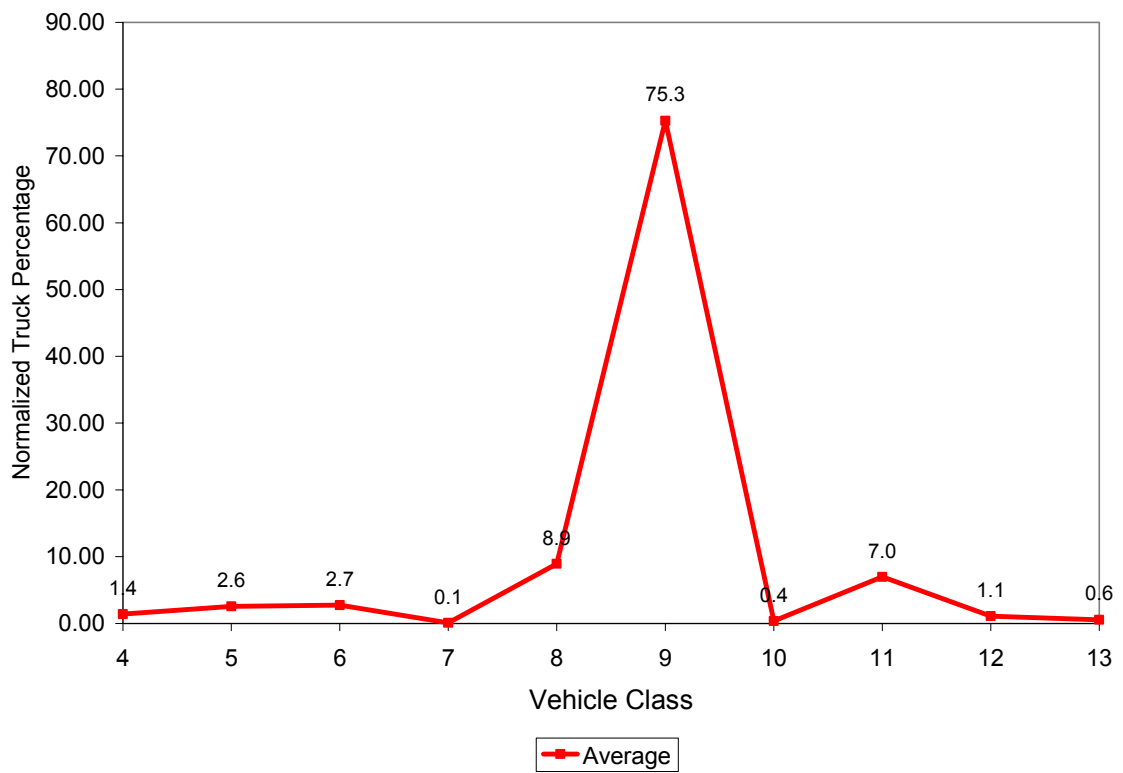
Figure 3.21 Vehicle Class Distribution for 5803
