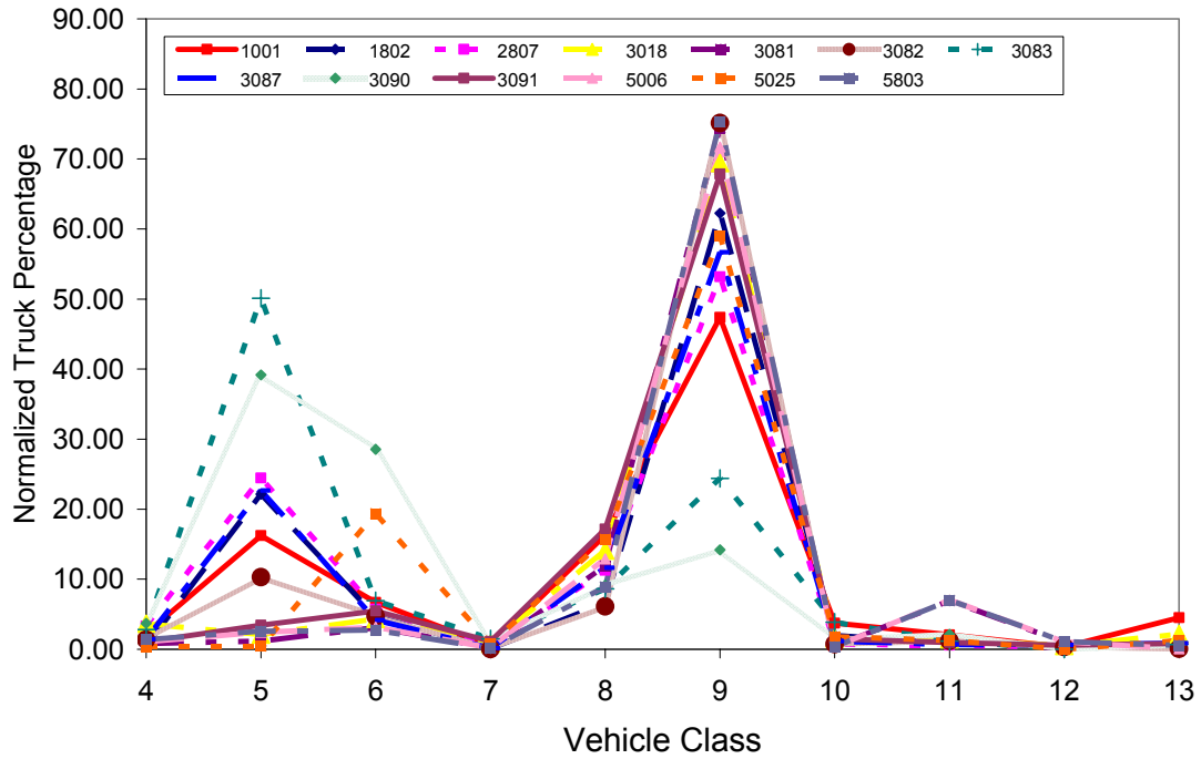
Figure 3.25 Vehicle Class Distribution for Functional Class 2
