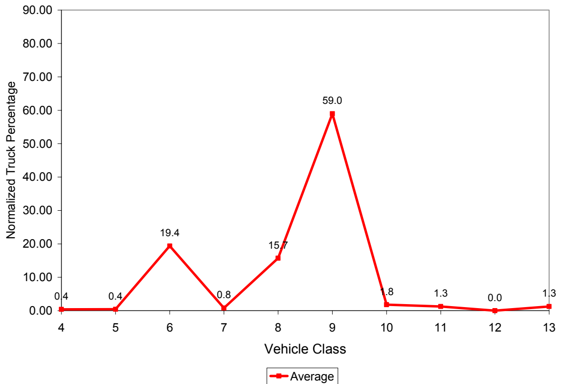
Figure 3.20 Vehicle Class Distribution for 5025
