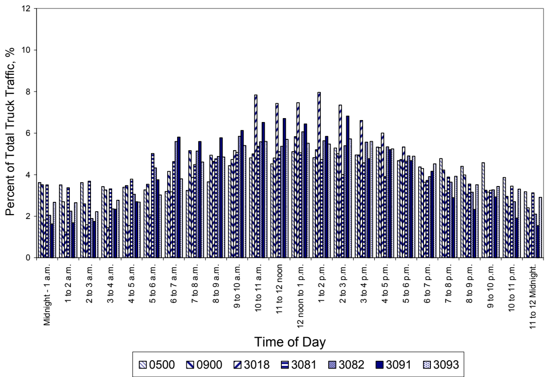
Figure 3.39 Hourly Truck Distribution for TTC 3 (1 st seven sites)
