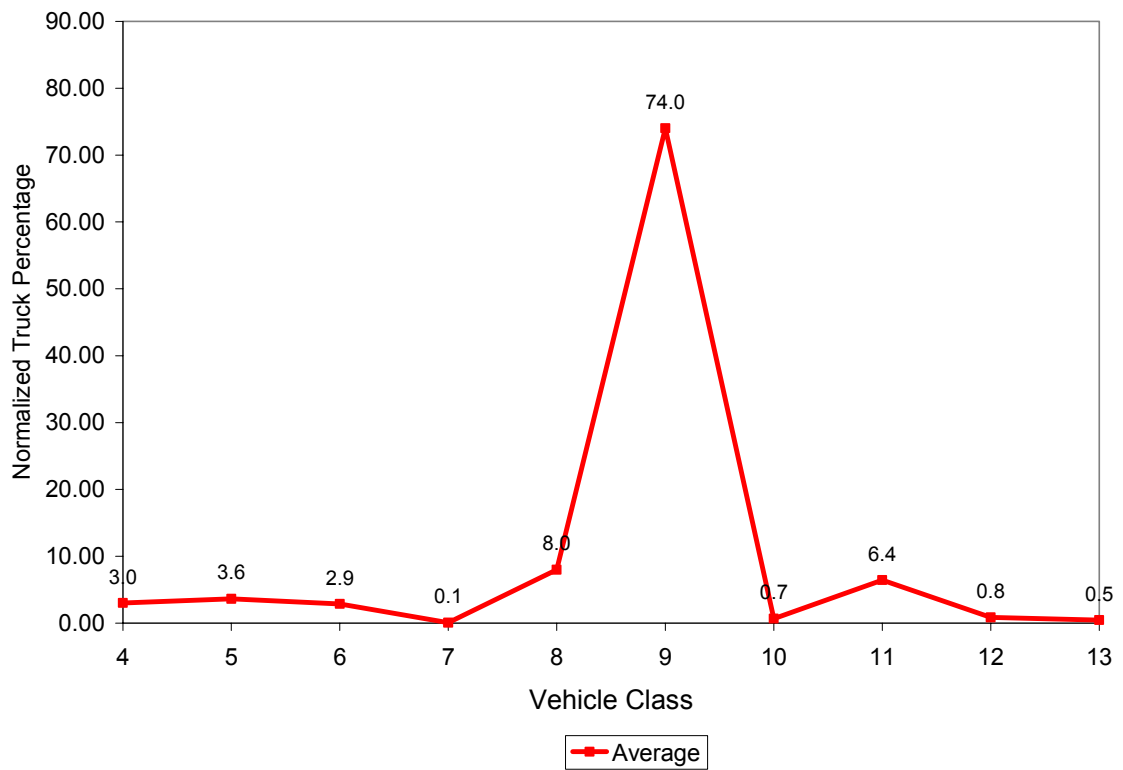
Figure 3.2 Vehicle Class Distribution for 0500
