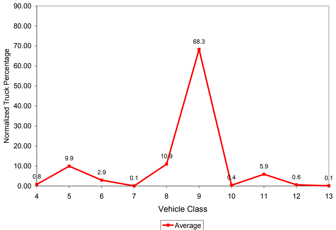
Figure 3.16 Vehicle Class Distribution for 3097
