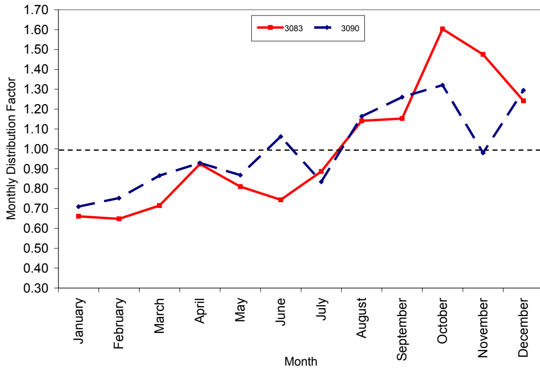
Figure 3.38 Monthly Distribution Factors for TTC 15
