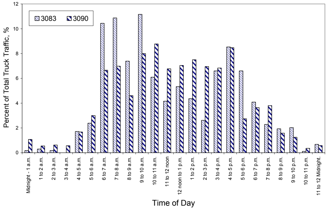
Figure 3.44 Hourly Truck Distribution for TTC 15
