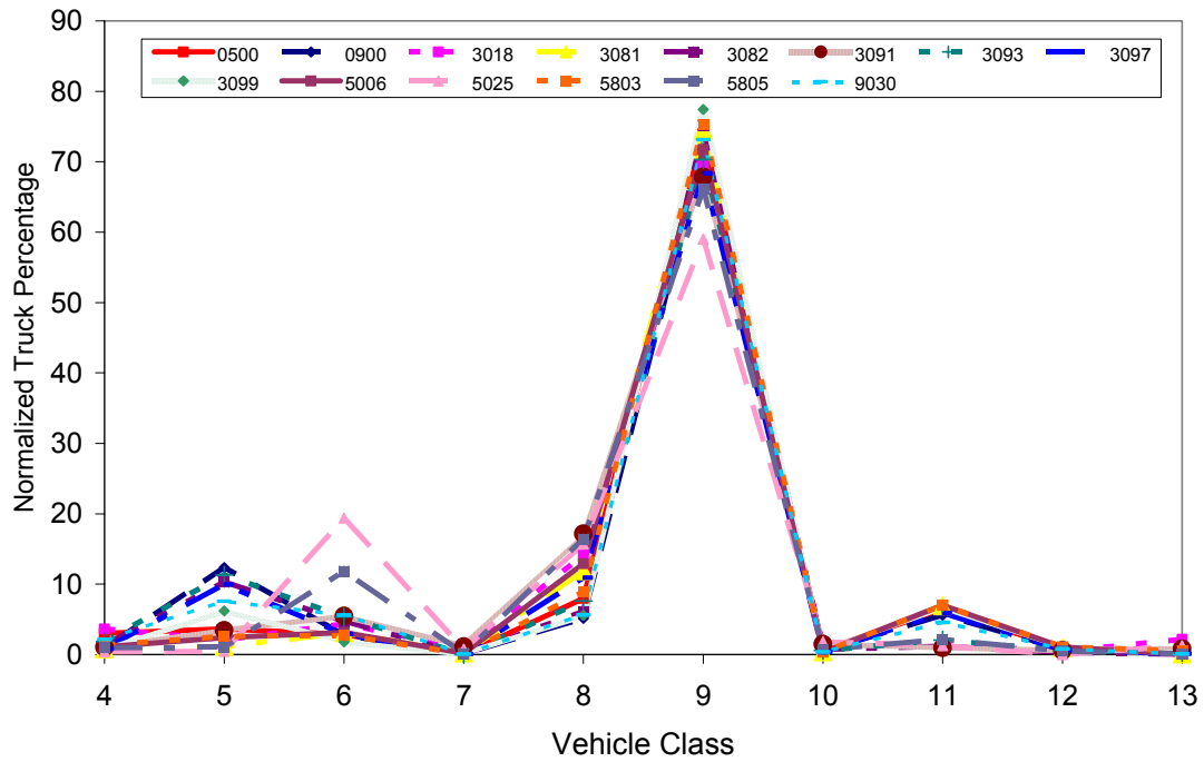
Figure 3.27 Vehicle Class Distribution for TTC 3
