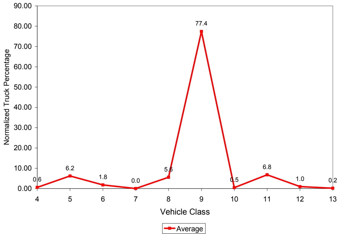
Figure 3.17 Vehicle Class Distribution for 3099
