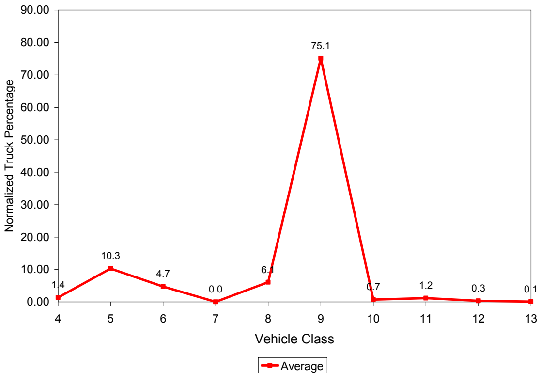
Figure 3.10 Vehicle Class Distribution for 3082
