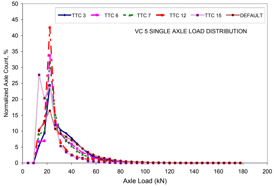
Figure 3.45 VC 5 Single Axle Load Spectra for TTC Groups
