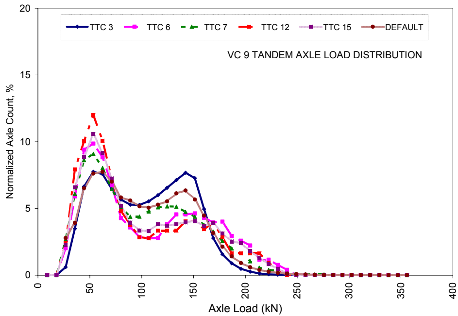
Figure 3.48 VC 9 Tandem Axle Load Spectra for TTC Groups
