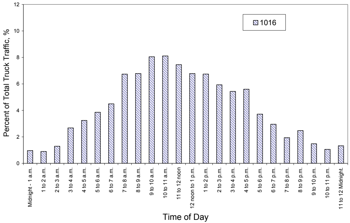
Figure 3.41 Hourly Truck Distribution for TTC 6
