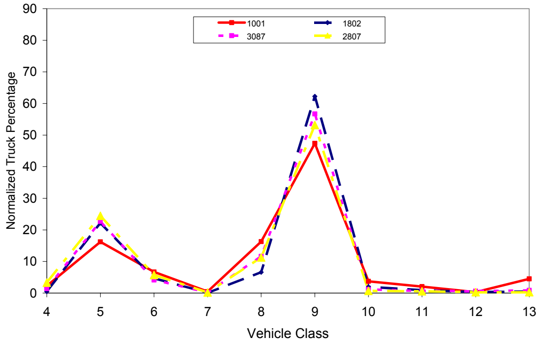
Figure 3.28 Vehicle Class Distribution for TTC 7
