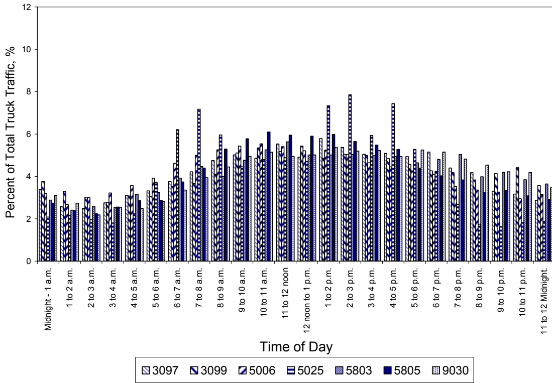
Figure 3.40 Hourly Truck Distribution for TTC 3 (2 nd seven sites)
