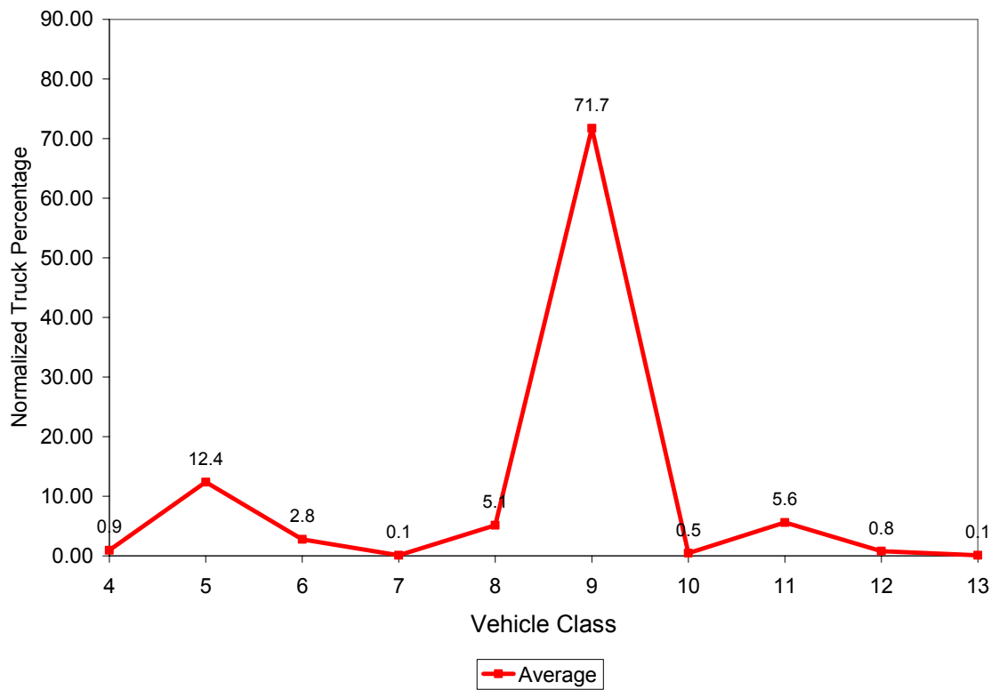
Figure 3.3 Vehicle Class Distribution for 0900
