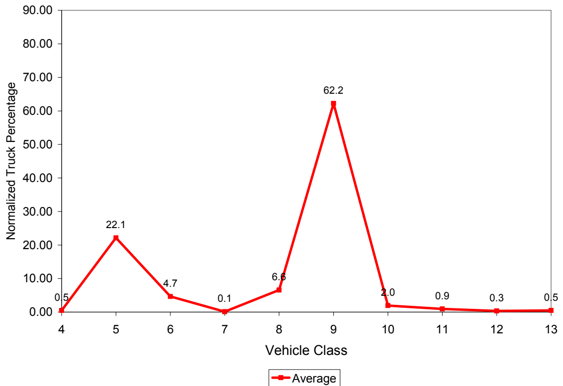
Figure 3.6 Vehicle Class Distribution for 1802
