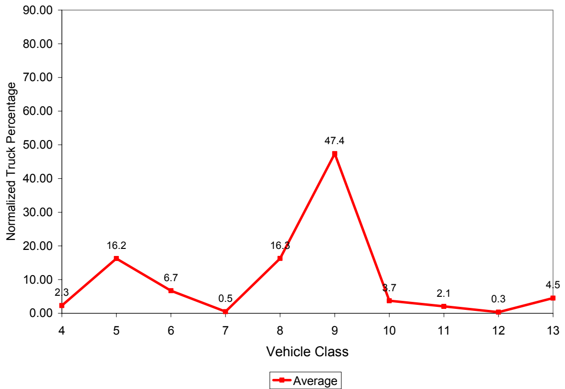
Figure 3.4 Vehicle Class Distribution for 1001
