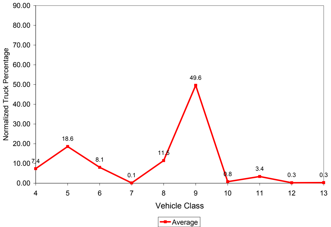
Figure 3.5 Vehicle Class Distribution for 1016
