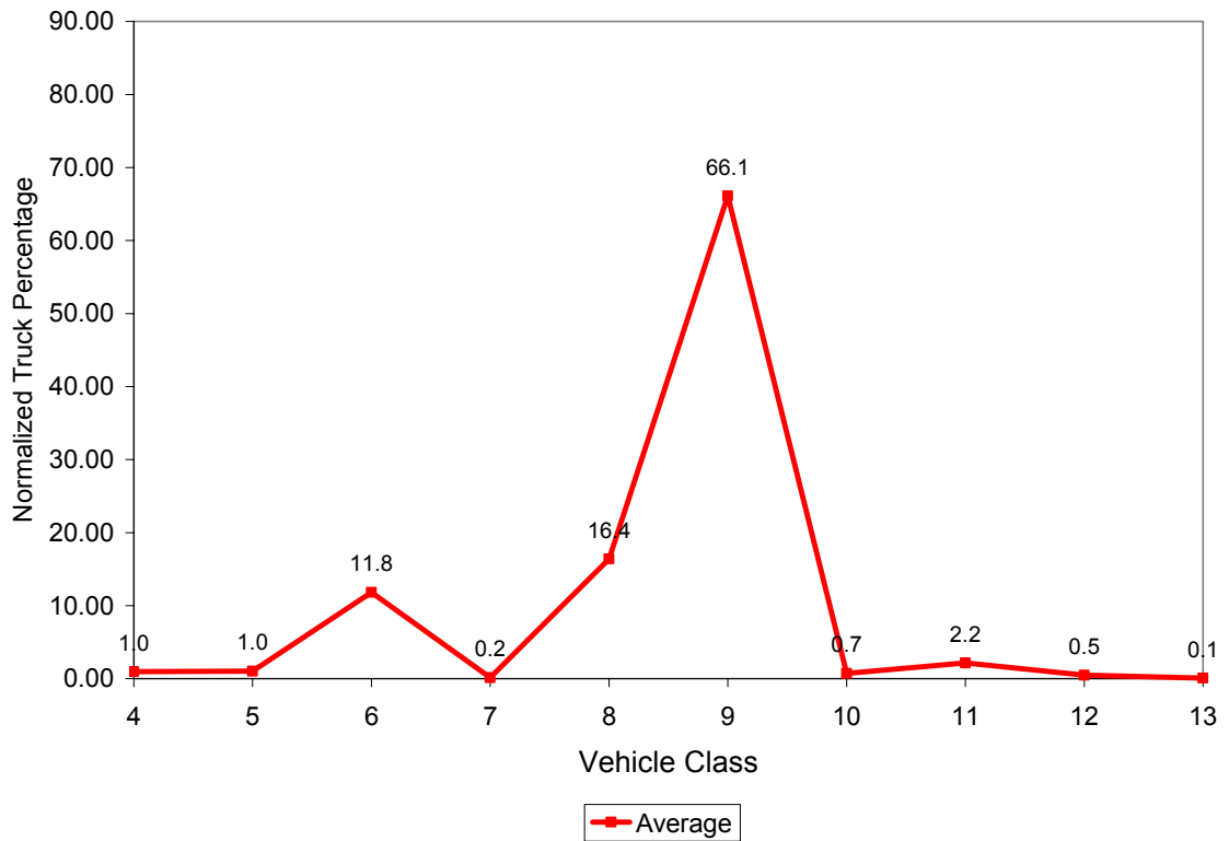
Figure 3.22 Vehicle Class Distribution for 5805
