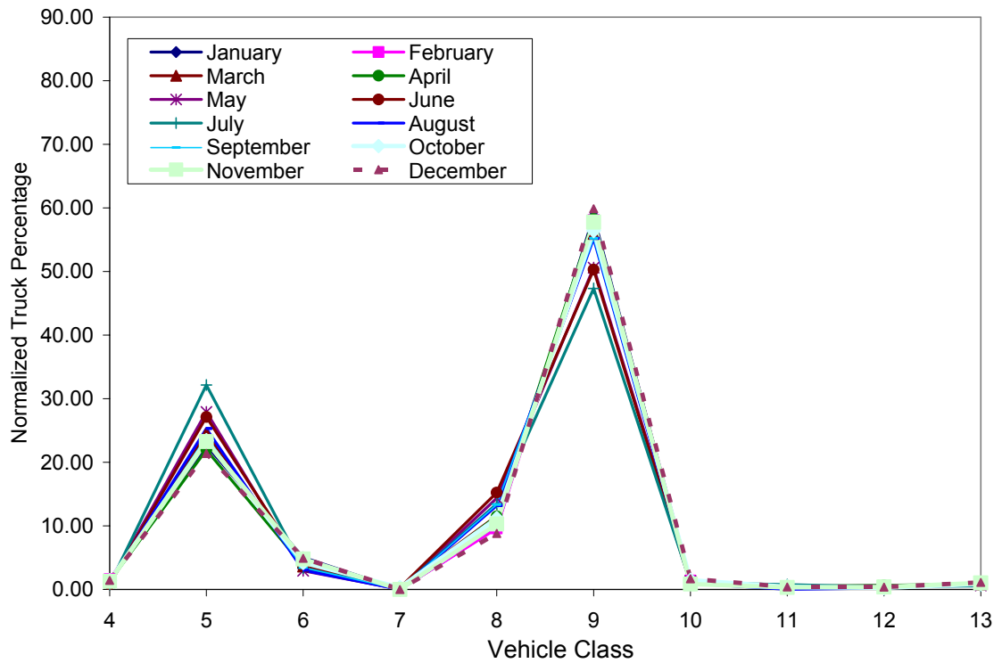
Figure 3.32 Monthly Truck Class Distribution for Site 3087
