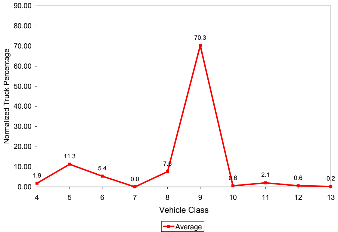
Figure 3.15 Vehicle Class Distribution for 3093
