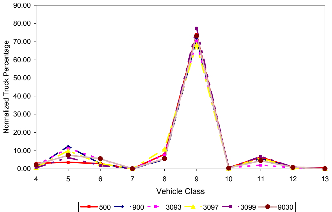
Figure 3.24 Vehicle Class Distribution for Functional Class 1
