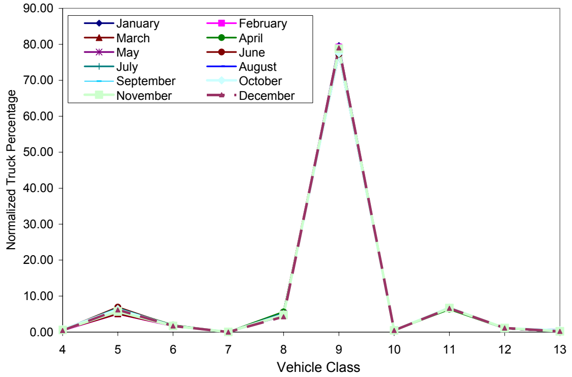
Figure 3.30 Monthly Truck Class Distribution for Site 3099
