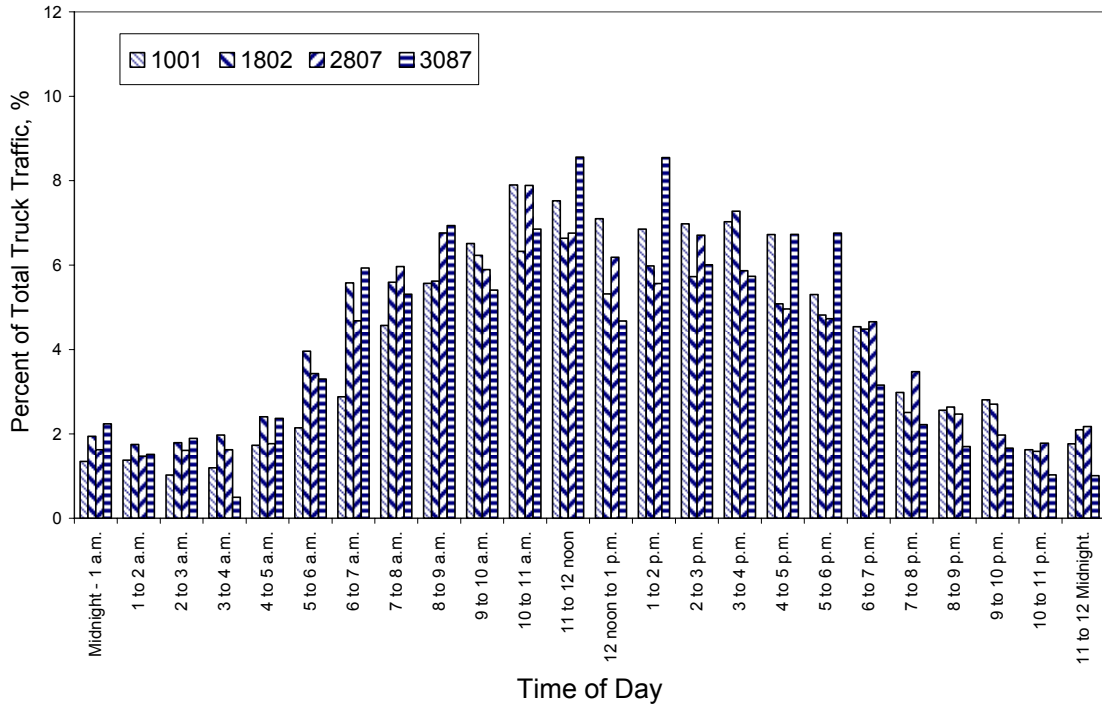
Figure 3.42 Hourly Truck Distribution for TTC 7
