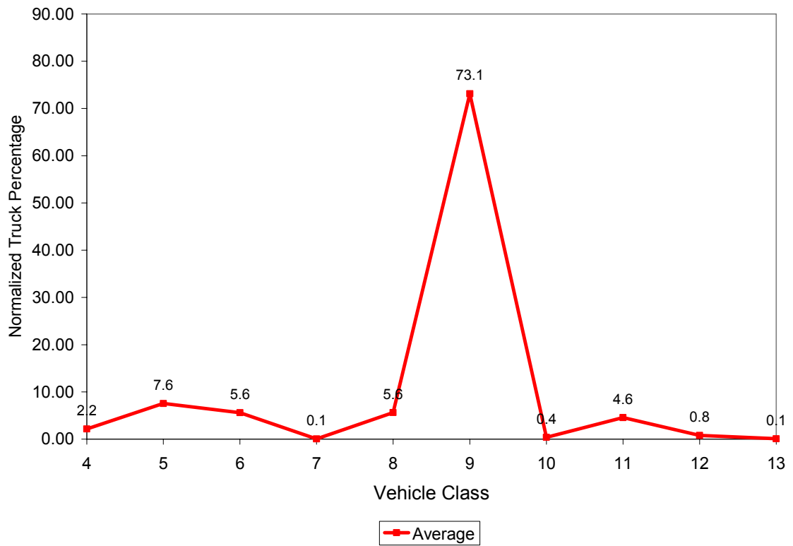
Figure 3.23 Vehicle Class Distribution for 9030
