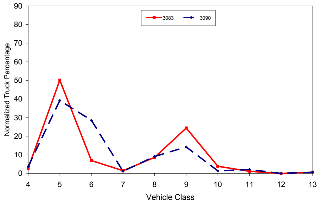
Figure 3.29 Vehicle Class Distribution for TTC 15
