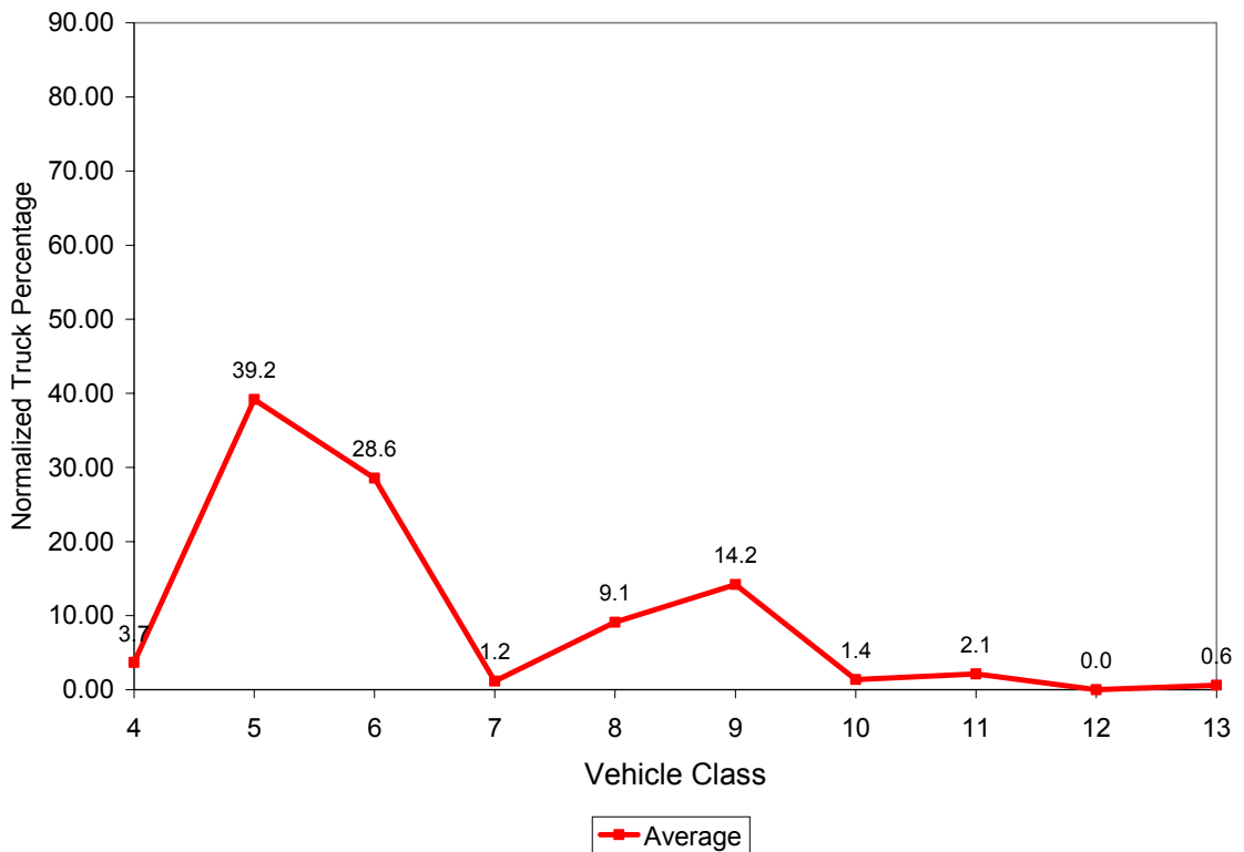
Figure 3.13 Vehicle Class Distribution for 3090
