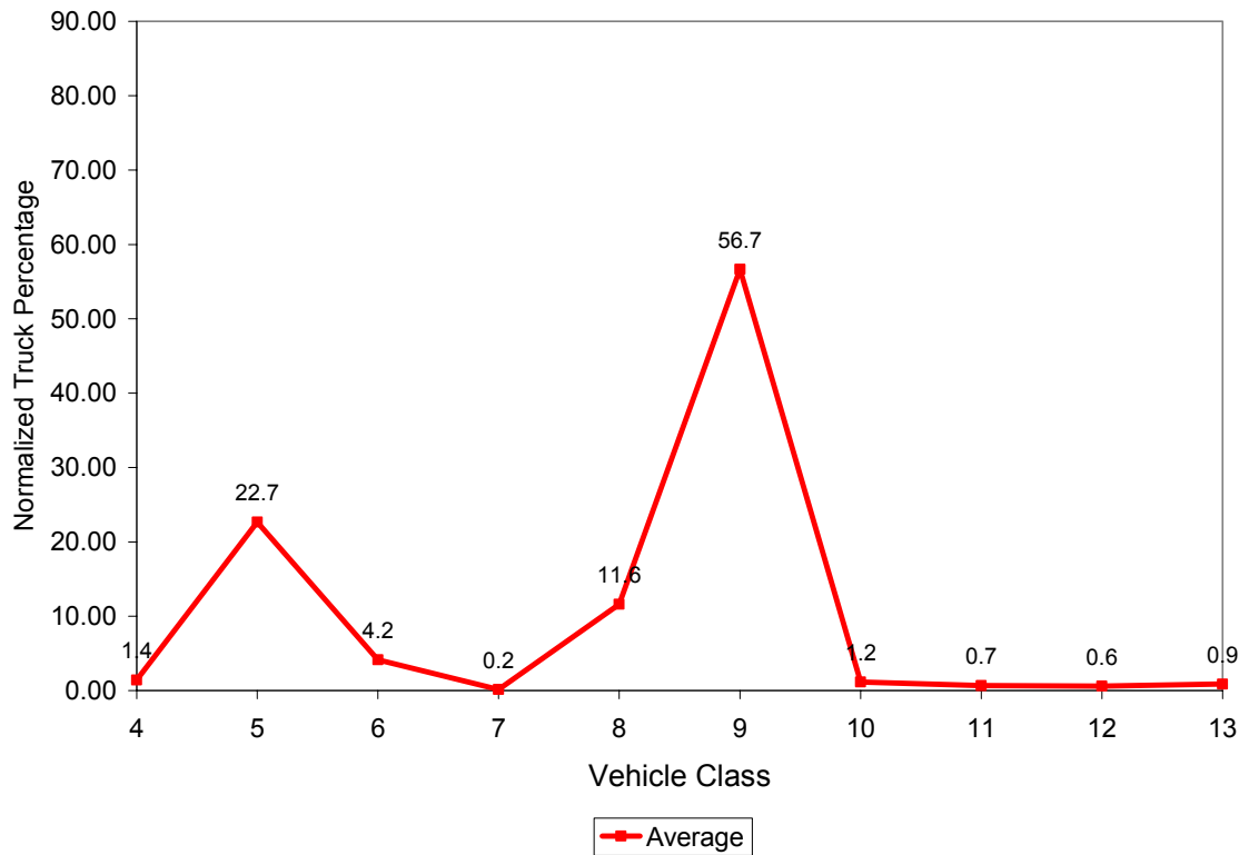
Figure 3.12 Vehicle Class Distribution for 3087
