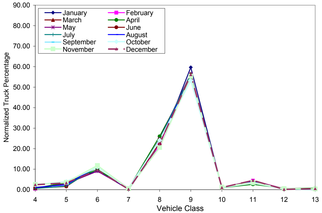
Figure 3.31 Monthly Truck Class Distribution for Site 1016
