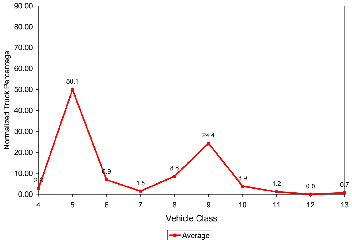
Figure 3.11 Vehicle Class Distribution for 3083
