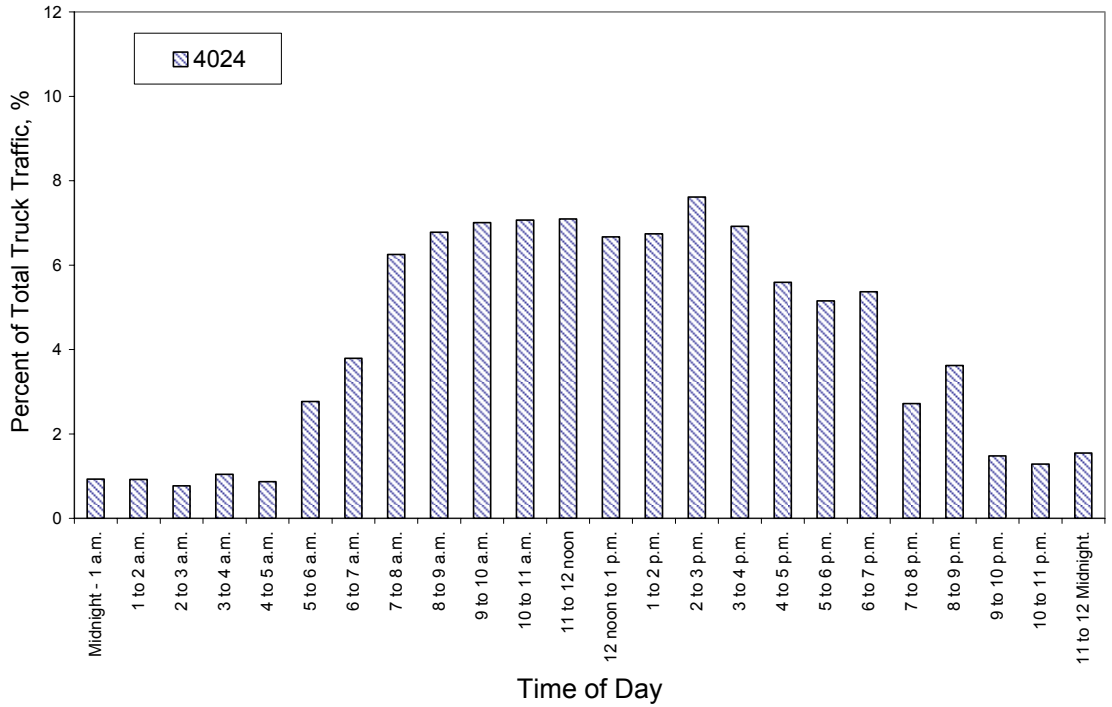
Figure 3.43 Hourly Truck Distribution for TTC 12
