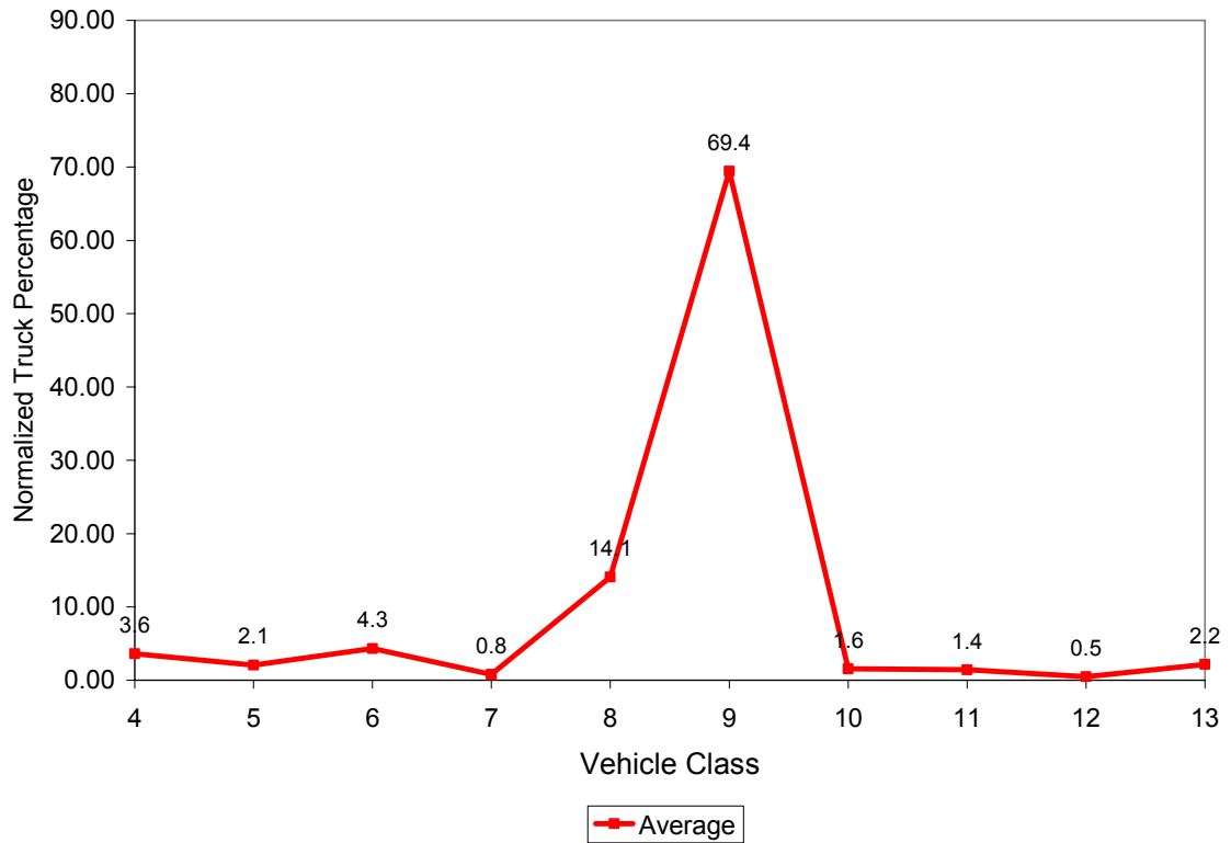
Figure 3.8 Vehicle Class Distribution for 3018
