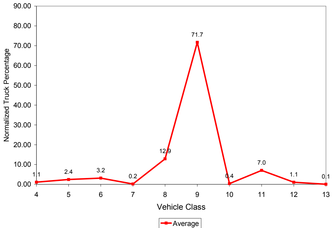
Figure 3.19 Vehicle Class Distribution for 5006
