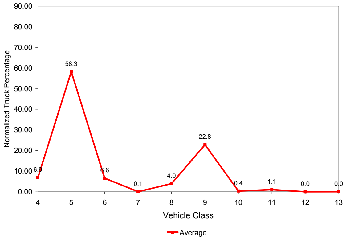
Figure 3.18 Vehicle Class Distribution for 4024
