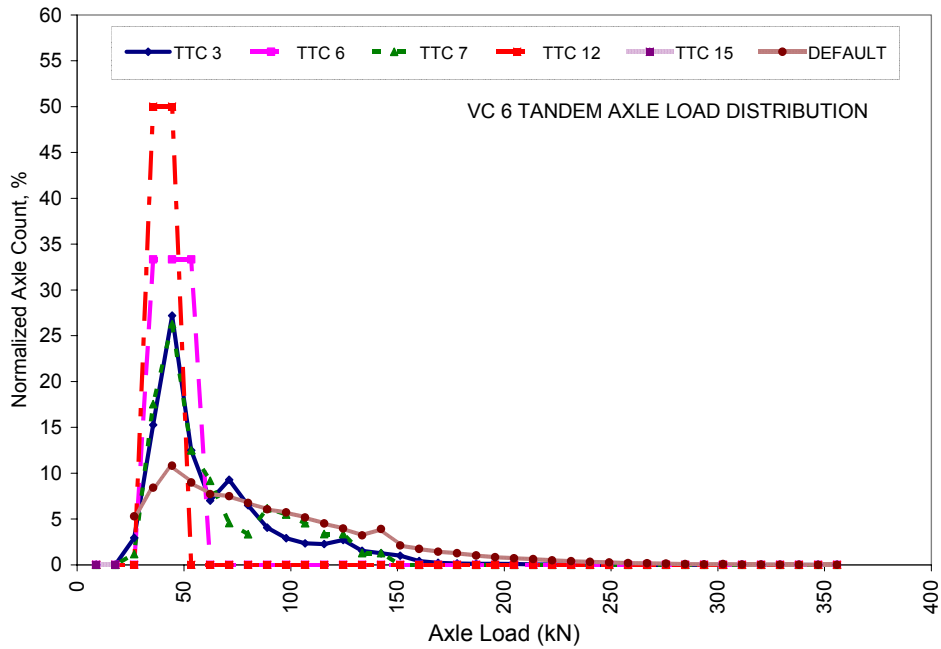
Figure 3.47 VC 6 Tandem Axle Load Spectra for TTC Groups
