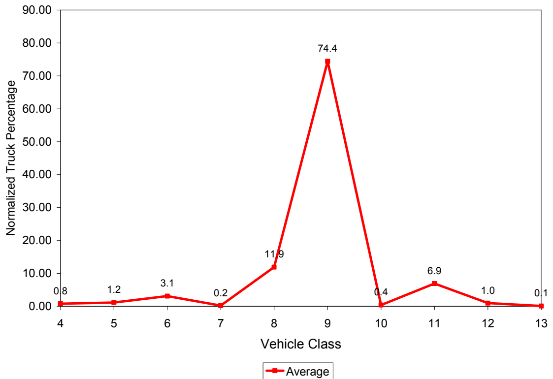
Figure 3.9 Vehicle Class Distribution for 3081
