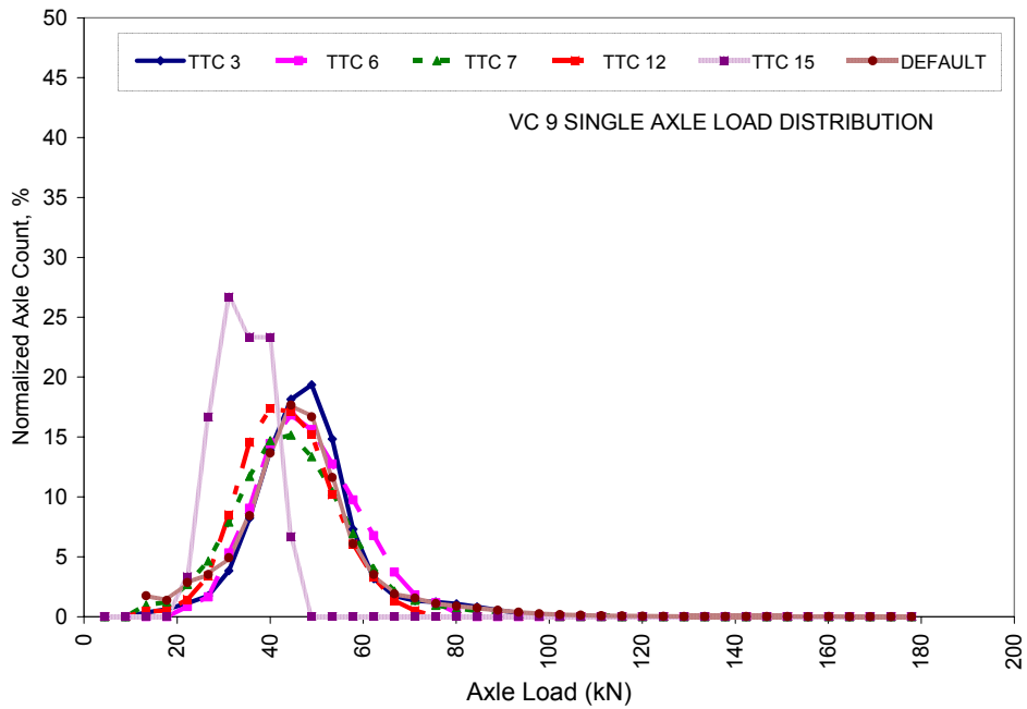
Figure 3.46 VC 9 Single Axle Load Spectra for TTC Groups
