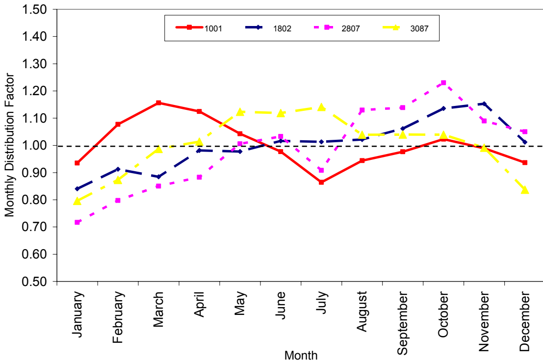
Figure 3.36 Monthly Distribution Factors for TTC 7
