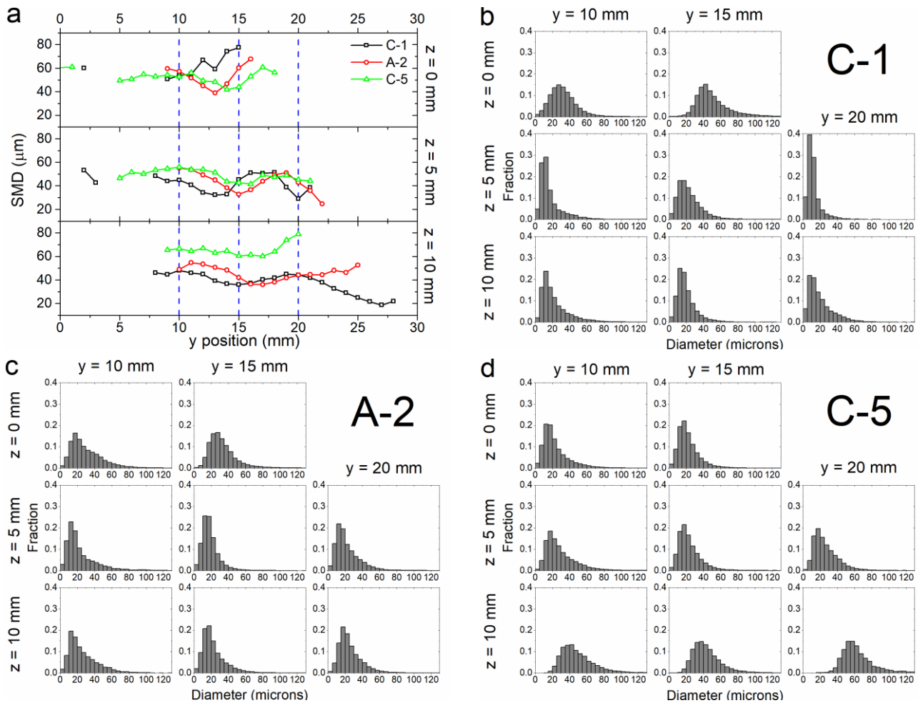
Figure 5 Sauter mean diameter and representative diameter histograms a) Sauter mean diameter plotted versus y position for each fuel 0 mm, 5 mm, and 10 mm downstream of the deflector plate for comparison with b) C-1 diameter histograms, c) A-2 diameter histograms, and d) C-5 diameter histograms.
