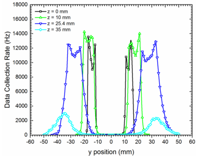
Figure 3 A-2 data collection rate. Data collection rate versus y-position at various axial locations for A-2 at \phi=0.096
