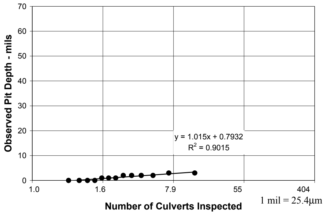
Figure 12. Extreme-value distribution with use of Potter's original data, low pitting mode.
