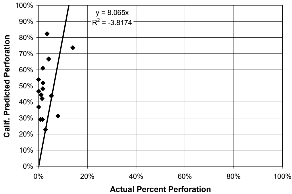
Figure 2. California Method curve prediction versus actual percent perforation, Aluminized Type 2 without outliers.
