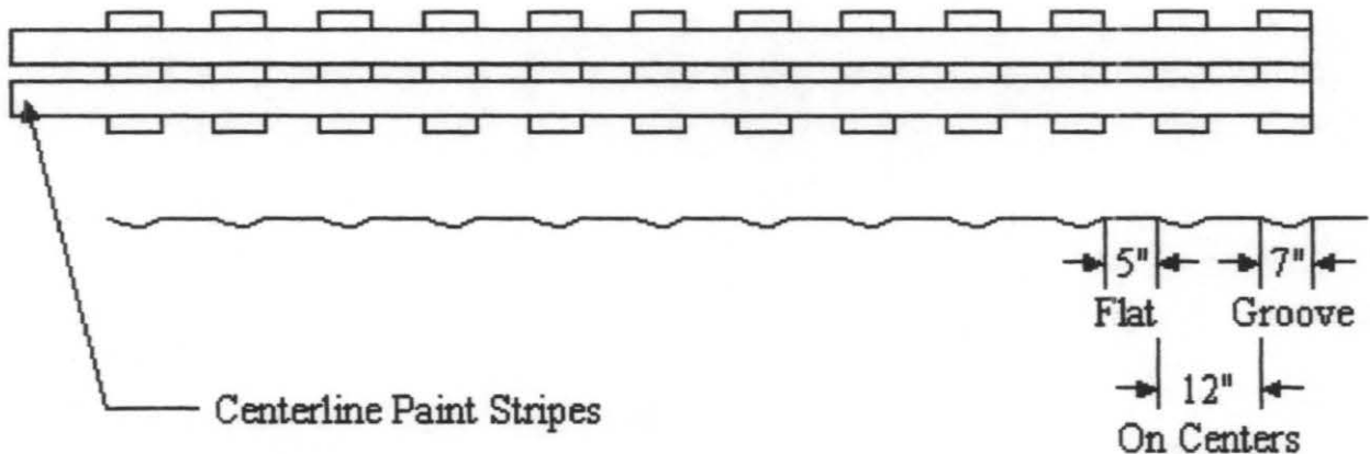
Figure 3. A drawing of the centerline rumble strips.
