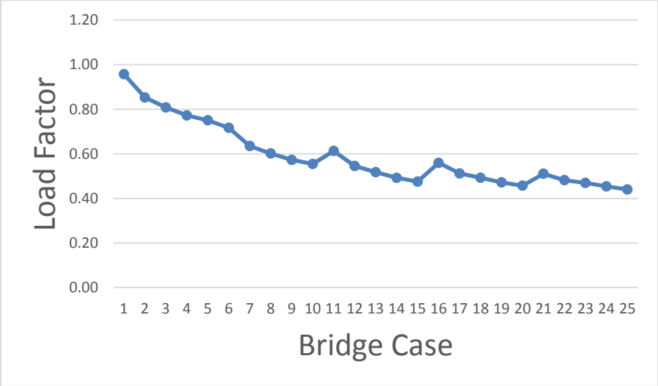
Figure K.1.22. Required Load Factors for RC, Simple Shear, Two Lane.
