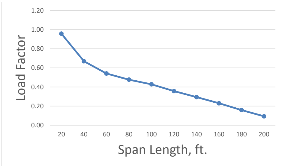
Figure K.1.46. Required Load Factors for 48" SBS Box, Simple Shear, Two Lane.
