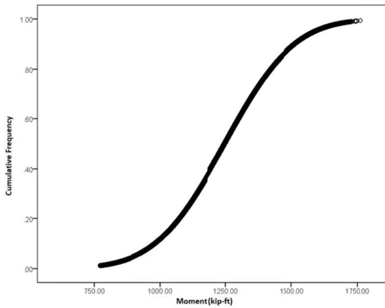
Figure H.26. CDF of Top 5% of Continuous 120 ft Span Moments, Single LEP Vehicles.
