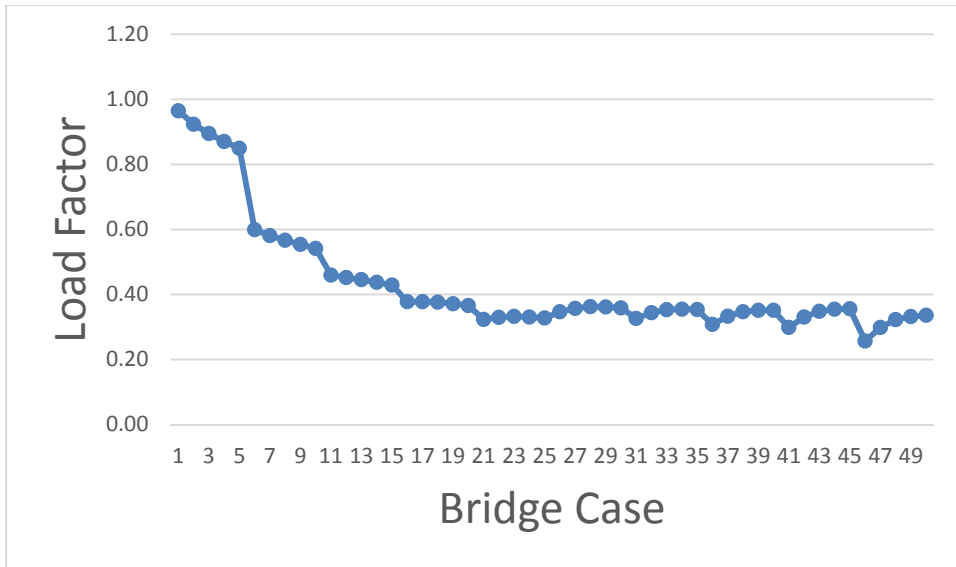
Figure K.1.25. Required Load Factors for Spread Box, Simple Moment, One Lane.
