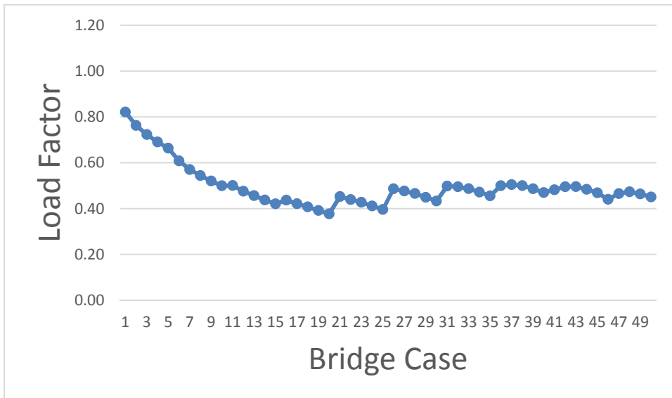
Figure K.1.26. Required Load Factors for Spread Box, Simple Shear, One Lane.
