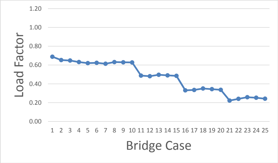
Figure K.1.23.1. Required Load Factors for RC, Continuous Negative Moment, Two Lane.
