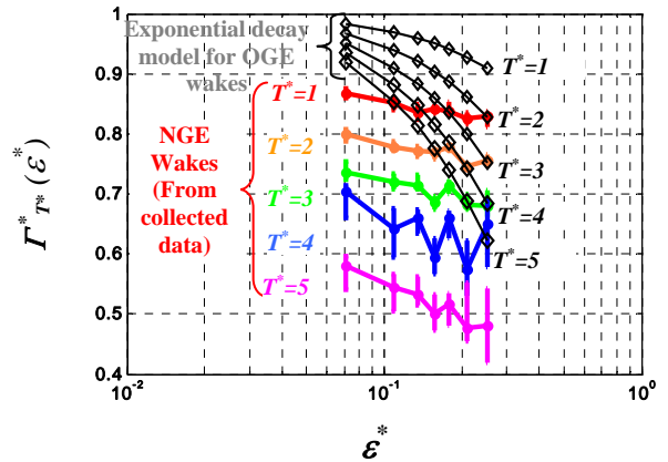
Figure 6: Dependence of Non-dimensional circulation I^{*T^*}(\varepsilon^*) on non-dimensional EDR ( \varepsilon^* ) for T^*=1,2,3,4 and 5 for wakes generated in NGE. These results are superimposed with the corresponding I^{*T^*}(\varepsilon^*) versus \varepsilon^* (in black) for the OGE exponential wake decay model.
