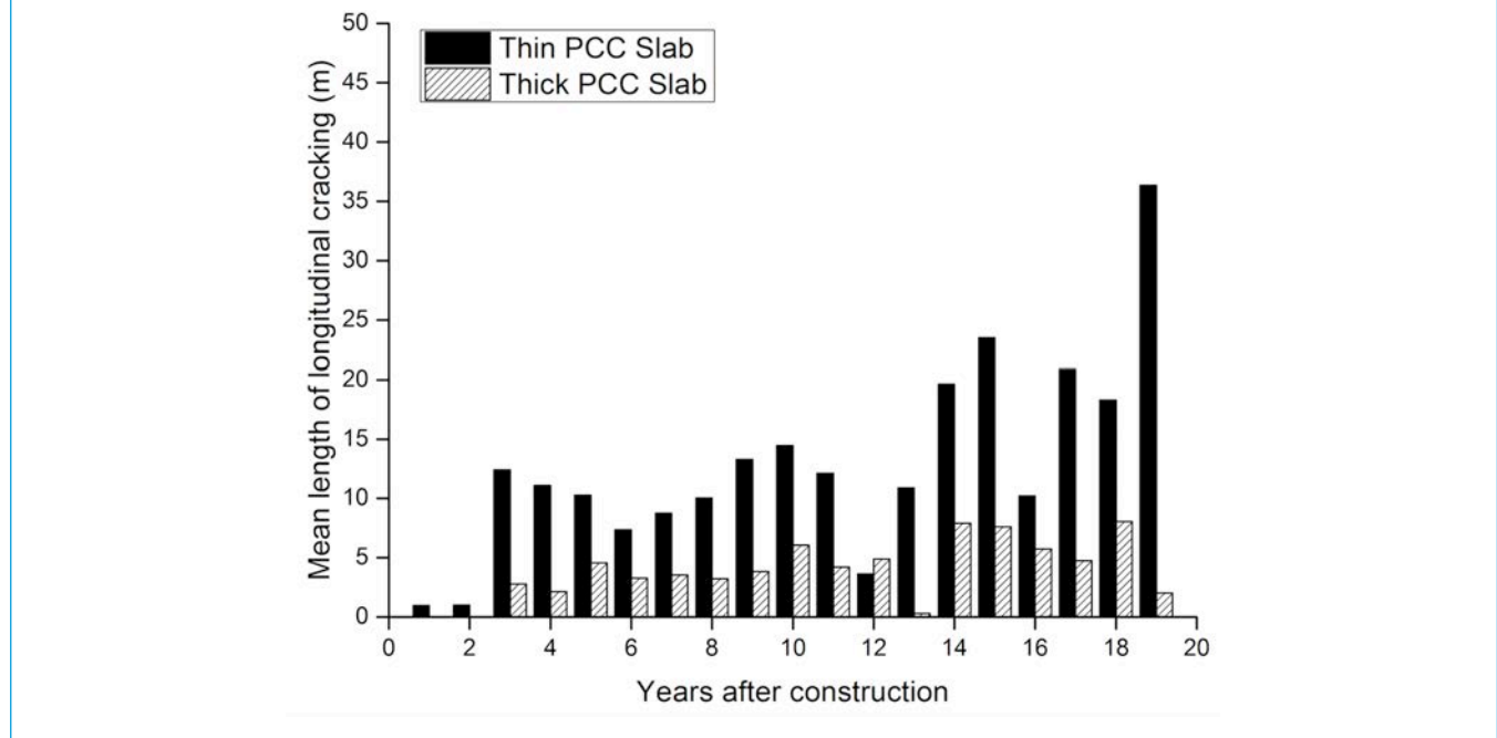
Figure 5. Mean longitudinal crack length per section over time for thin PCC slabs and thick PCC slabs.
