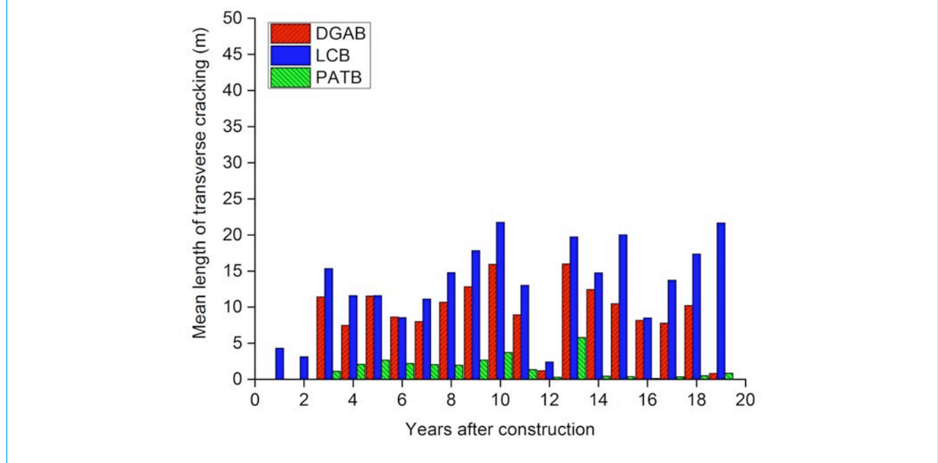
Figure 4. Mean transverse crack length per section over time for three different pavement base types.
