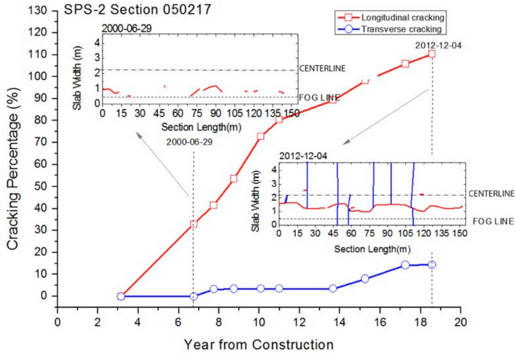
Figure 19. The development of cracking in Arkansas-0217 section.
