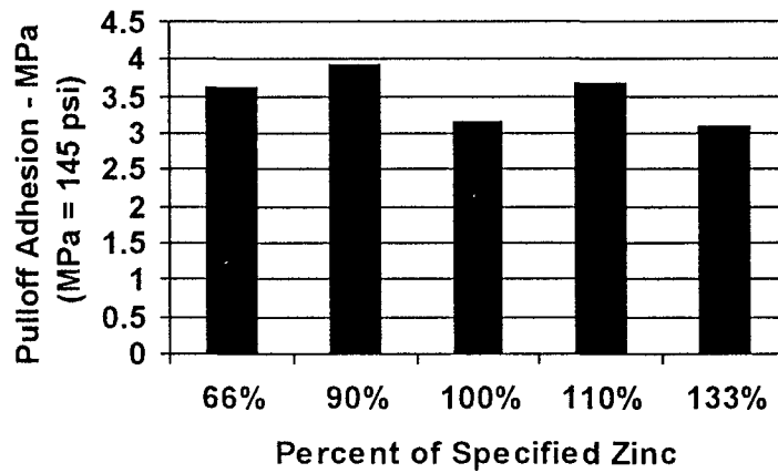
Figure 12. Acrylic topcoat adhesion over films with varying zinc content.
