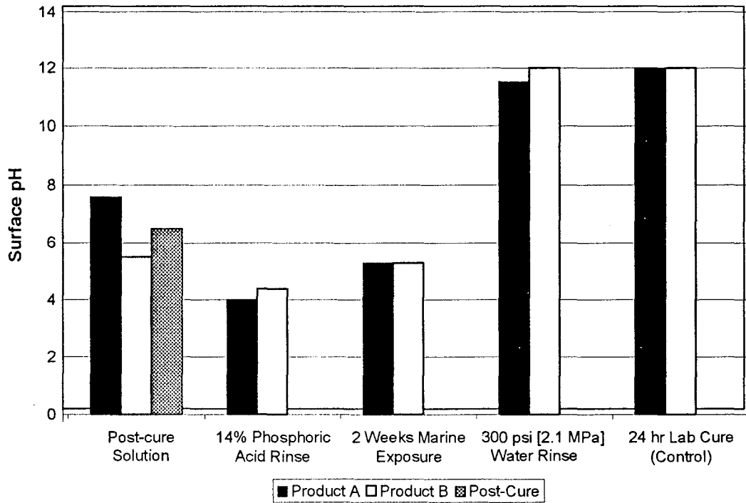
Figure 14. Surface pH measured after various primer treatments.
