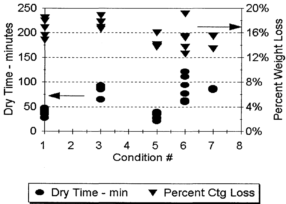
Figure 8. Drying data for the various conditions studied.
