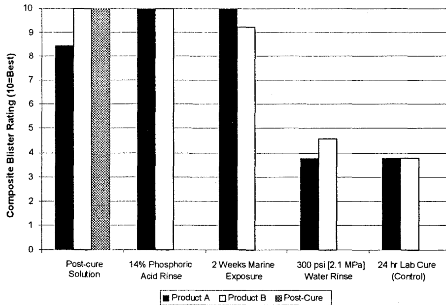
Figure 15. Composite blister ratings after 2-day marine atmosphere exposure.
