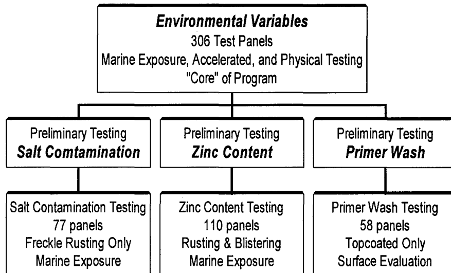
Figure 5. Outline of testing conducted.
