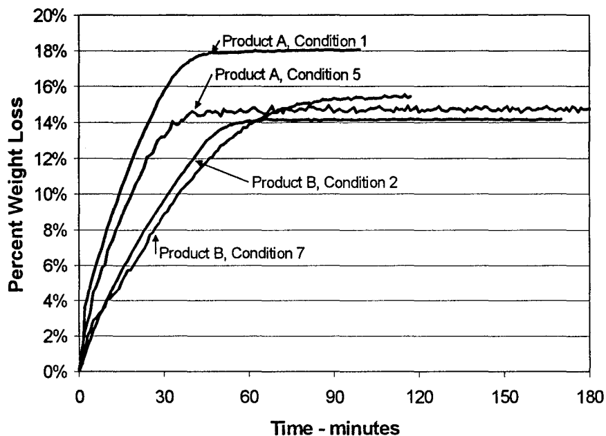
Figure 6. Typical drying curves for WBIOZ primer.
