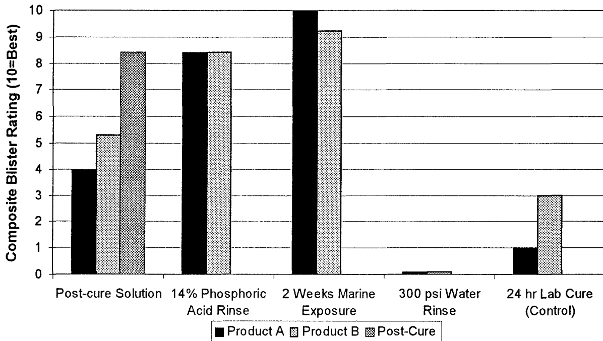
Figure 16. Composite blister ratings after 8-day condensing humidity exposure.
