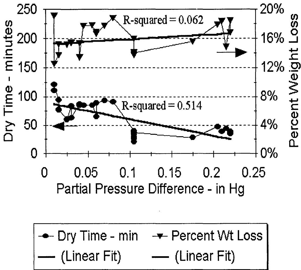
Figure 9. Drying characteristics as a function of actual partial pressure difference.
