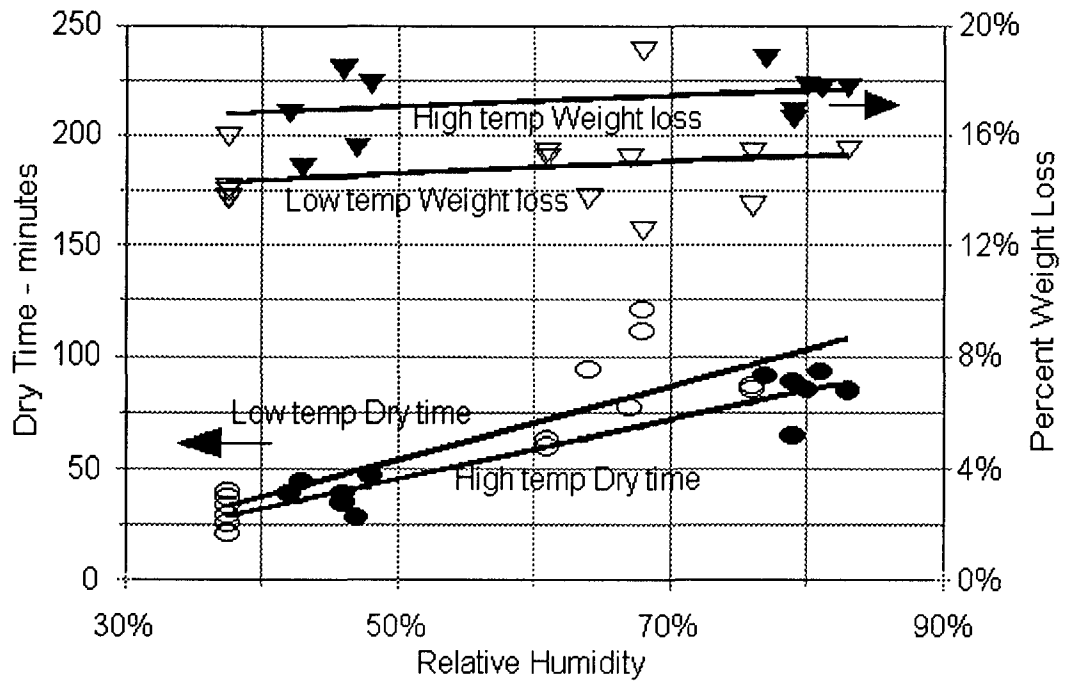
Figure 7. Drying characteristics as a function of target temperature and relative humidity.
