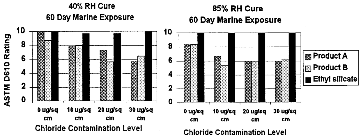
Figure 11. Freckle rusting as a function of surface chloride contamination and relative humidity.
