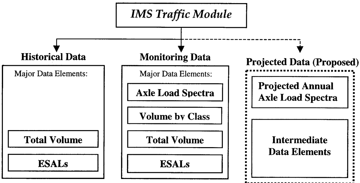
Figure 88. Overview of the IMS Traffic Module showing the proposed addition of projected data.
