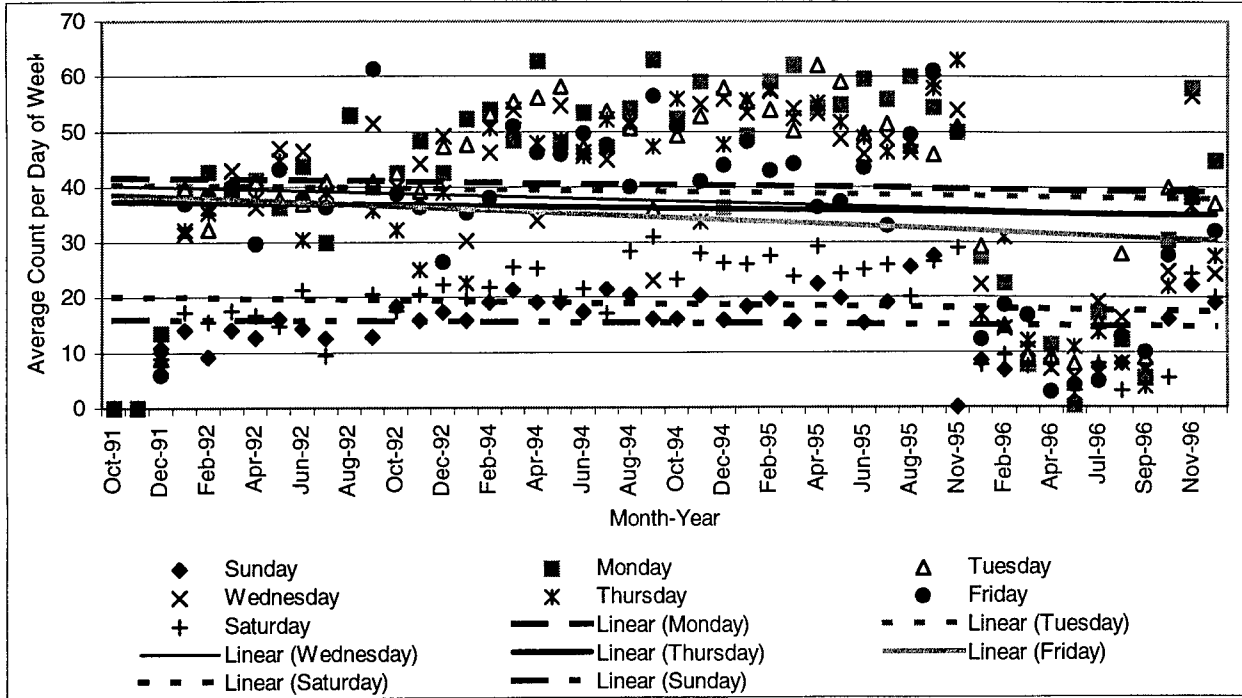
Figure 5. Axle load distributions by day of the week for Class 9 vehicles for Site 12-4000 – tandem-axle loads, 0-142.4 kN (0-31,999 lb), 1991 to 1996.
