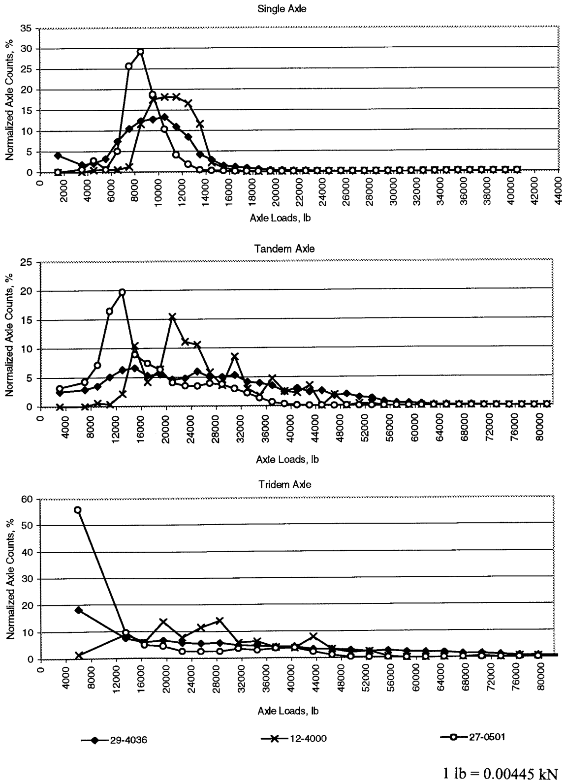
Figure 116. Normalized load spectra for Class 10 vehicles.
