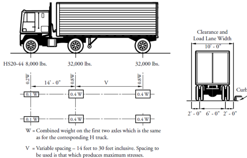
Figure 7-10. AASHTO HS20-44 Truck (Precast/Prestressed Concrete Institute, 2003) An influence line analysis was conducted to determine the location of the truck that resulted in the maximum moment demand on the bridge spans. This location was determined to be when the front axle
