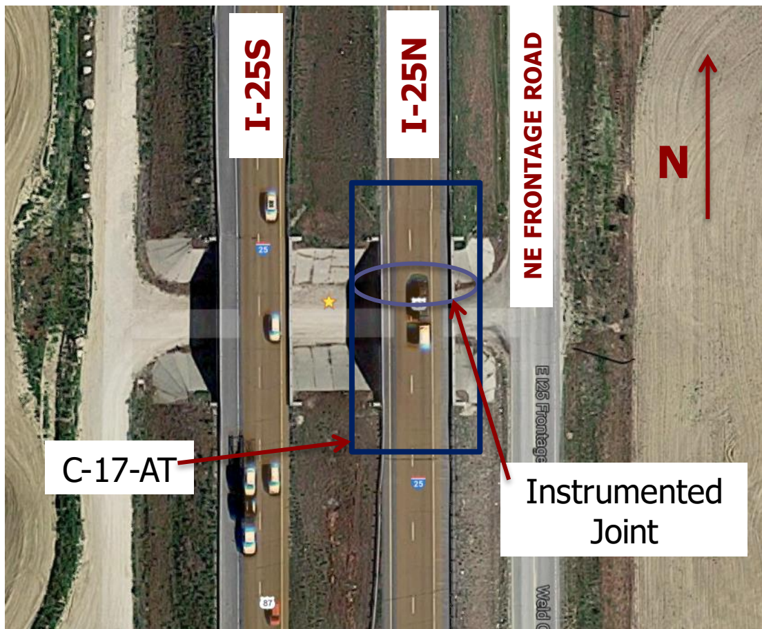
Figure 3-8 C-17-AT Overview
