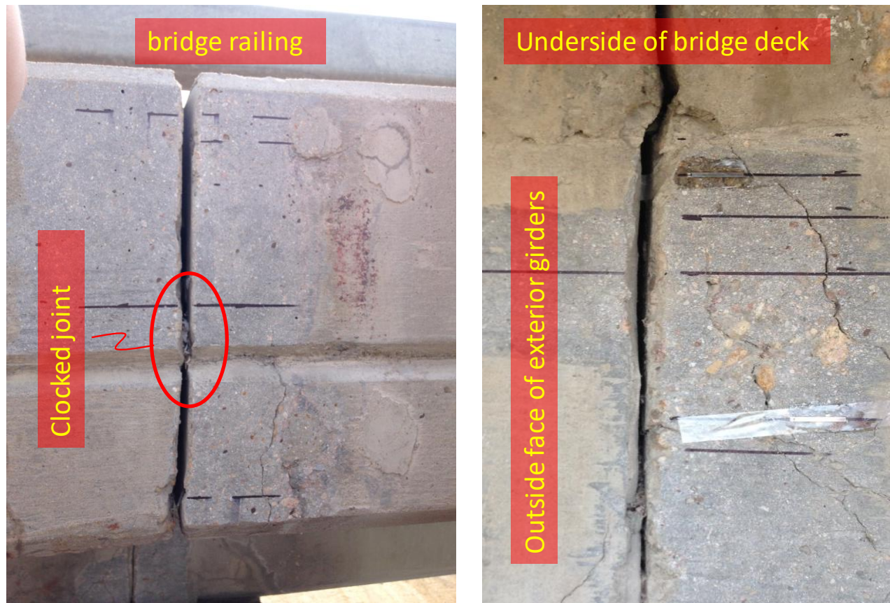
Figure 3-11 C-17-AT Expansion Joint Clogging
