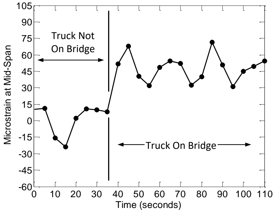
Figure 4-4. Field Control Load Test with Front Axle of A-40 Truck at Mid-Span
