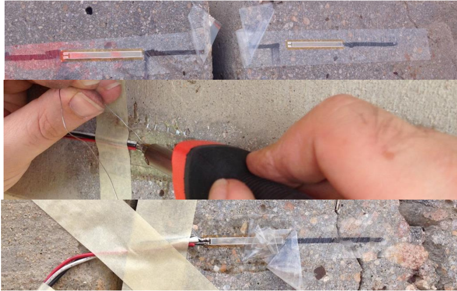
Figure 3-15 Strain Gage Application
