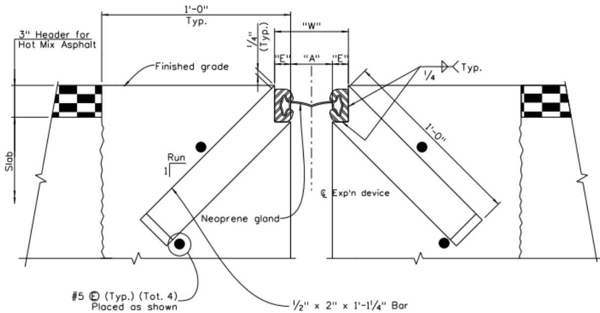
Figure 2-10 Section Thru Strip Seal Bridge Expansion Device (CDOT, 2015)
