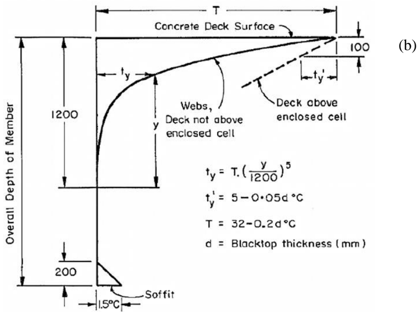
Figure 6-3 (a) AASHTO Thermal Gradient, (b) New Zealand Thermal Gradient.
