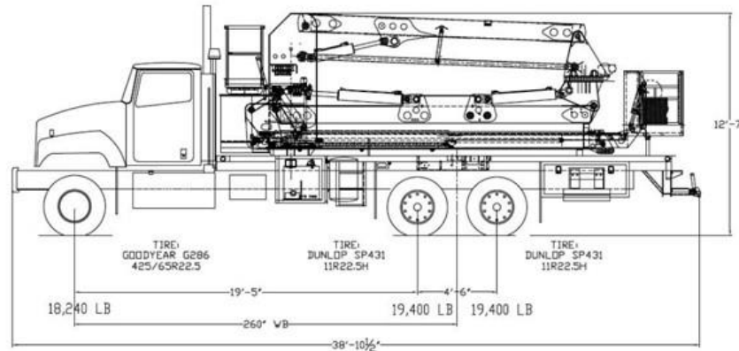
Figure 4-1 Aspen Aerials A-40 Truck with Dimensions and Axel Weights
