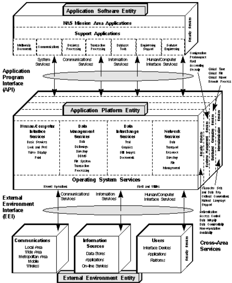
FIGURE 2. NAS OSE reference model
