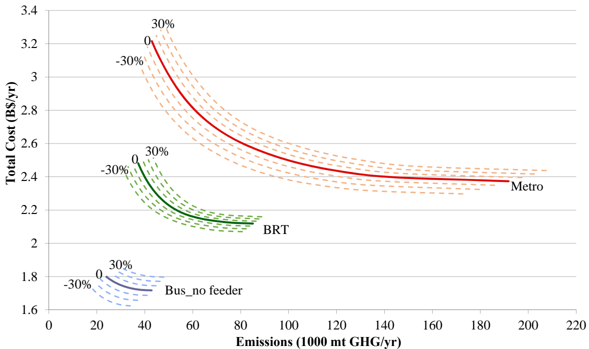
Figure 4.15 Sensitivity to changes in parameters for metro, BRT and trunk-only bus (scenario 2)
