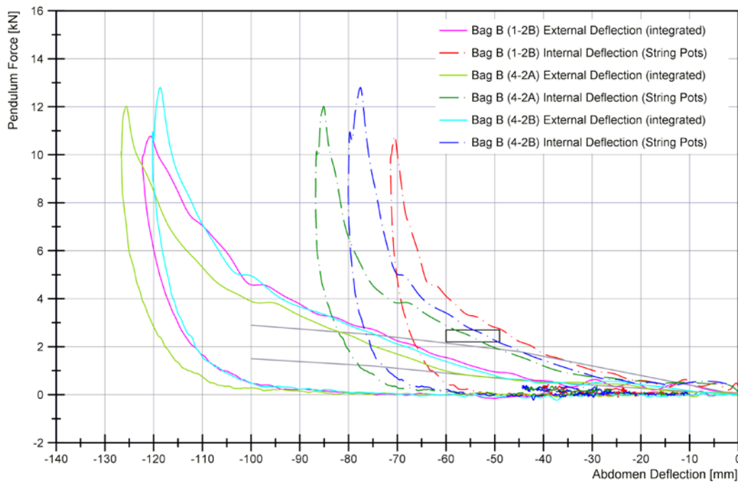
Figure 11. Repeatability of lower abdomen deflection measurements – internal and external force-deflection
