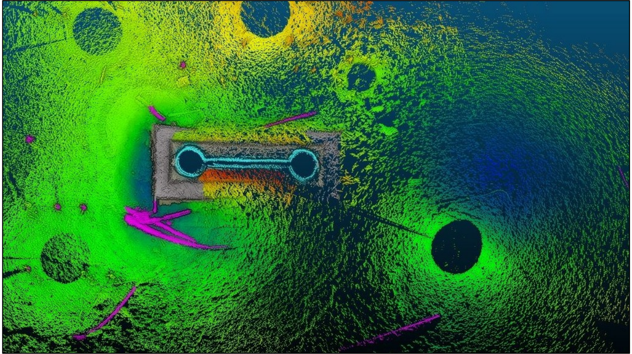
Figure 3-3: Bridge 4654 Pier 8 Colorized Point Cloud Plan View
