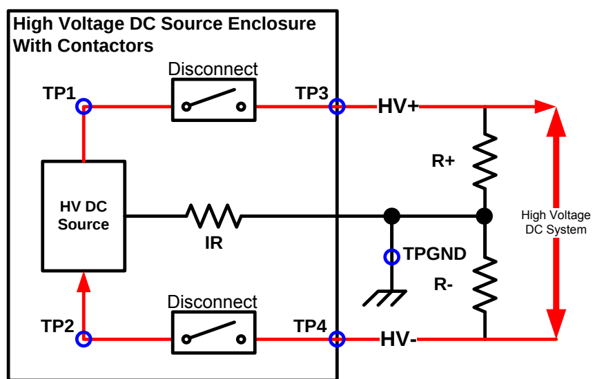
Figure 12. Test points for source with disconnects.
