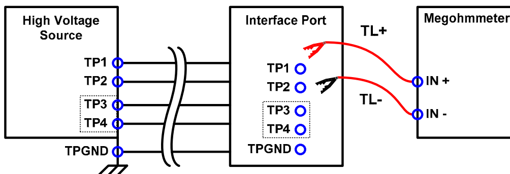
Figure 4. Overview of the test setup for one high-voltage source.
