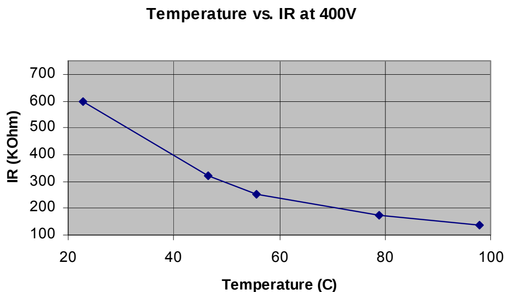
Figure 20. Glystantin megohmmeter results at increasing temperatures.
