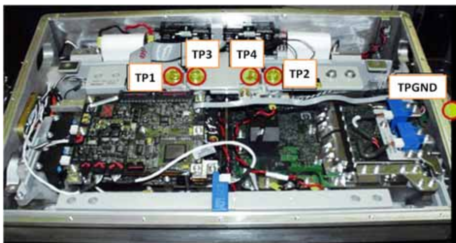
Figure 13. GM Chevrolet Equinox test point locations.
