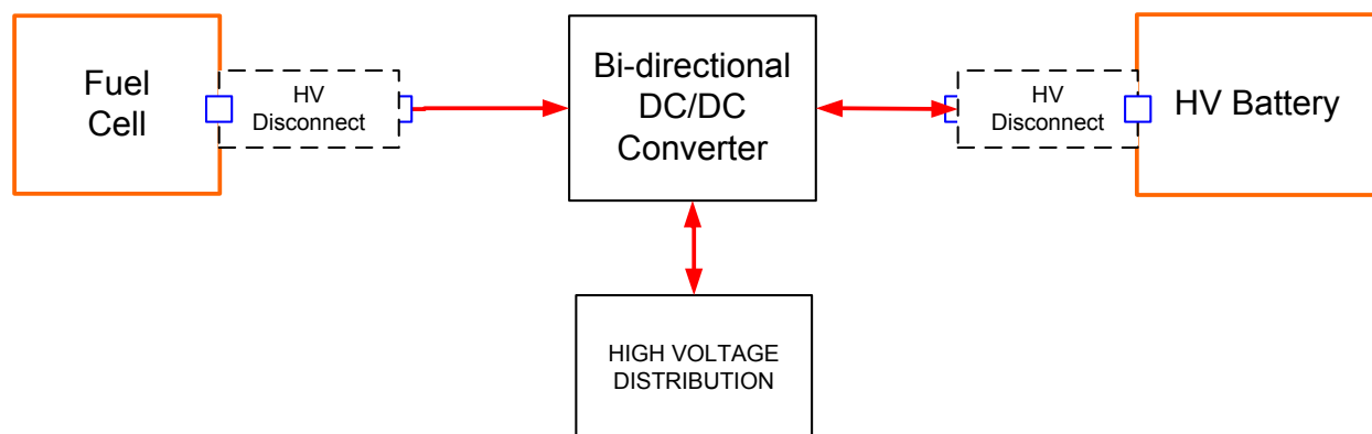
Figure 9. Simplified HFCV power system diagram.
