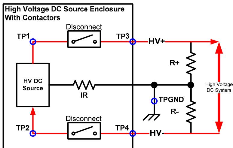
Figure 3. High-voltage source with marked test points having direct access to the high-voltage terminals.
