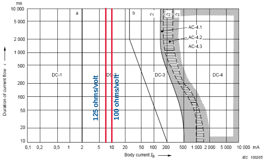
Figure 2. Conventional time/current zones of effects of DC currents on persons for a longitudinal upward current path (IEC TS 60479-1: 2005-07) with 100 ohms/volt and 125 ohms/volt references added.
