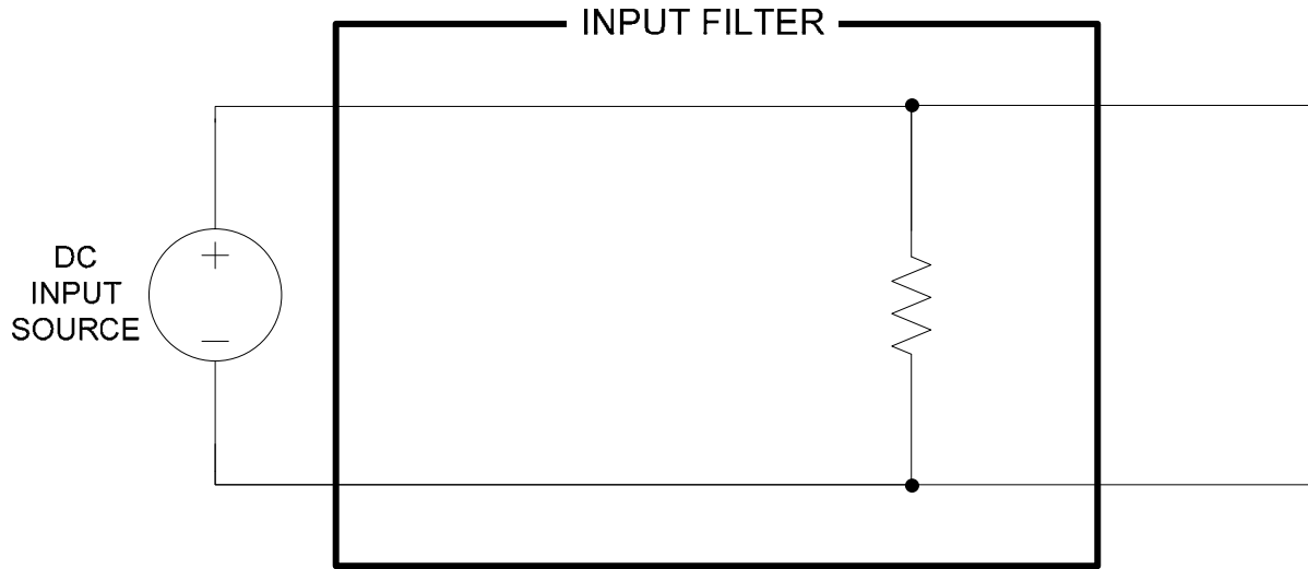
Figure 16. Input power filter DC equivalent circuit.
