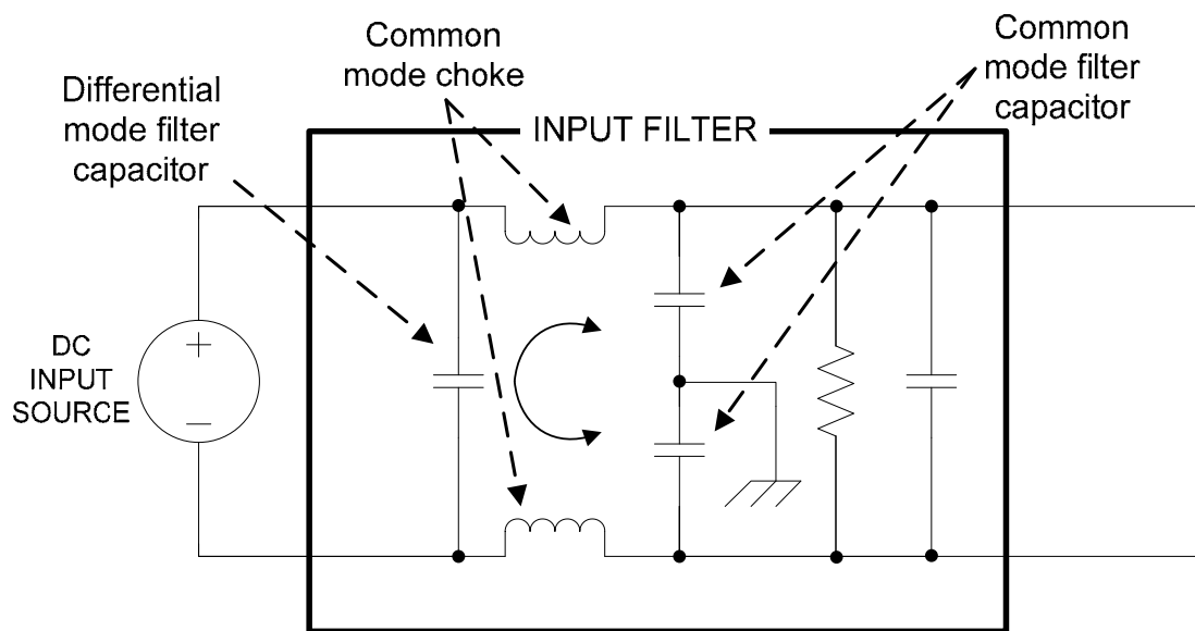
Figure 15. Input power filter.
