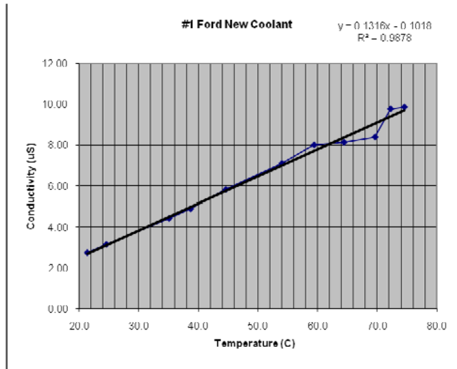
Figure 21. New Glystantin sample from Ford results at increasing temperatures.
