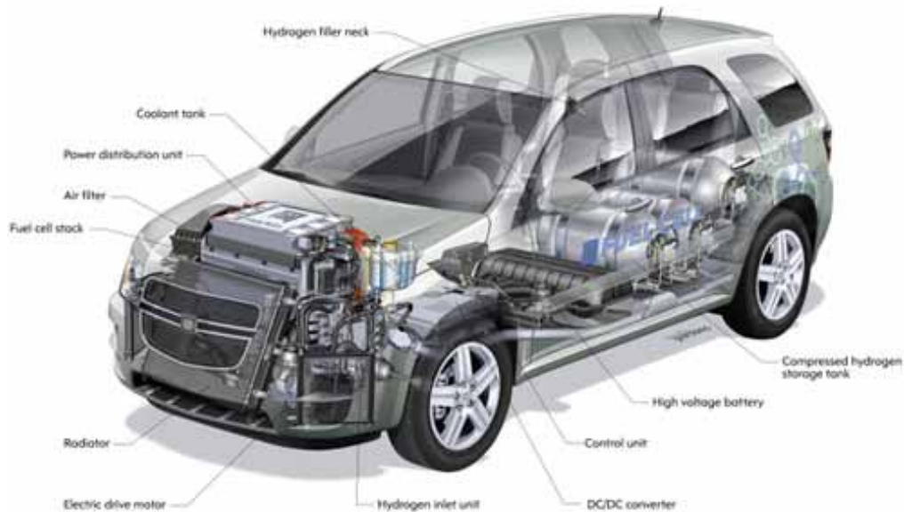
Figure 4. Photograph of the 2009 Chevrolet Equinox HFCV provided by GMC.
