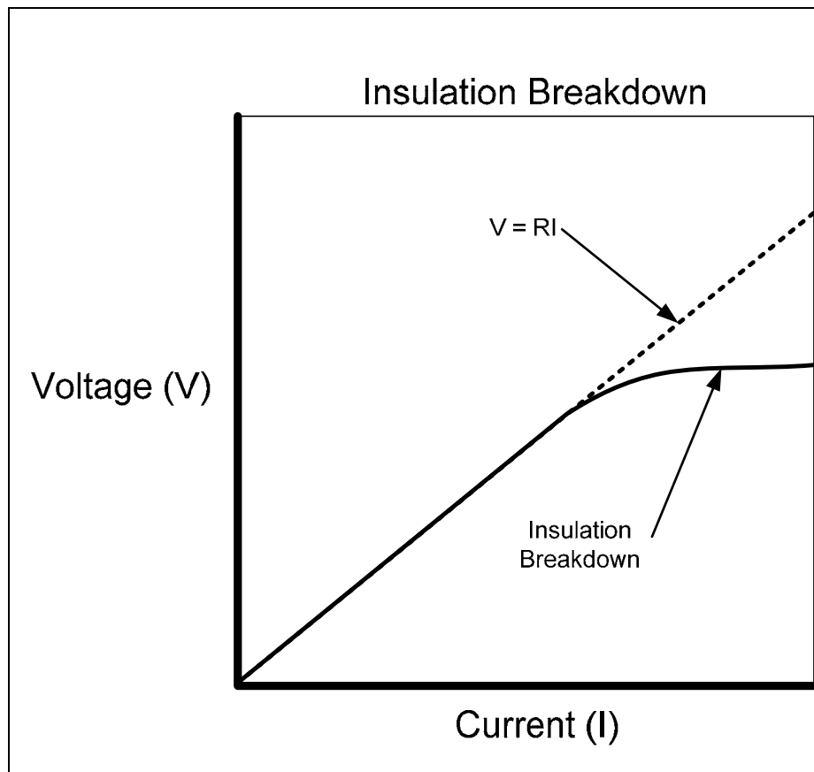
Figure 5. Insulation breakdown.
