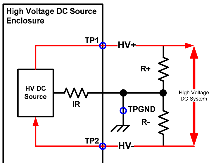
Figure 11. Test points for source without disconnects.
