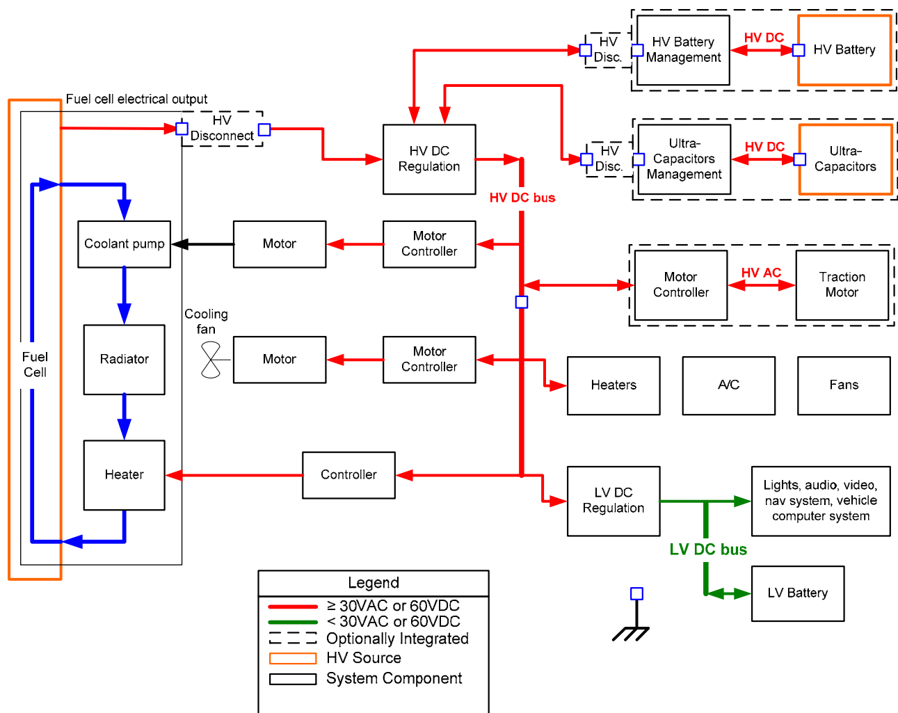
Figure 8. General block diagram for an HFCV with test points and disconnects.
