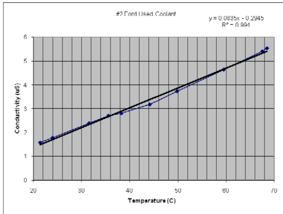
Figure 22. Aged Glystantin sample from Ford results at increasing temperatures.
