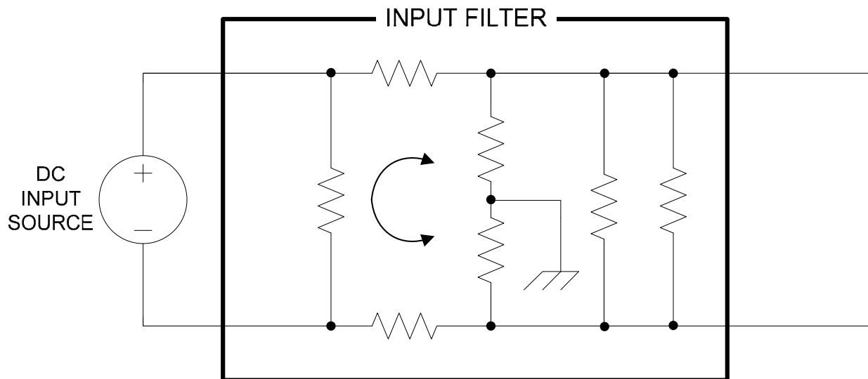
Figure 17. Input power filter AC equivalent circuit.
