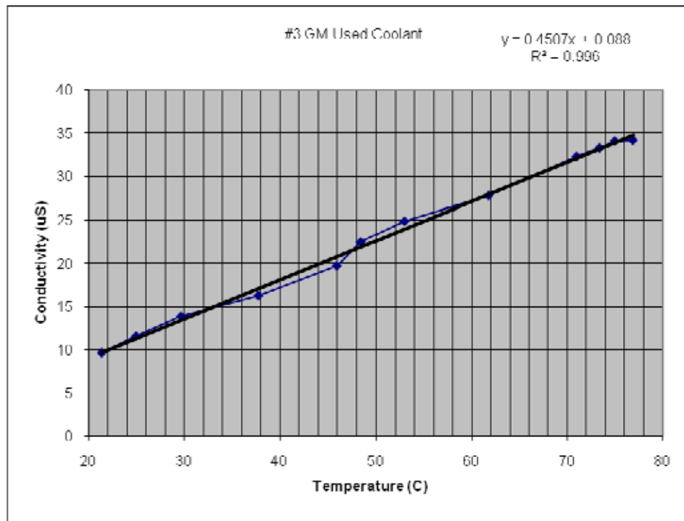
Figure 23. Aged Glystantin sample from General Motors results at increasing temperatures.
