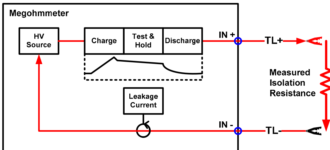
Figure 1. Diagram of a megohmmeter with positive and negative test leads, TL+ and TL-, respectively.
