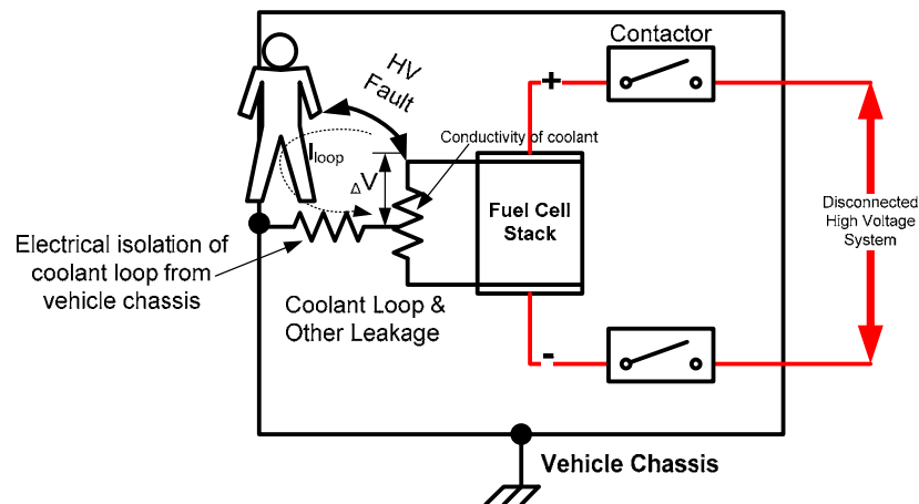
Figure 10. Potential shock hazard from fuel cell and coolant loop.
