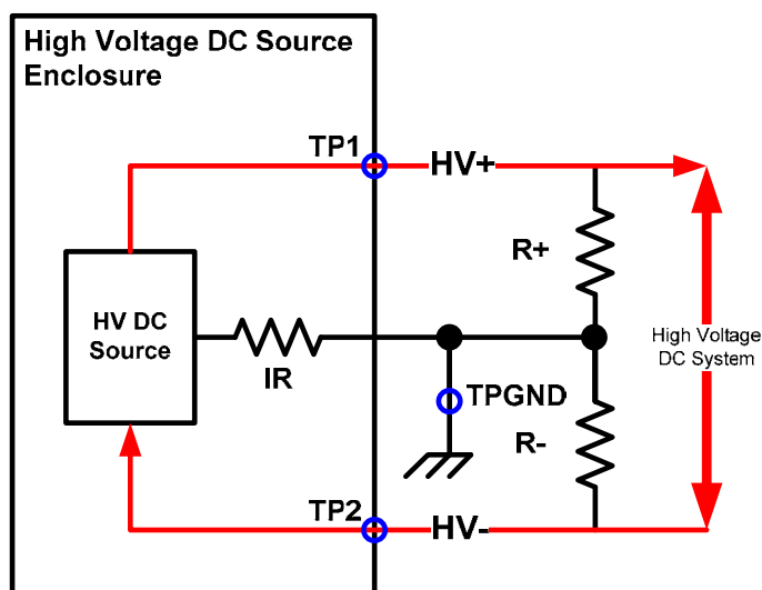
Figure 2. High-voltage source with marked test points providing direct access to the high-voltage terminals.
