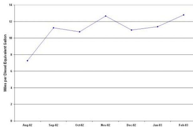
Figure 3. ThunderPower Bus Fuel Economy by Month
