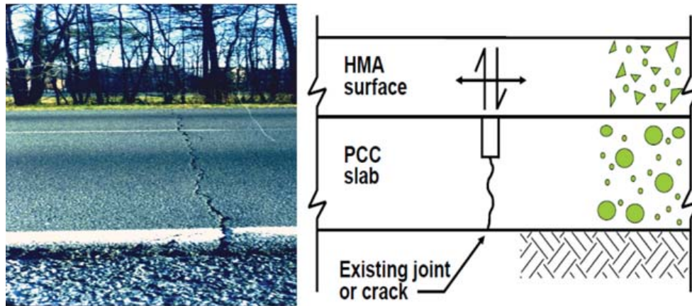
Figure 1 Reflective cracking
