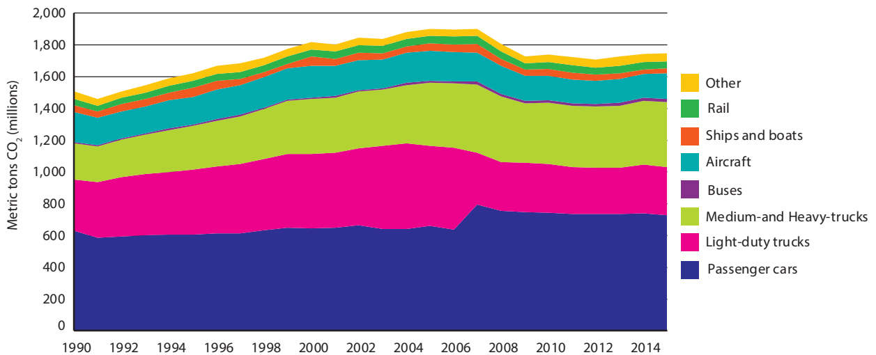
FIGURE 7-5 CO 2 Greenhouse Gas Emissions by Mode: 1990–2015
