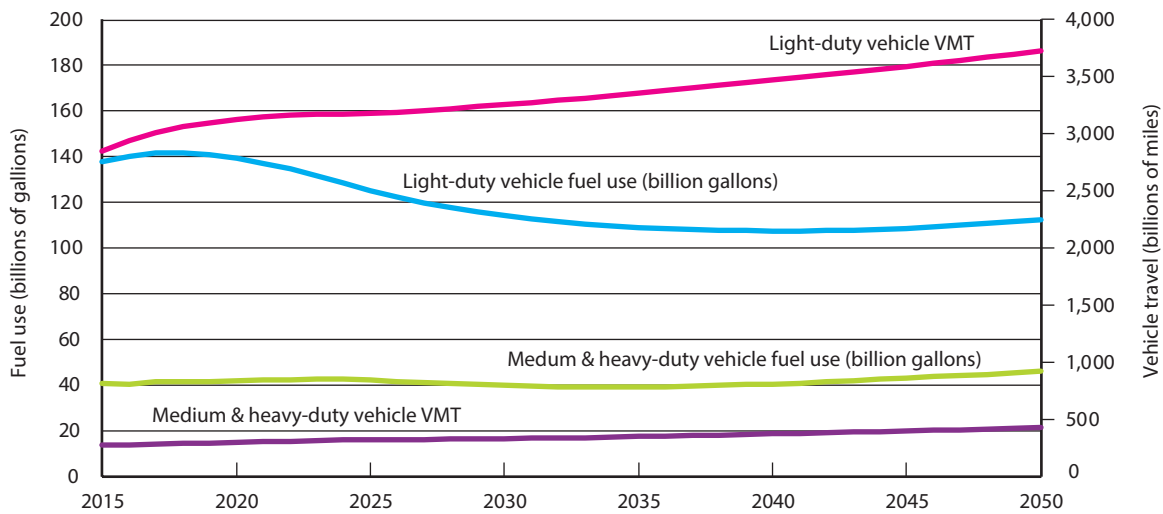
FIGURE 7-14 Highway Vehicle Fuel Use and Travel: 2015 Projected to 2050
