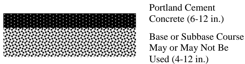
Fig. 5.5 Typical Cross Section of a Rigid Pavement
