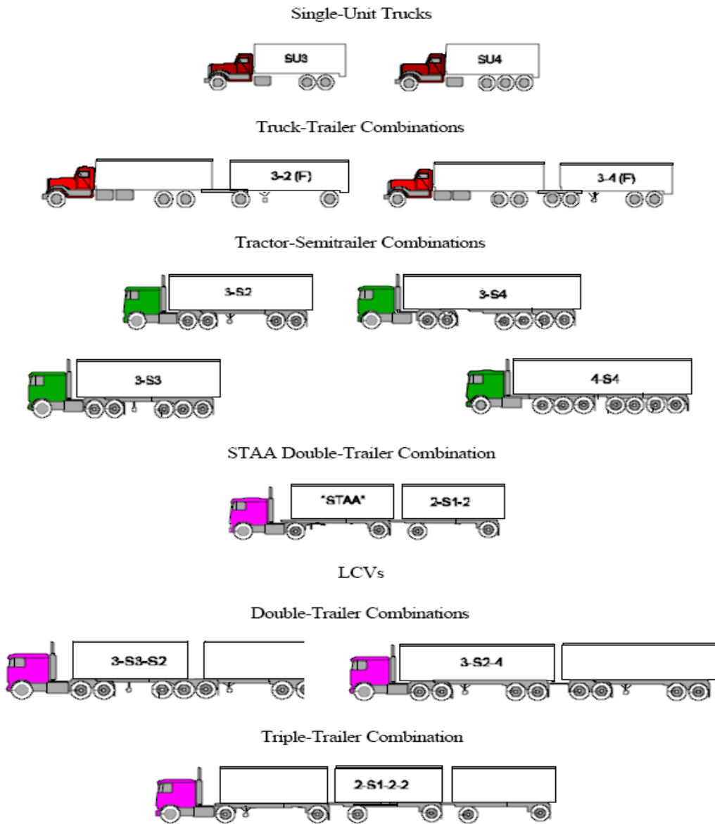
Fig. 5.1 Illustrative Truck Fleet Configuration
