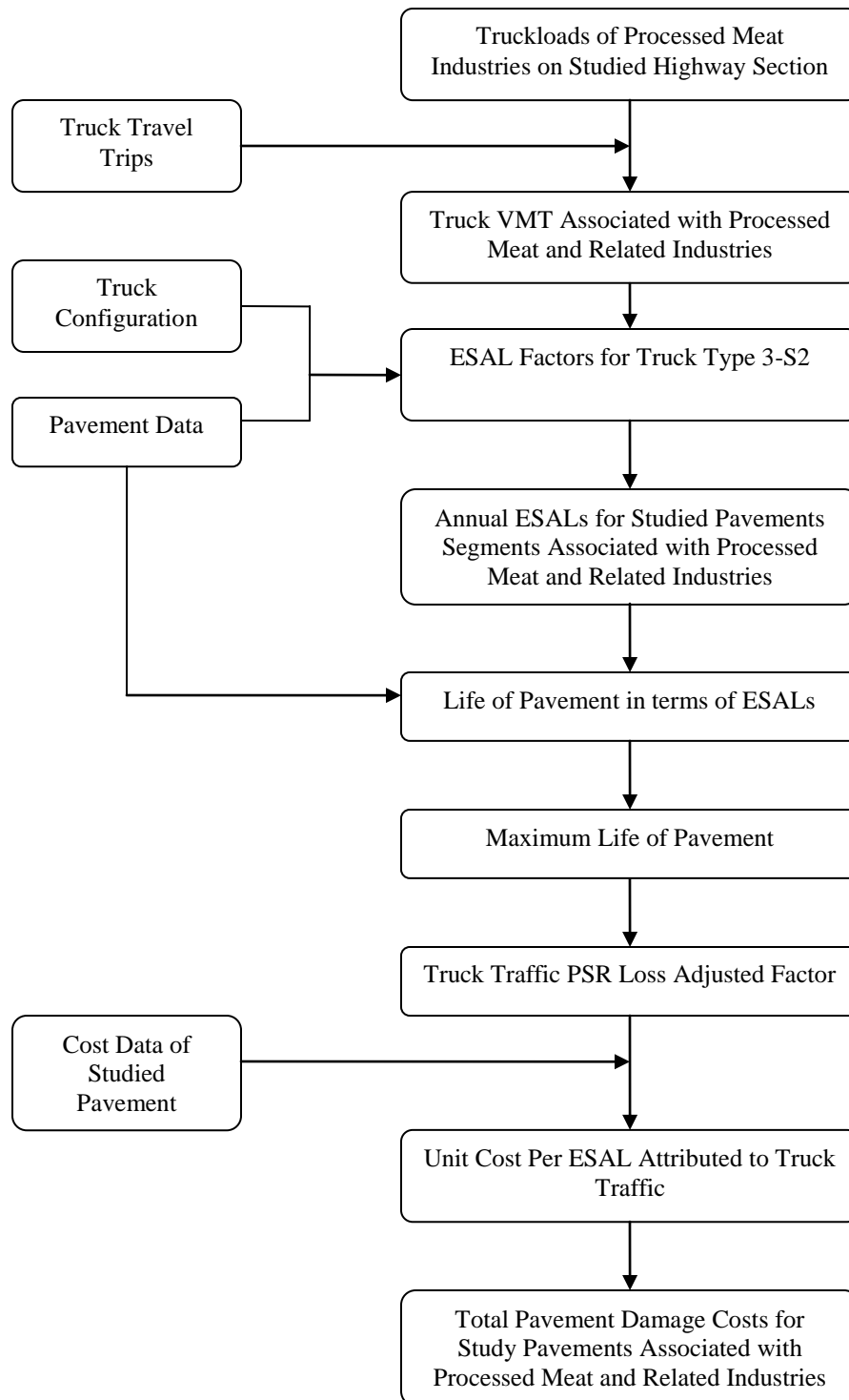
Fig. 3.2 Flowchart of Pavement Damage Cost Analysis Procedure
