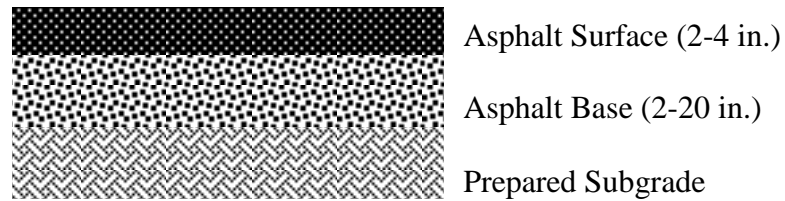
Fig. 5.4 Typical Cross Section of a Full-Depth Asphalt Pavement
