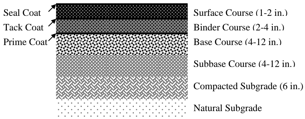
Fig. 5.3 Typical Cross Section of a Conventional Flexible Pavement
