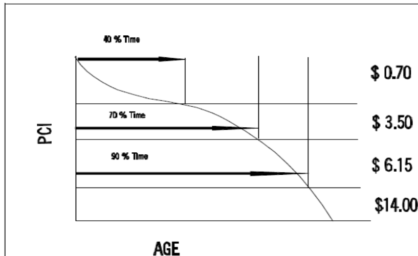
Fig. 2.3 Effect of Treatment Timing on Repair Costs (AASHTO, 2001)
