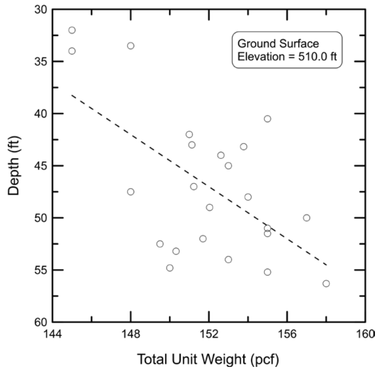
Figure H.5 Total unit weight profile.
