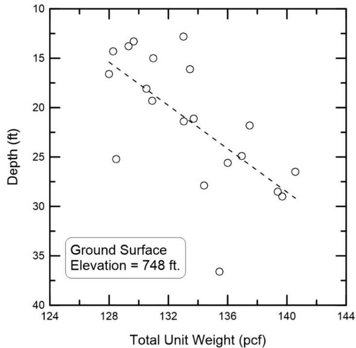
Figure A.4 Total unit weight profile.
