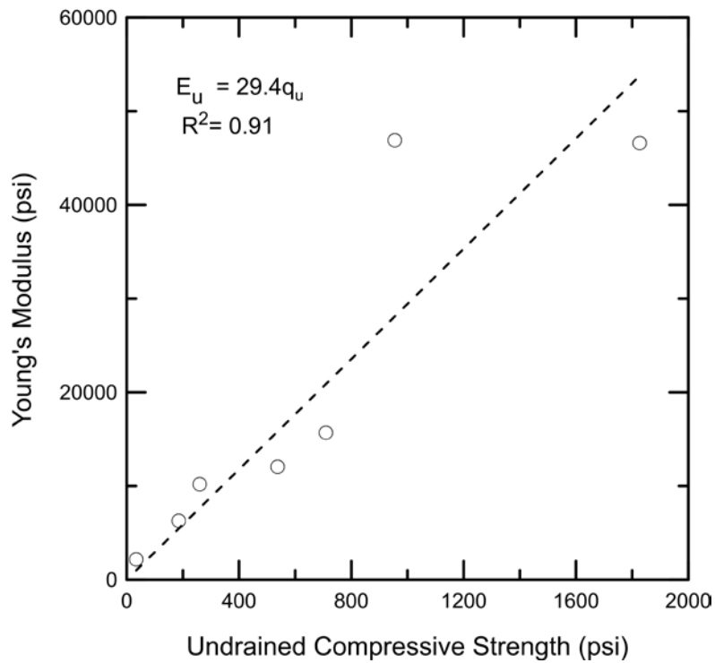
Figure J.6 Relationship between undrained compressive strength and Young's modulus.
