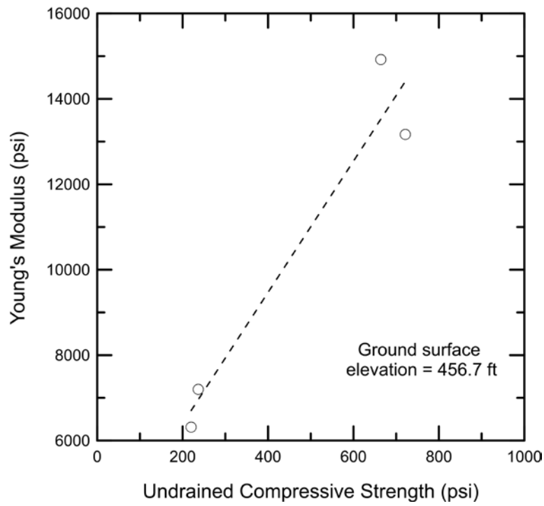
Figure E.6 Relationship between undrained compressive strength and Young's modulus.
