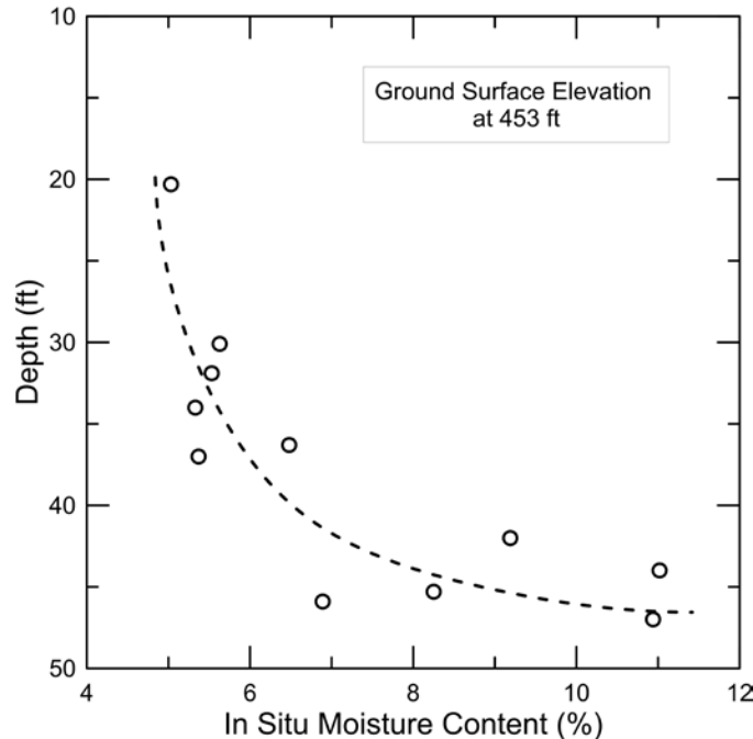
Figure I.5 In situ moisture content profile.
