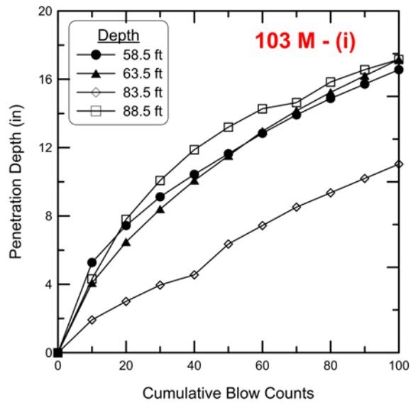
Figure C.5 Modified Standard Penetration Test results for Pier 3.
