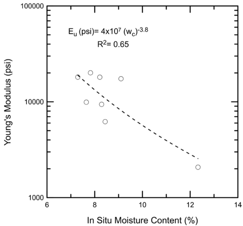
Figure N.7 Relationship between initial water content and Young's modulus.
