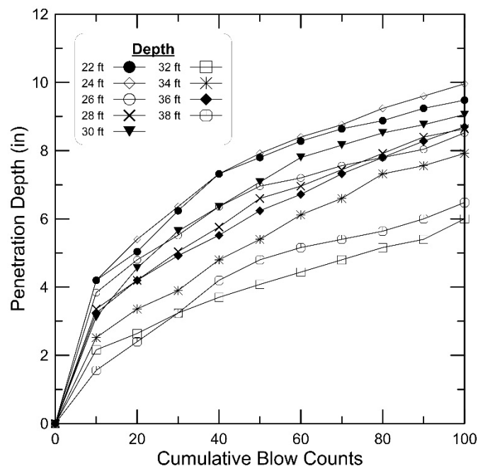
Figure N.3 Modified Standard Penetration Test results.
