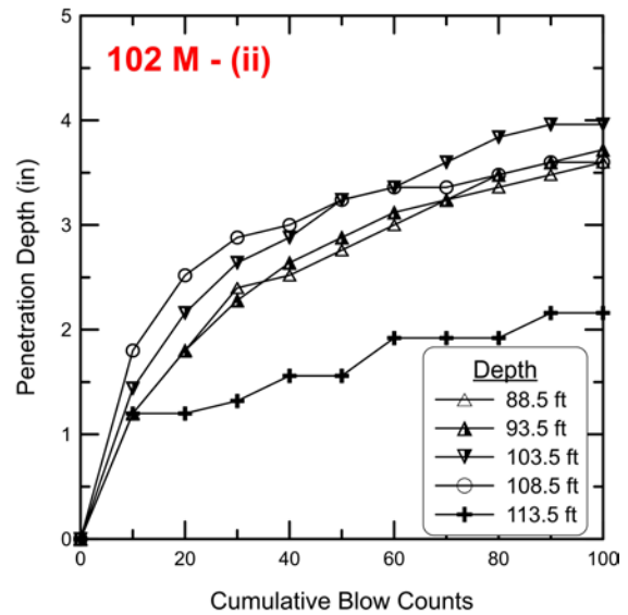
Figure C.4 Modified Standard Penetration Test results for Pier 2.
