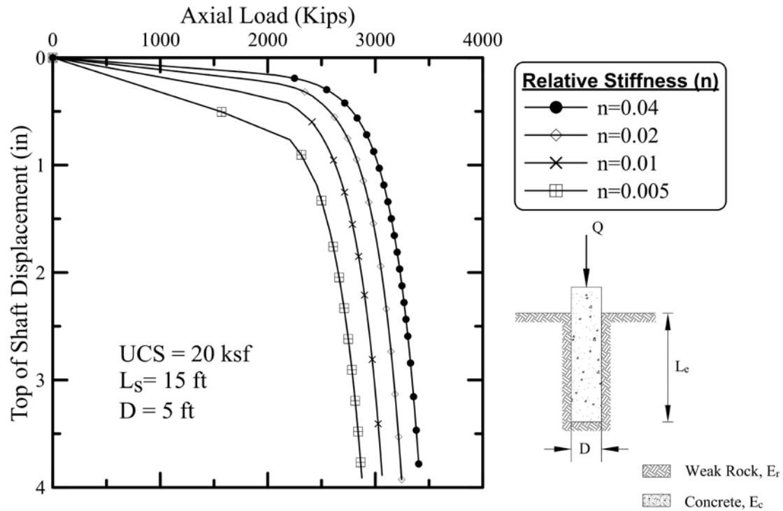
Figure 6.16. Effect of relative stiffness ( n ) on load-displacement response of weak rock drilled shaft sockets.
