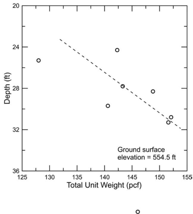
Figure N.4 Total unit weight profile.
