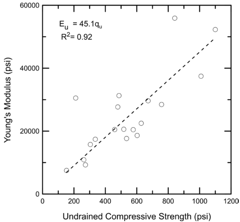
Figure K.6 Relationship between undrained compressive strength and Young's modulus.
