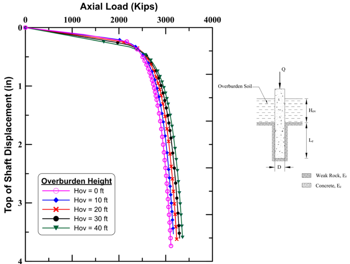
Figure 6.19. Effect of overburden height on the axial load-displacement behavior of weak rock-socketed shafts.
