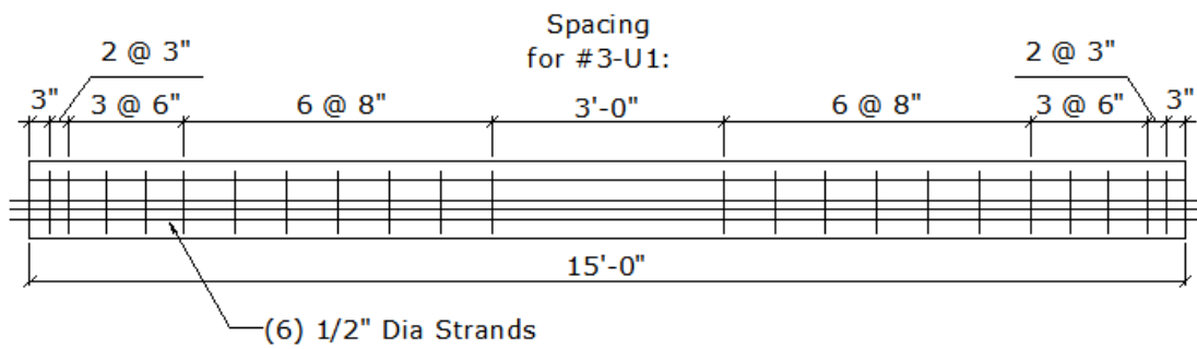
Figure 2 – Shear Stirrup Spacing for Flexural Girders
