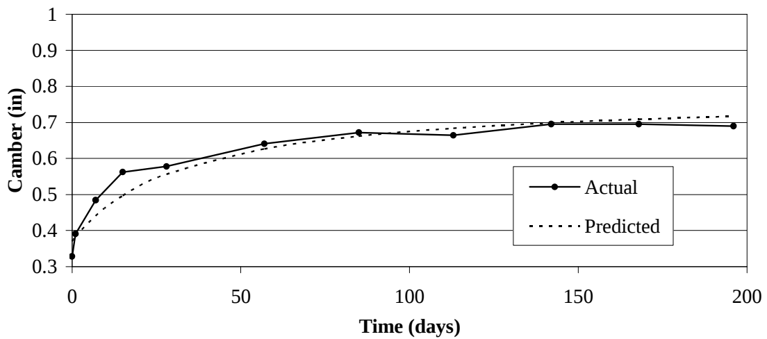
Figure 4 – Camber Development for Beam 65
