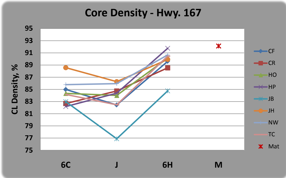
FIGURE 38 Phase 2 Vacuum Sealing Core Density Summary of Results – Hwy. 167.
