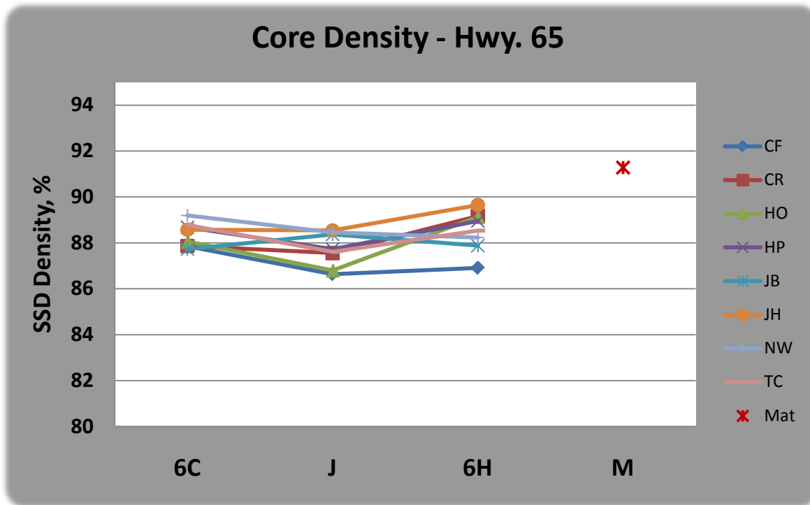
FIGURE 37 Phase 2 SSD Core Density Summary of Results – Hwy. 65.
