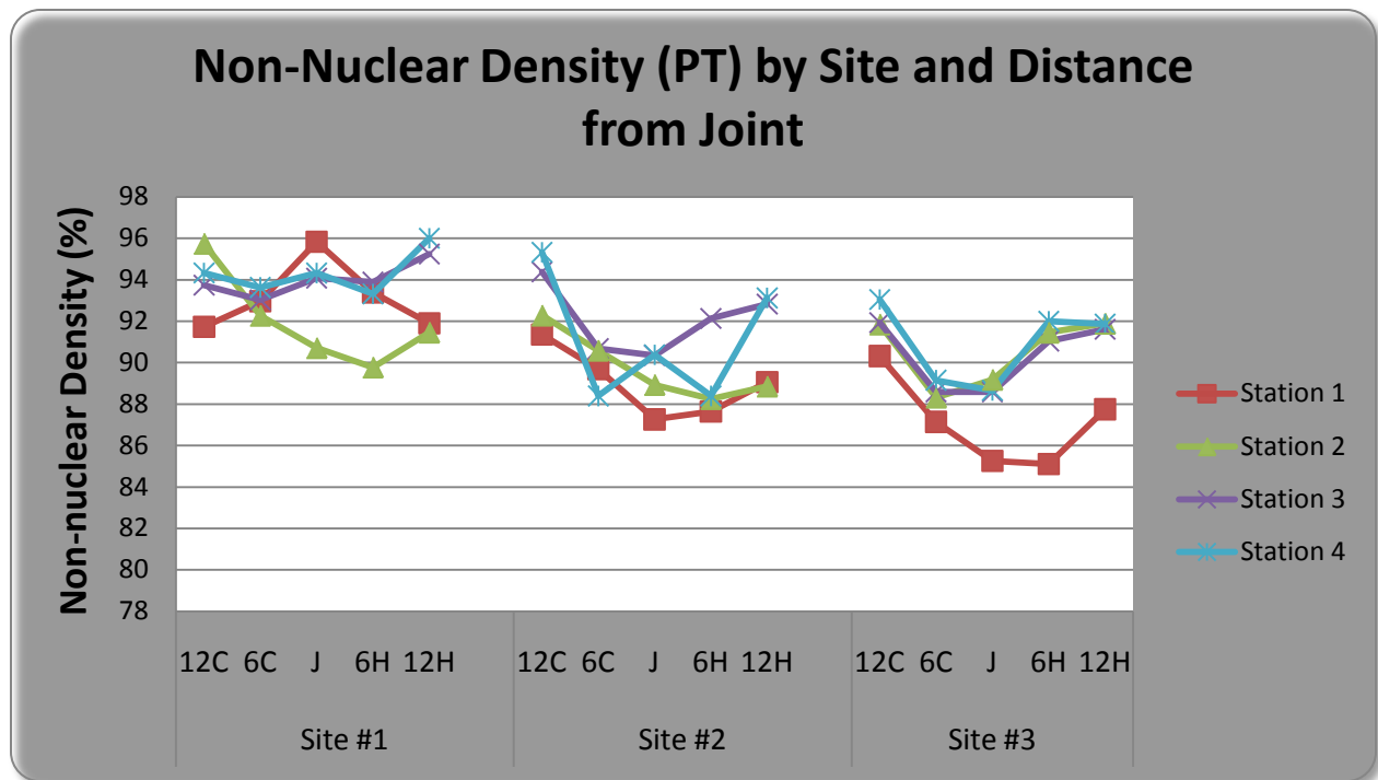
FIGURE 12 Phase 1 PaveTracker Non-Nuclear Density Comparison (%Gmm).
