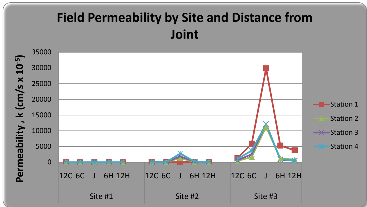
FIGURE 13 Phase 1 Field Permeability Comparison (cm/s x 10 -5 ).
