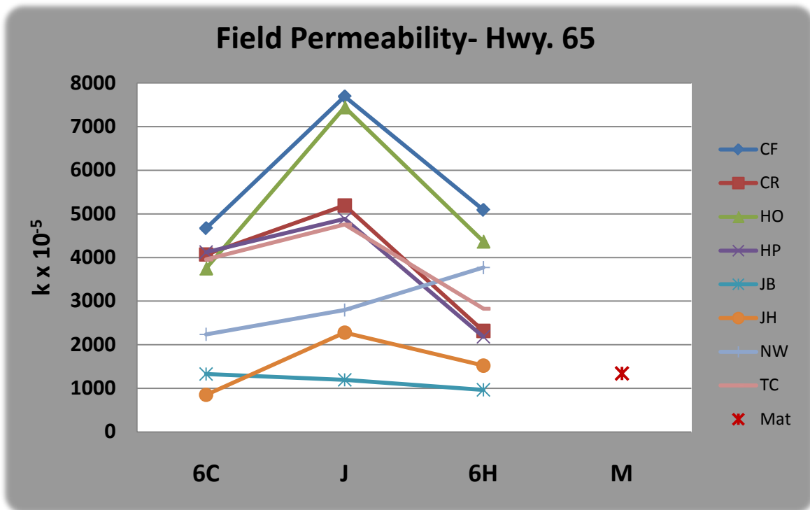
FIGURE 43 Phase 2 Permeability Summary of Results – Hwy. 65.
