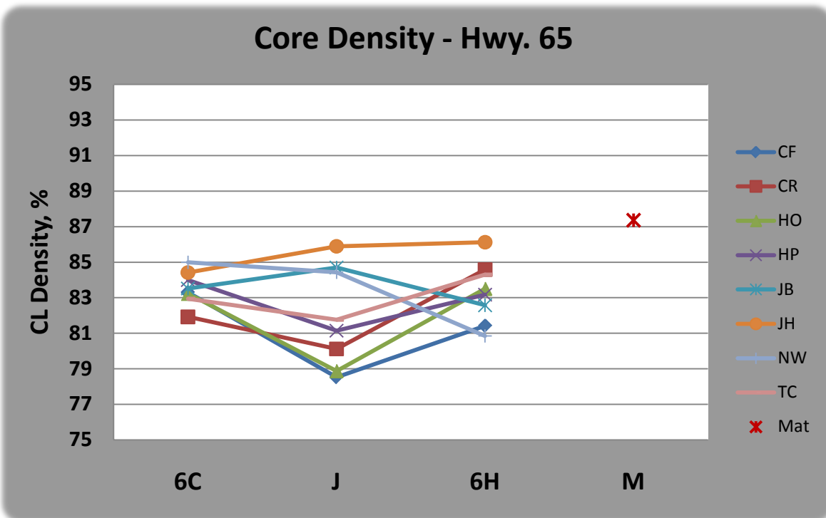
FIGURE 39 Phase 2 Vacuum Sealing Core Density Summary of Results – Hwy. 65.
