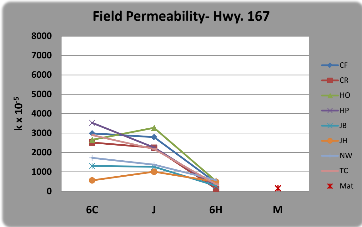
FIGURE 42 Phase 2 Permeability Summary of Results – Hwy. 167.
