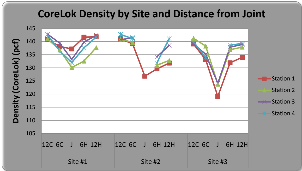
FIGURE 17 Phase 1 Vacuum Sealing Density Comparison (pcf).
