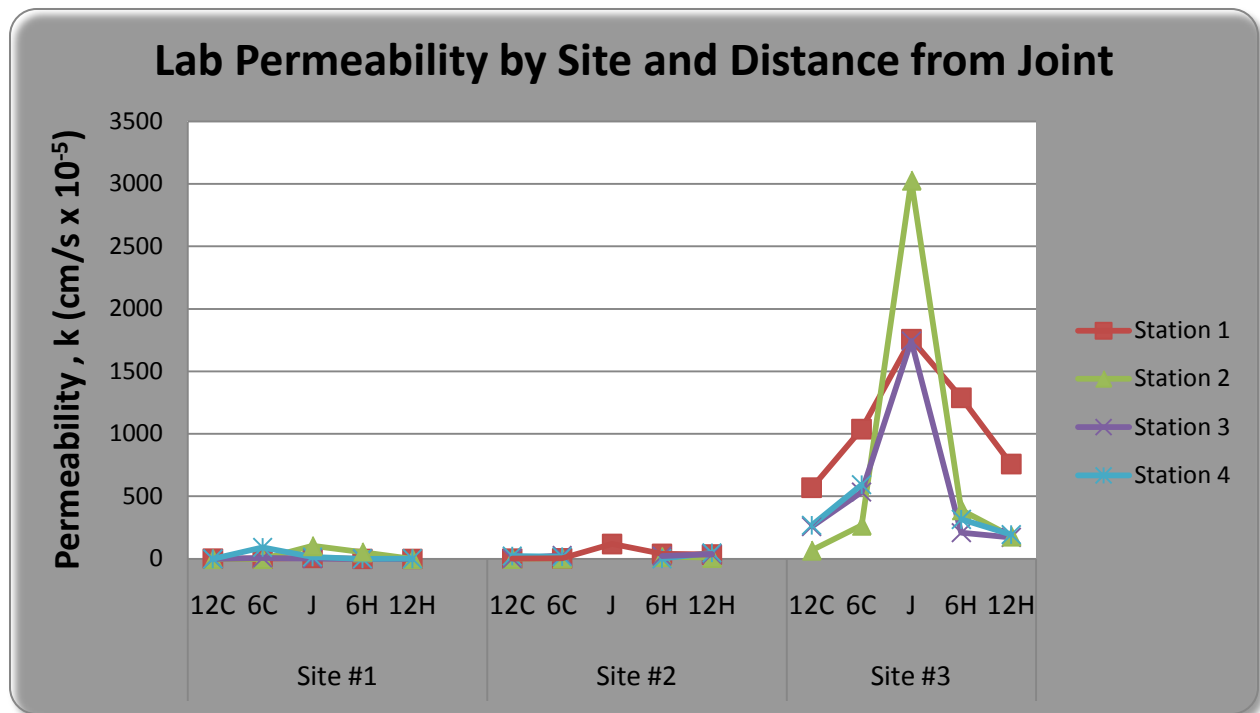
FIGURE 20 Phase 1 Laboratory Permeability Comparison (cm/s \times 10^{-5} ).
