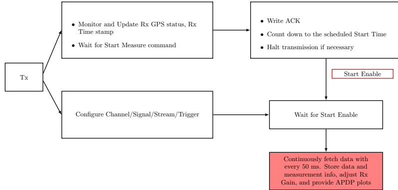
Figure 2.2: Functionality diagram of the Rx USRP
