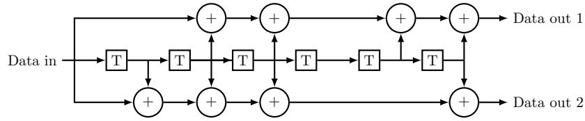
Figure 5.3: Data encoder
