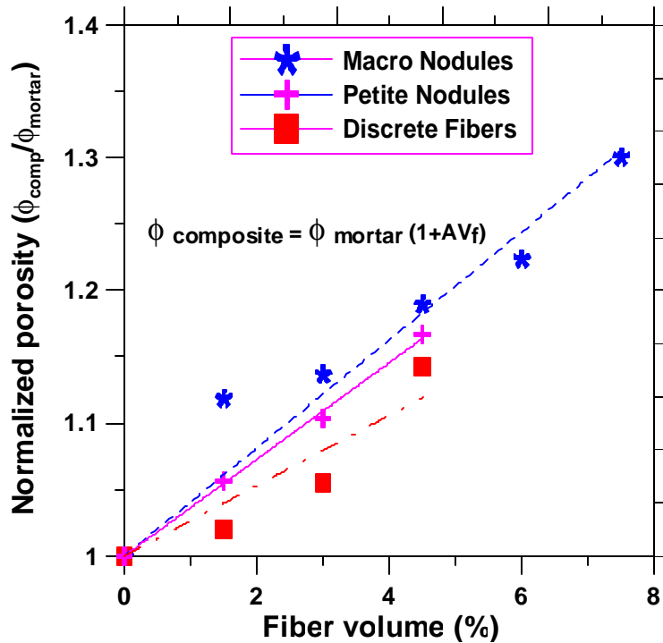
Figure 5.1 Influence of fiber volume and morphology on composite porosity
