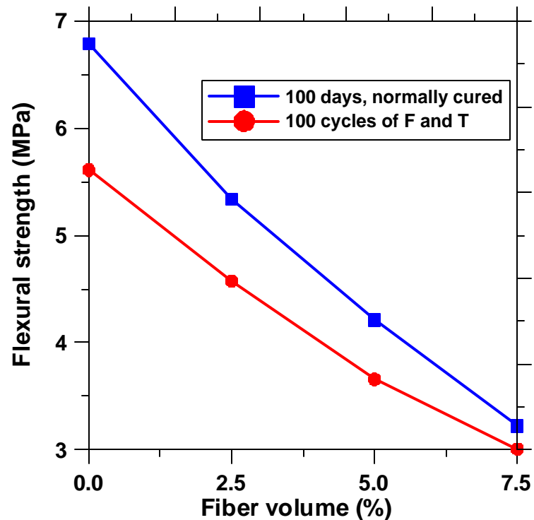
Figure 7.5 Comparison between flexural strengths of normally cured specimens and those subjected to 100 cycles of freezing and thawing
