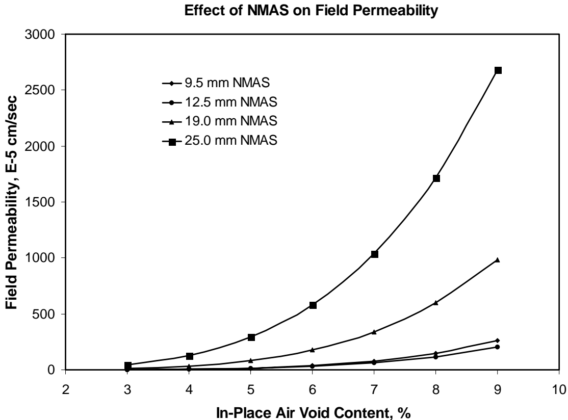
Figure 9. Effect of NMAS on Permeability
