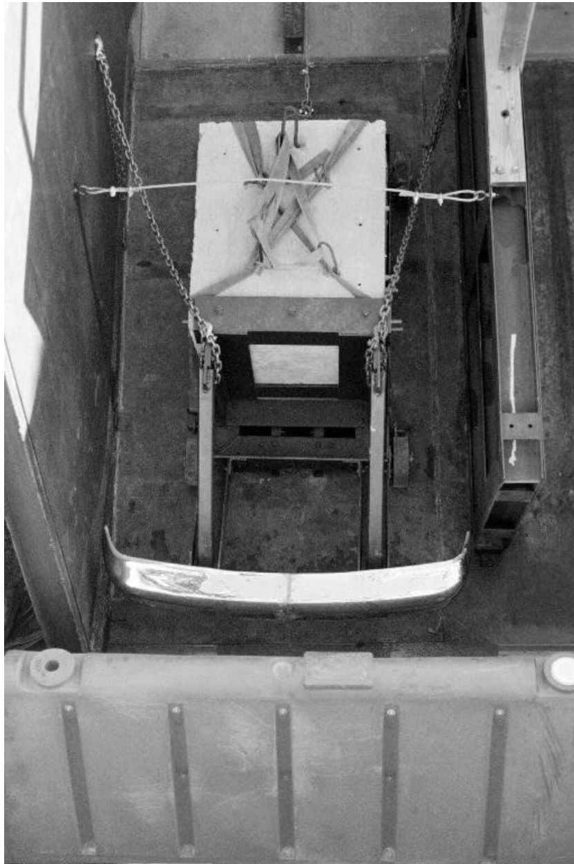
Figure 4.3: Surrogate test vehicle loaded with the concrete block and chained to the flume to permit safe barrier placement. Also visible are the safety cable, tiedown straps, and the end of the guide rail.
