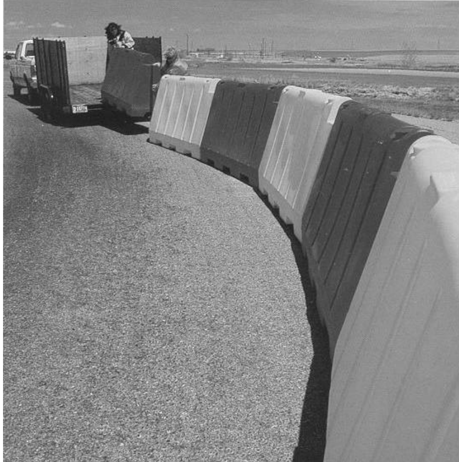
Figure 3.11: Assembly of an interconnected line of barrier specimens in the field.
