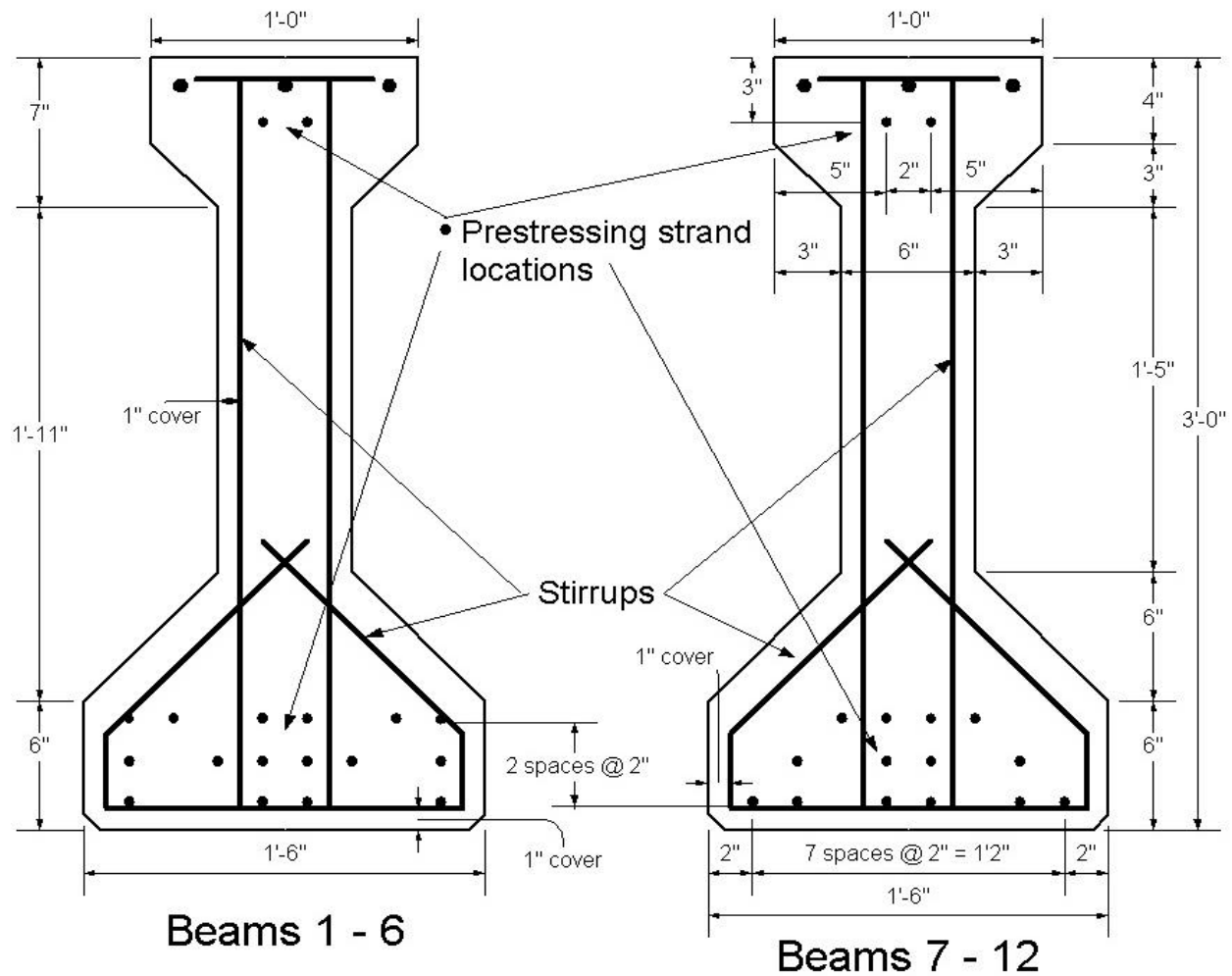
Figure 2. Beam cross sections detailing stirrup and pre-stressing strand locations.
