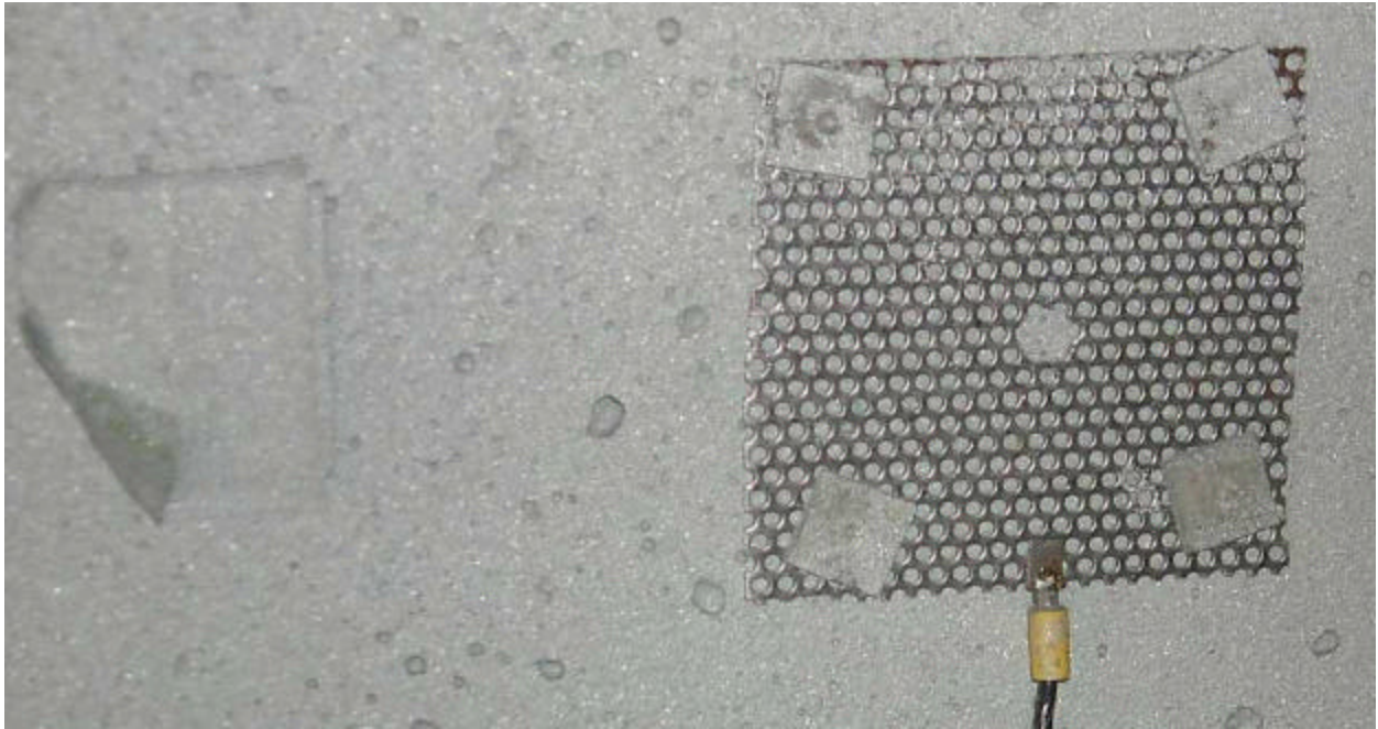
Photo 5. Expanded steel plate before second metallizing pass. Note loose tape on left.
