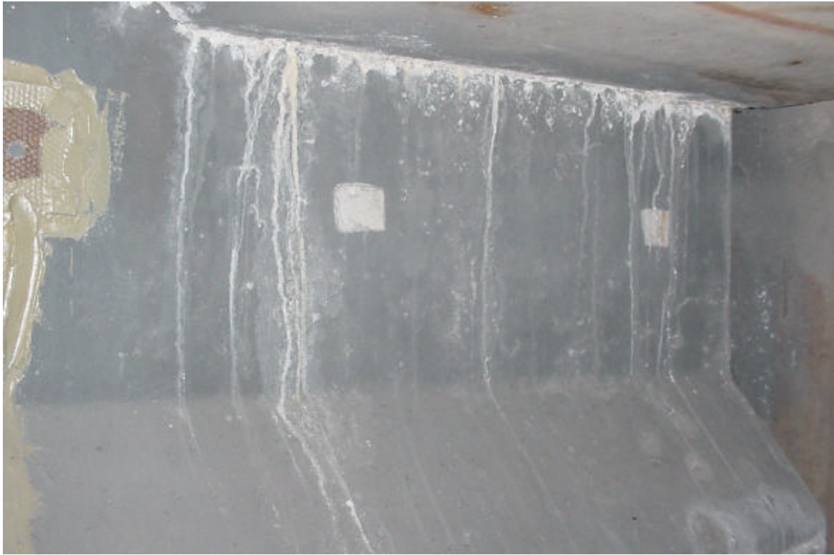
Photo 9. Beam 10, east side. Corrosion products forming from leaks in deck or at joint.
